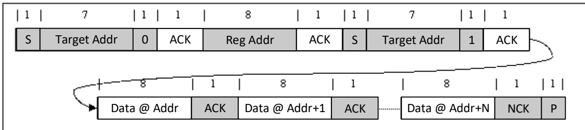
Figure 8-16. Multi-Read
