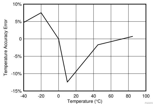
Figure 8-4. Internal Temperature Accuracy Error
