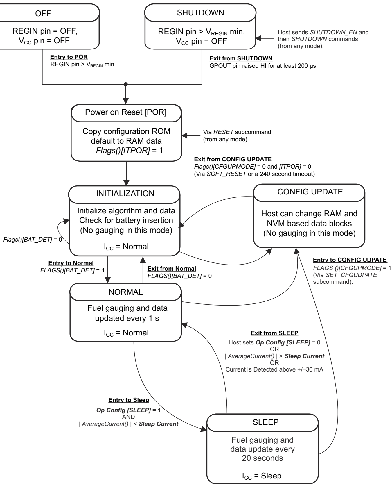
Figure 7-5. Power Mode Diagram
