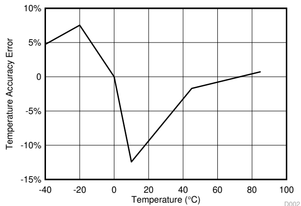
Figure 6-4. Internal Temperature Accuracy Error
