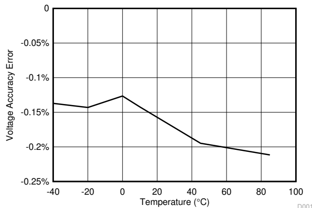
Figure 8-3. Voltage Accuracy Error
