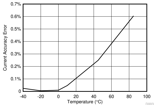
Figure 8-5. Current Accuracy Error
