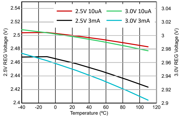
Figure 6-7. Regulator Output vs. Temperature (2.5V and 3V Settings)
