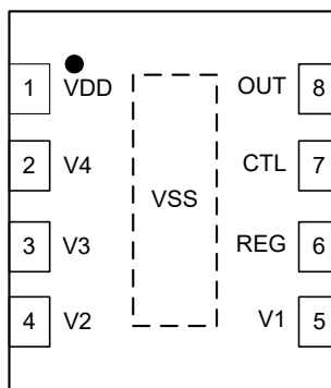
Figure 5-1. 2-Series to 4-Series BQ2969T (Top View)
