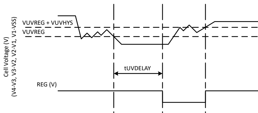
Figure 7-3. REG Output Timing
