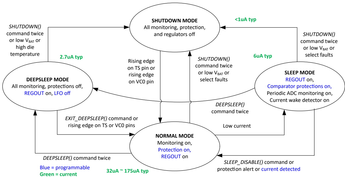
Figure 7-5. BQ76907 Operational Power Modes
