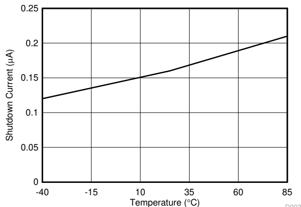
Figure 7-2. Shutdown Current
