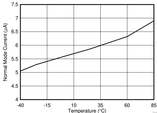
Figure 7-1. NORMAL Mode Current
