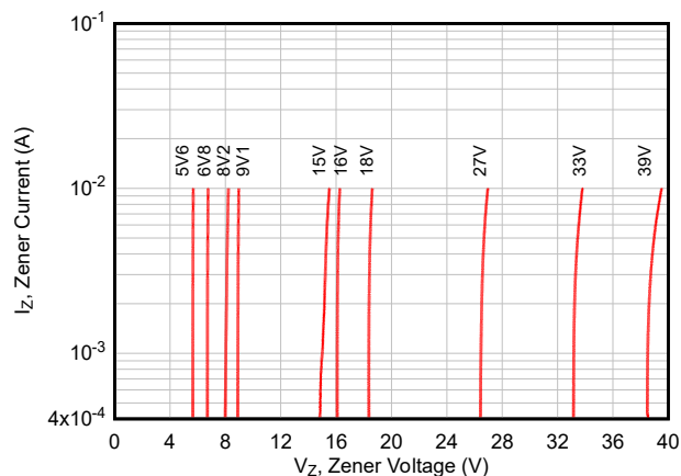
Figure 6-1. Zener Current vs Zener Voltage
