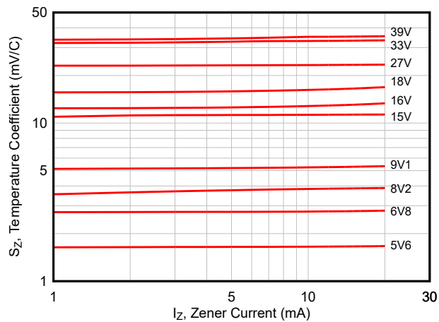
Figure 6-2. Temperature Coefficient
