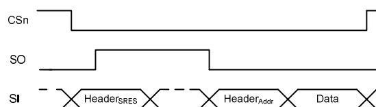
Figure 12: SRES Command Stroke
