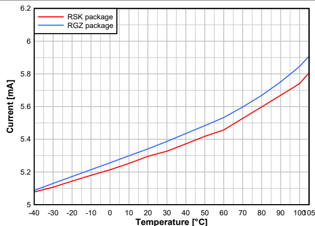
Figure 8-6. RX Current vs. Temperature (50 kbps, 868.3 MHz, VDD5 = 3.6 V)
