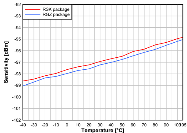
Figure 8-19. Sensitivity vs. Temperature (BLE 1 Mbps, 2.44 GHz)
