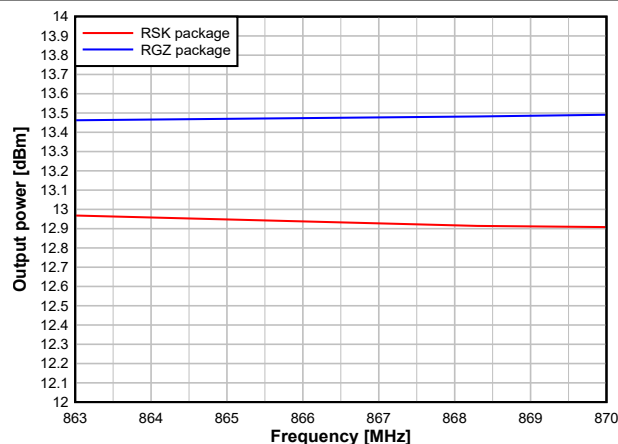
Figure 8-31. Output Power vs. Frequency (50 kbps, 868 MHz, +14 dBm)
