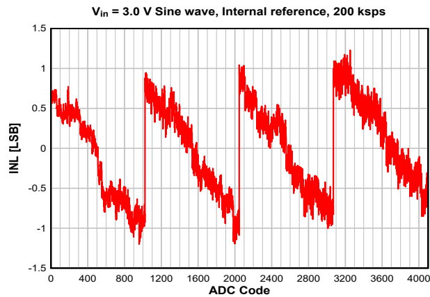
Figure 8-37. INL vs. ADC Code
