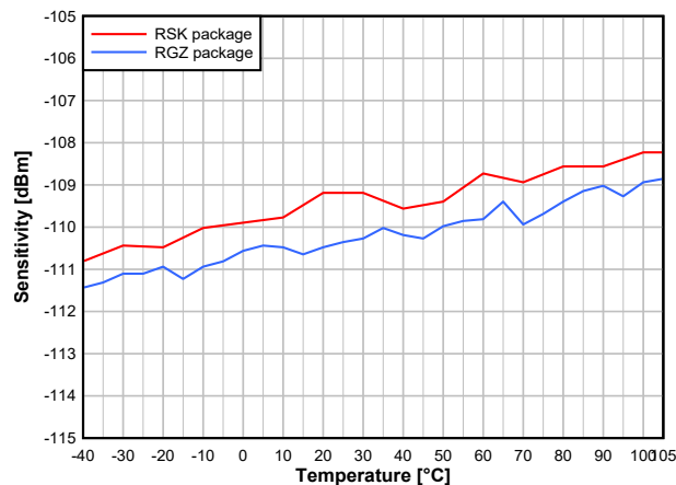
Figure 8-18. Sensitivity vs. Temperature (50 kbps, 868.3 MHz)
