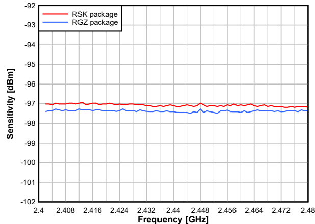
Figure 8-16. Sensitivity vs. Frequency (BLE 1 Mbps, 2.44 GHz)
