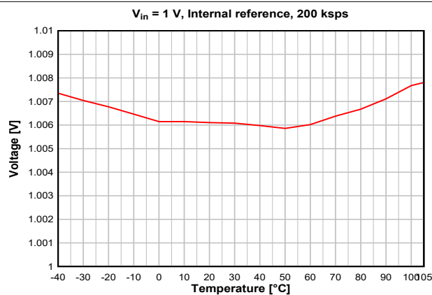
Figure 8-39. ADC Accuracy vs. Temperature
