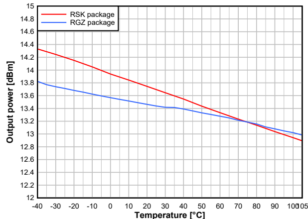
Figure 8-25. Output Power vs. Temperature (50 kbps, 868.3 MHz, +14 dBm)
