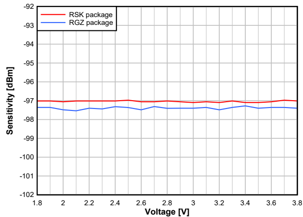
Figure 8-22. Sensitivity vs. Supply Voltage (VDD5) (BLE 1 Mbps, 2.44 GHz)
