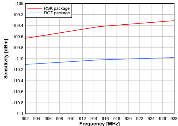
Figure 8-15. Sensitivity vs. Frequency (50 kbps, 915 MHz)
