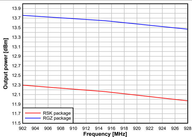
Figure 8-32. Output Power vs. Frequency (50 kbps, 915 MHz, +14 dBm)
