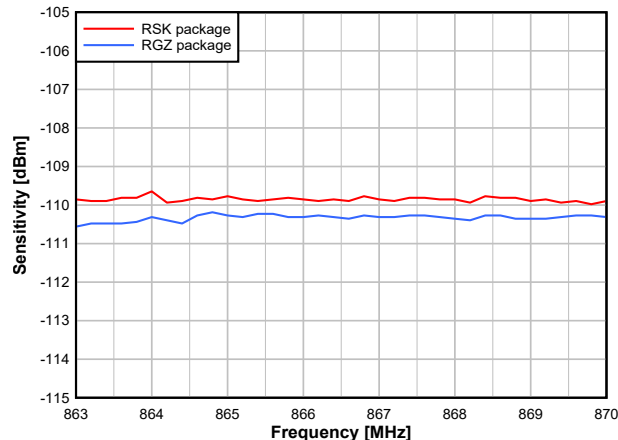
Figure 8-14. Sensitivity vs. Frequency (50 kbps, 868 MHz)
