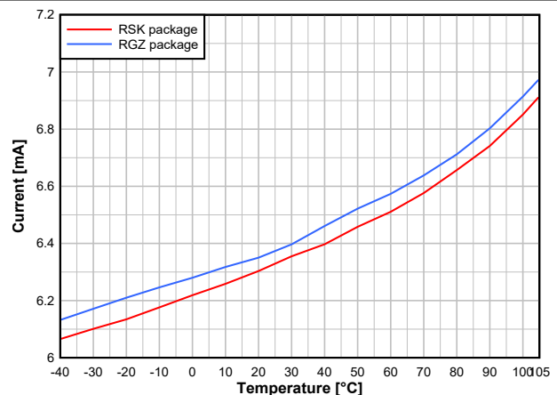
Figure 8-7. RX Current vs. Temperature (BLE 1 Mbps, 2.44 GHz)
