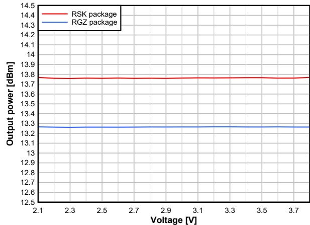
Figure 8-28. Output Power vs. Supply Voltage (VDD5) (50 kbps, 868.3 MHz, +14 dBm)
