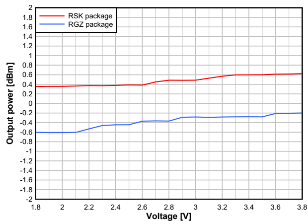
Figure 7-29. Output Power vs. Supply Voltage (VDD5) (BLE 1Mbps, 2.44GHz, 0dBm)
