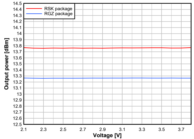
Figure 7-28. Output Power vs. Supply Voltage (VDD5) (50kbps, 868.3MHz, +14dBm)
