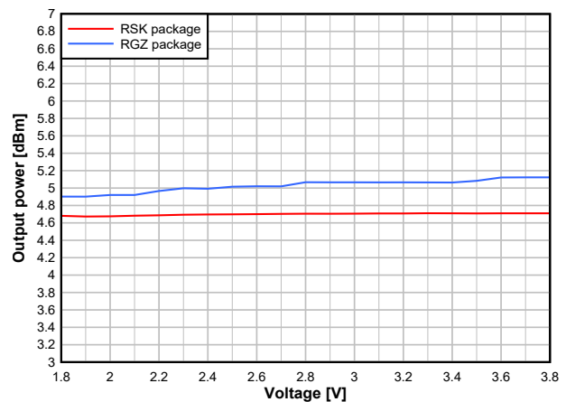
Figure 7-30. Output Power vs. Supply Voltage (VDD5) (BLE 1Mbps, 2.44GHz, +5dBm)
