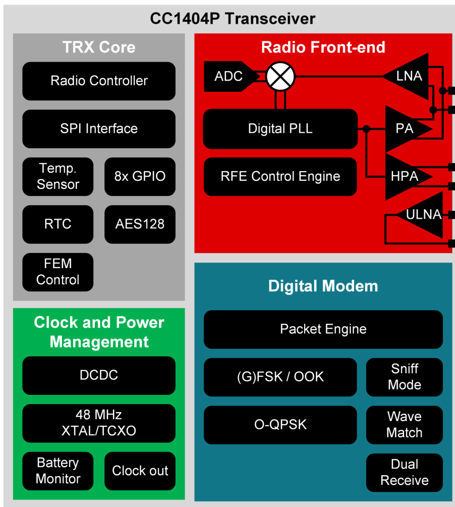
CC1404P Block Diagram
