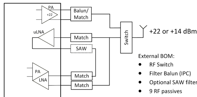
Figure 8-1. Full Entitlement reference design block diagram
