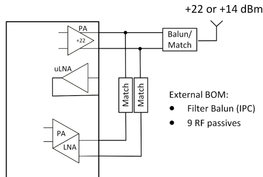
Figure 8-2. Switchless dual-PA reference design
