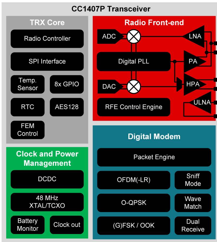
CC1407P Block Diagram
