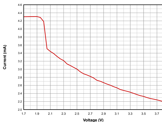
Figure 7-6. Active Mode (MCU) Current vs. Supply Voltage ( V_{DD5} ) (Running CoreMark)
