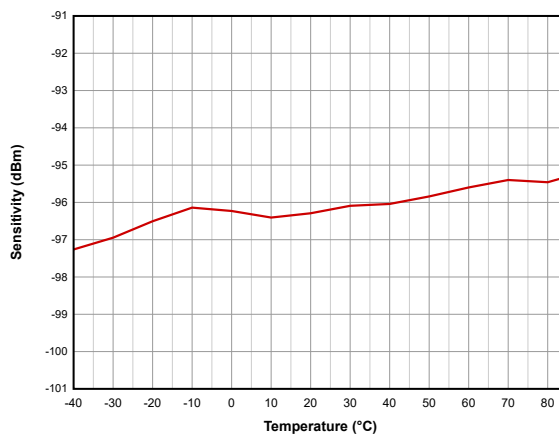
Figure 7-15. Sensitivity vs. Temperature (BLE 1Mbps, 2.44GHz)
