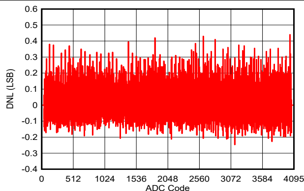
Figure 7-29. DNL vs. ADC Code ( V_{in} = 3V Sine Wave, Internal Reference, 200ksps)
