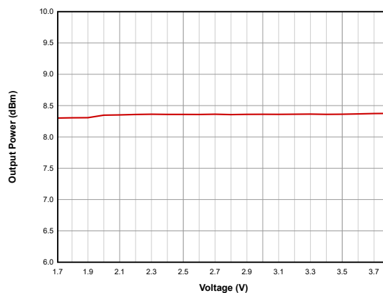
Figure 7-21. Output Power vs. Supply Voltage (VDD5) (BLE 1Mbps, 2.44GHz, +8dBm)
