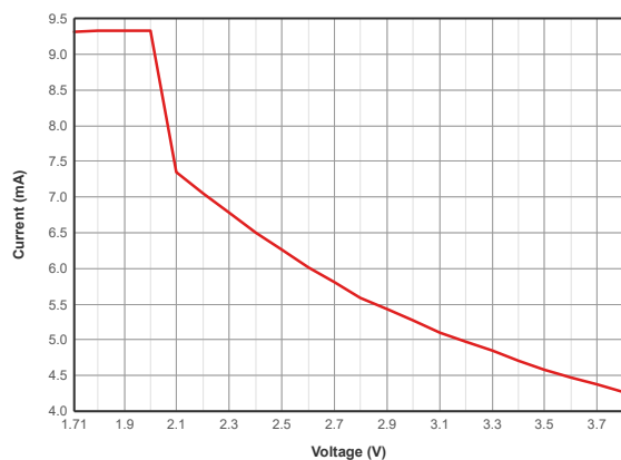
Figure 7-12. TX Current vs. Supply Voltage, VDD (BLE 1Mbps, 2.44GHz, 0dBm)
