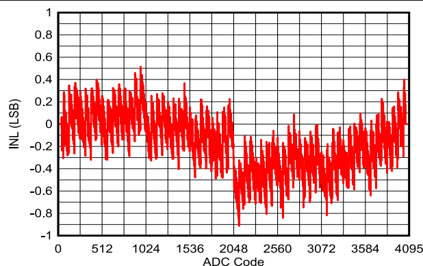
Figure 7-28. INL vs. ADC Code ( V_{in} = 3V Sine Wave, Internal Reference, 200ksps)
