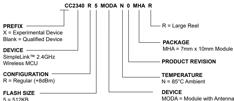
Figure 11-1. Device Nomenclature
