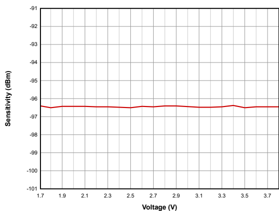
Figure 7-17. Sensitivity vs. Supply Voltage (VDDS) (BLE 1Mbps, 2.44GHz, DCDC Off)
