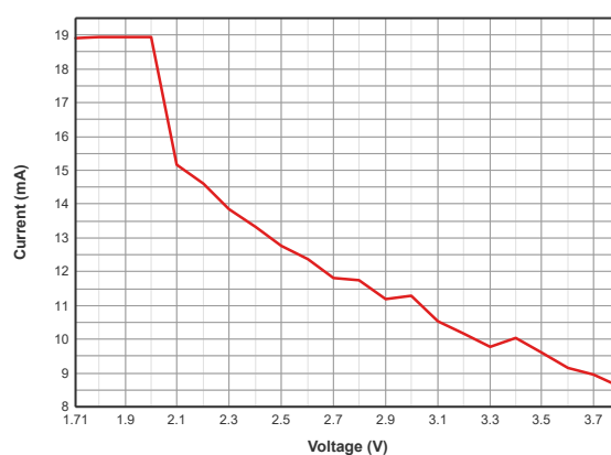
Figure 7-13. TX Current vs. Supply Voltage, VDD (BLE 1Mbps, 2.44GHz, +8dBm)
