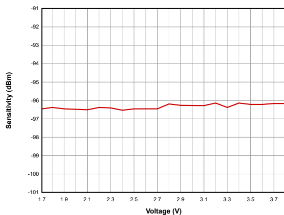
Figure 7-16. Sensitivity vs. Supply Voltage (VDDS) (BLE 1Mbps, 2.44GHz)
