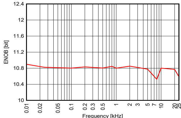
Figure 7-24. ENOB vs. Input Frequency (Internal Reference)
