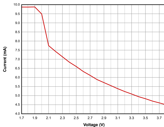
Figure 7-9. RX Current vs. Supply Voltage (VDD) (BLE 1Mbps, 2.44GHz)
