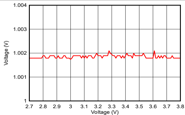
Figure 7-31. ADC Accuracy vs. Supply Voltage ( V_{in}=1V , Internal Reference, 200ksps)
