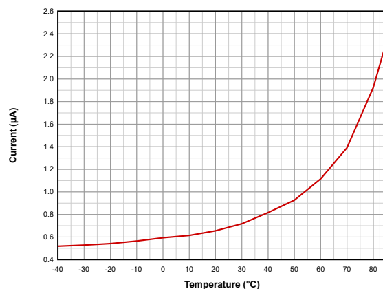
Figure 7-7. Standby Mode (MCU) Current vs. Temperature ( RAM and partial register retention, RTC)
