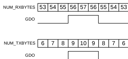
Figure 19: FIFO_THR=13 vs. Number of Bytes in FIFO ( GD0x_CFG=0x00 in RX and GD0x_CFG=0x02 in TX)
