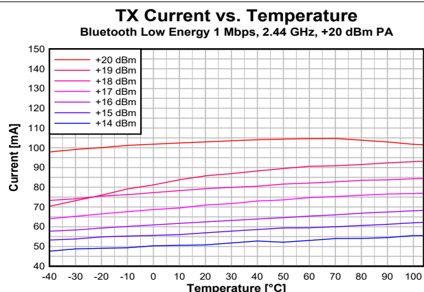
Figure 7-9. TX Current vs. Temperature (Bluetooth Low Energy 1 Mbps, 2.44 GHz, VDD5 = 3.3 V)
