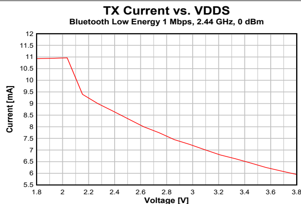
Figure 7-11. TX Current vs. Supply Voltage (VDD5) (Bluetooth Low Energy 1 Mbps, 2.44 GHz)
