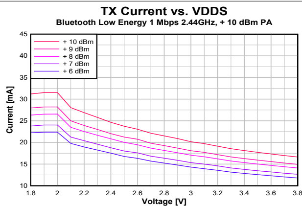
Figure 7-13. TX Current vs. Supply Voltage (VDD5) (250 kbps, 2.44 GHz, +10 dBm PA)
