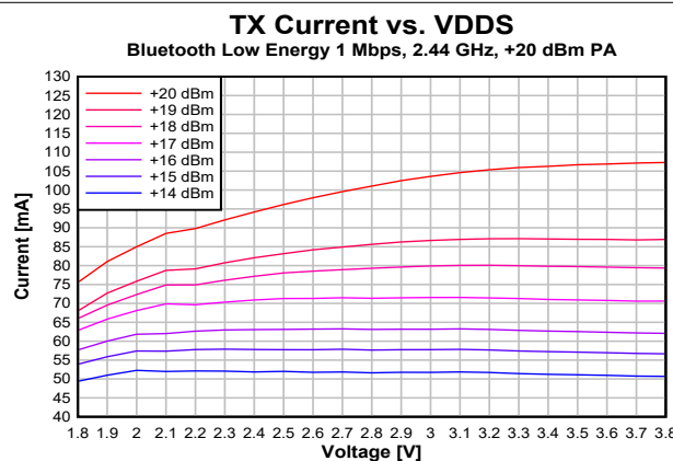
Figure 7-12. TX Current vs. Supply Voltage (VDD5) (Bluetooth Low Energy 1 Mbps, 2.44 GHz, +20 dBm PA)
