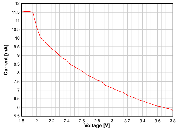
Figure 8-10. TX Current vs. Supply Voltage (VDD) (WBMS, 2.44 GHz, 0 dBm)
