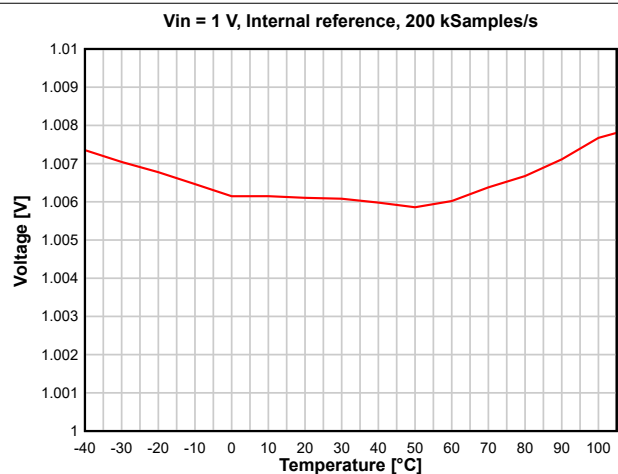
Figure 8-25. ADC Accuracy versus Temperature
