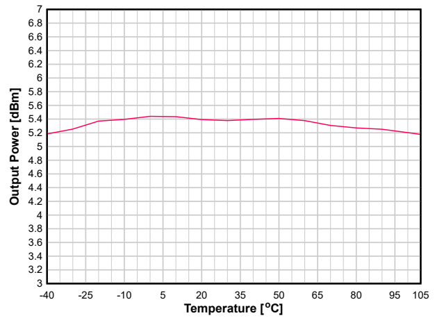
Figure 8-16. Output Power vs. Temperature (WBMS, 2.44 GHz, +5dBm)
