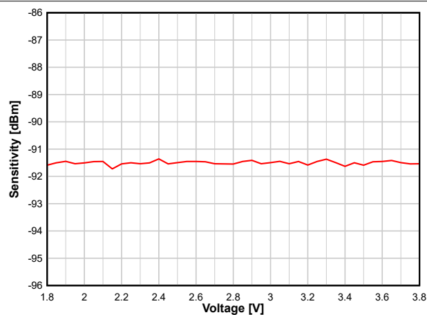
Figure 8-13. Sensitivity versus Supply Voltage (VDDS) (WBMS, 2.44 GHz)
