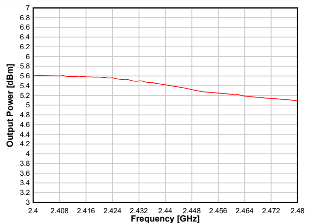
Figure 8-20. Output Power vs. Frequency (WBMS, +5dBm)
