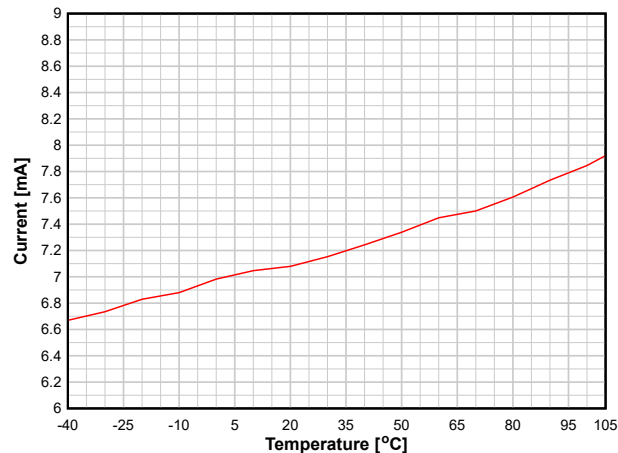
Figure 8-9. TX Current vs. Temperature (WBMS, 2.44 GHz, 0 dBm)
