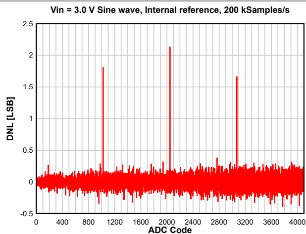
Figure 8-24. DNL versus ADC Code
