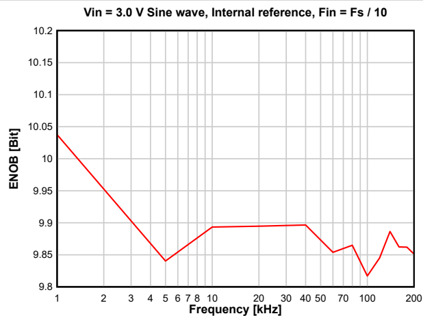
Figure 8-22. ENOB versus Sampling Frequency
