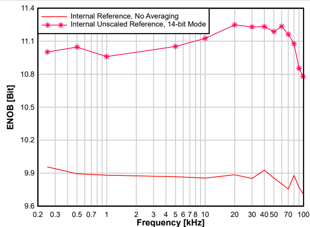
Figure 8-21. ENOB versus Input Frequency
