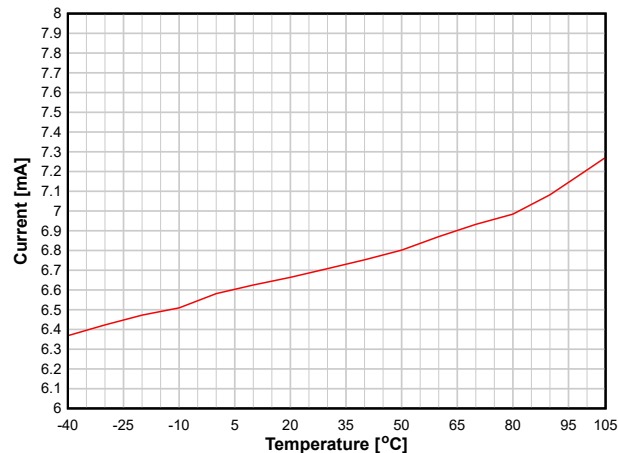
Figure 8-7. RX Current versus Temperature (WBMS, 2.44 GHz)
