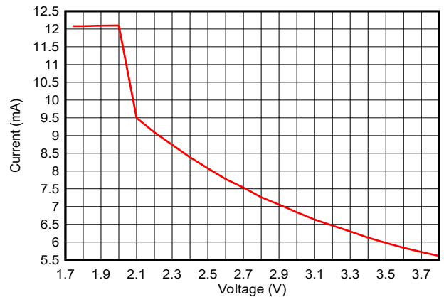
Figure 7-9. RX Current vs Supply Voltage ( V_{\text{DDS}} ) (LE 1M PHY, 2.44GHz)
