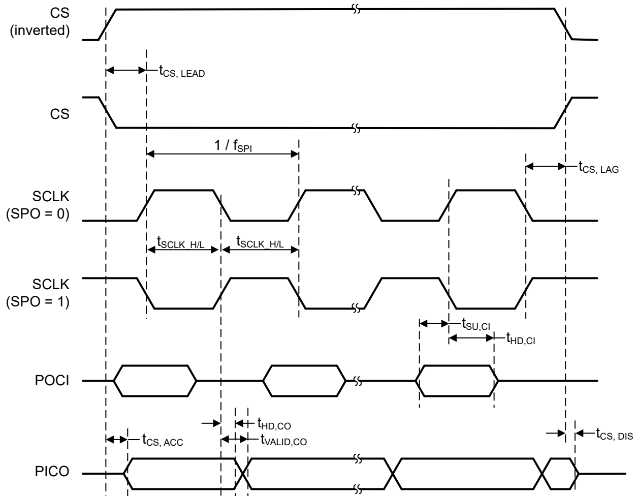
Figure 7-1. SPI Timing Diagram—Controller Mode, SPH = 0
