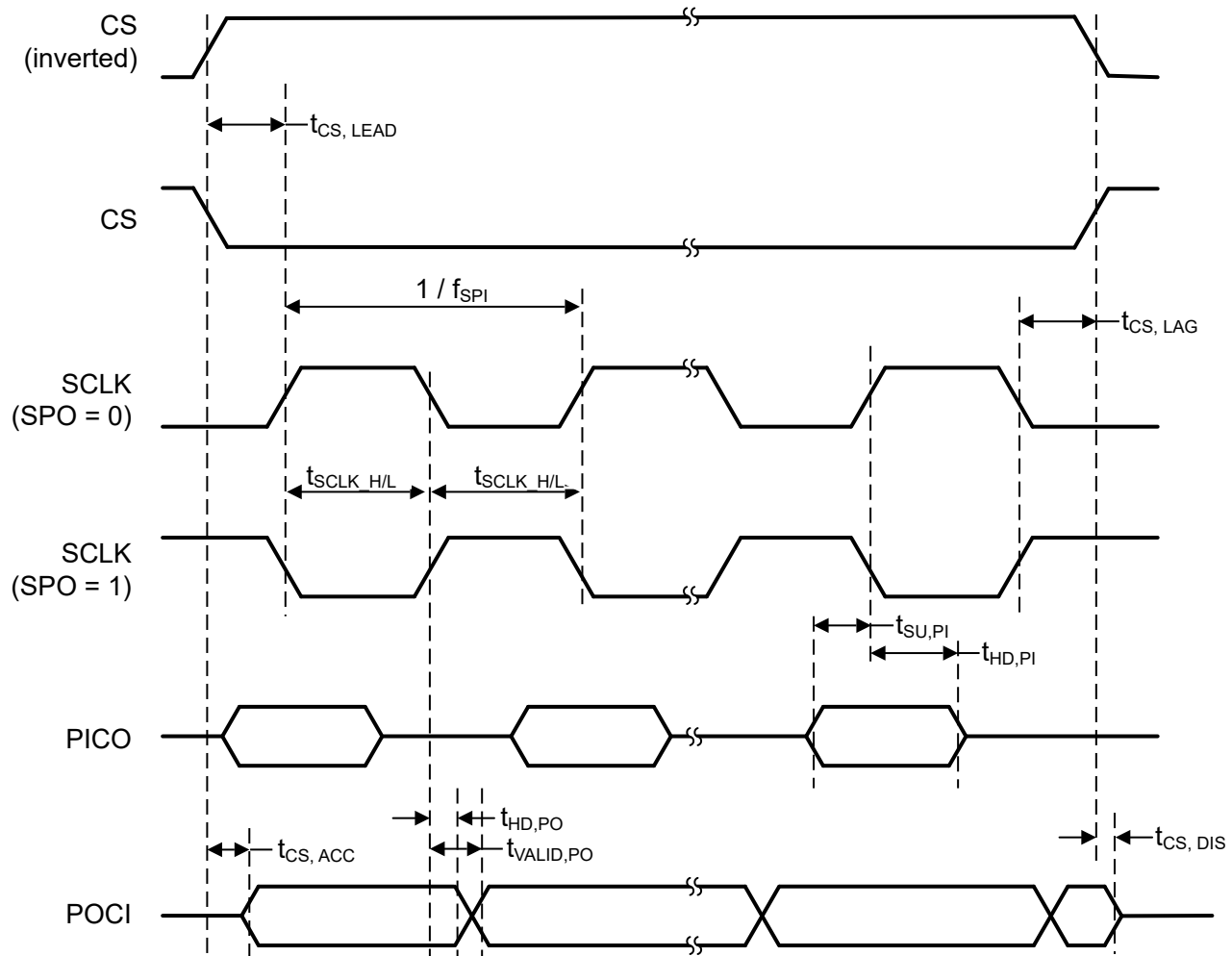
Figure 7-3. SPI Timing Diagram—Peripheral Mode, SPH = 0
