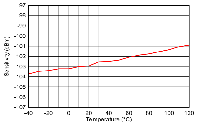
Figure 7-17. Sensitivity vs Temperature (IEEE 802.15.4 PHY)
