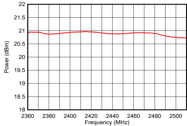
Figure 7-27. Output Power vs Frequency (LE 1M PHY, +20dBm)
