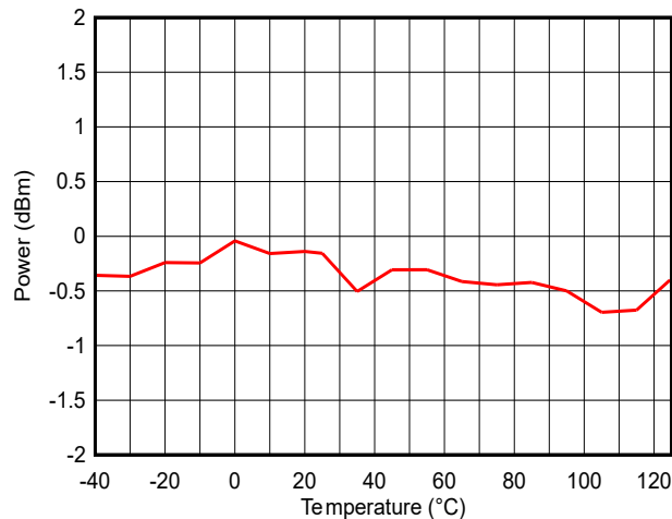
Figure 7-22. Output Power vs Temperature (LE 1M PHY, 2.44GHz, 0dBm)
