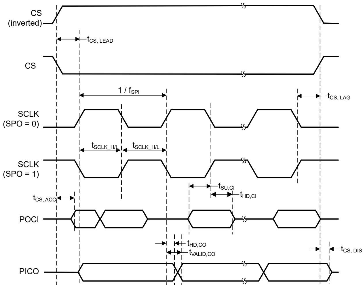
Figure 7-2. SPI Timing Diagram—Controller Mode, SPH = 1
