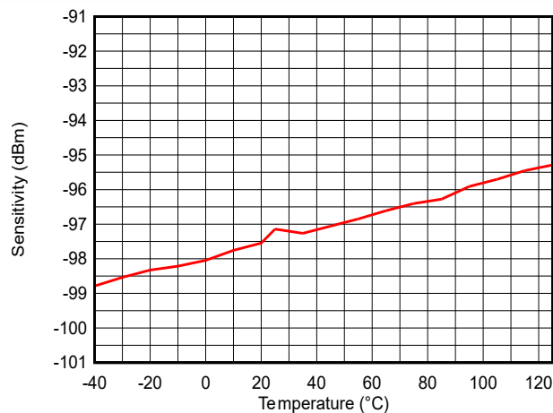
Figure 7-16. Sensitivity vs Temperature (LE 1M PHY, 2.44GHz)
