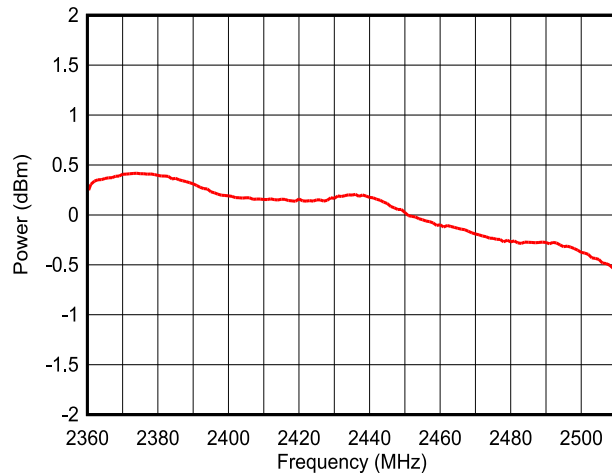
Figure 7-26. Output Power vs Frequency (LE 1M PHY, 0dBm)
