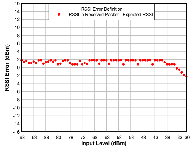
Figure 7-21. RSSI Error vs Input Level (dBm)
