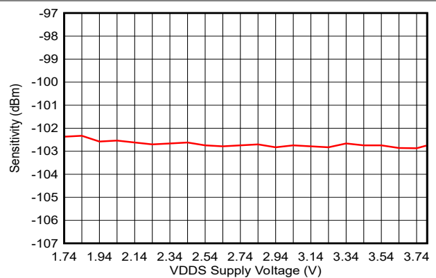
Figure 7-19. Sensitivity vs VDD (IEEE 802.15.4 PHY)
