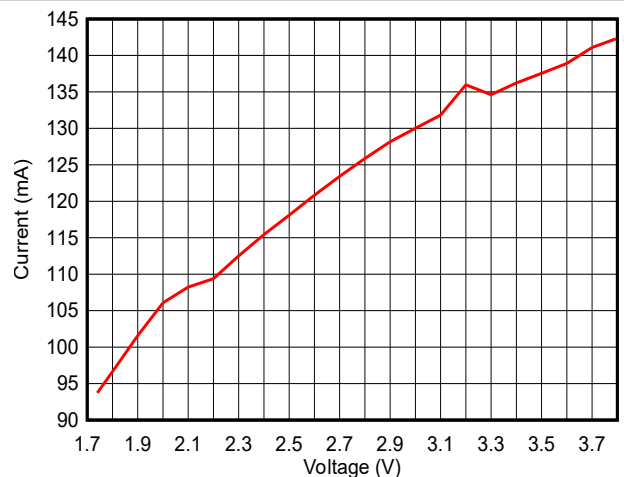
Figure 7-13. TX Current vs Supply Voltage (VDDS) (LE 1M PHY, 2.44GHz, +20dBm)
