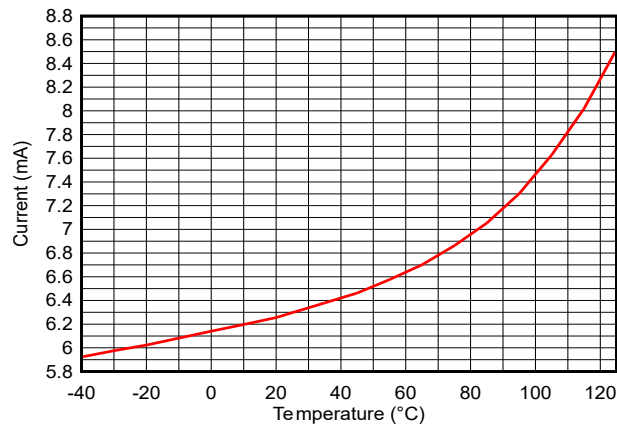
Figure 7-8. RX Current vs Temperature (LE 1M PHY, 2.44GHz), V_{\text{DDS}} = 3.3\text{V}
