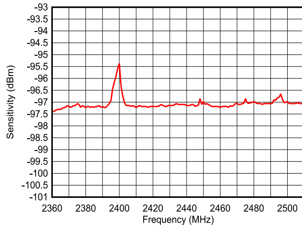
Figure 7-14. Sensitivity vs Frequency (LE 1M PHY)
