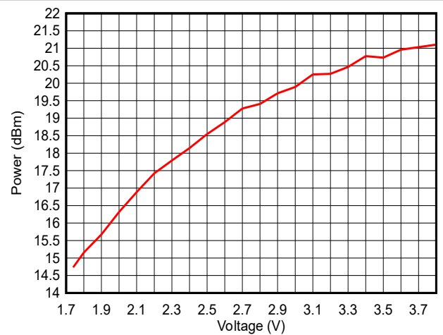
Figure 7-25. Output Power vs Supply Voltage (VDD5) (LE 1M PHY, 2.44GHz, +20dBm)
