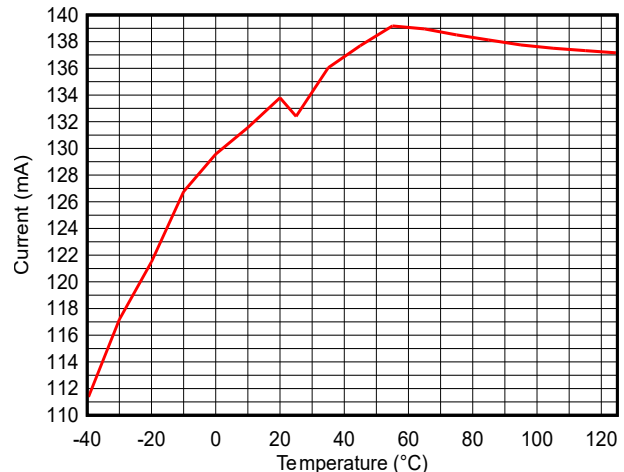
Figure 7-11. TX Current vs Temperature (LE 1M PHY, 2.44GHz, +20dBm), VDDS = 3.3V
