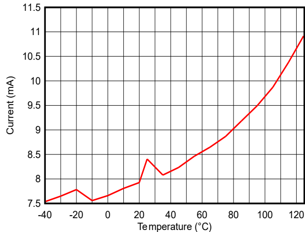
Figure 7-10. TX Current vs Temperature (LE 1M PHY, 2.44GHz, 0dBm), VDDS = 3.3V
