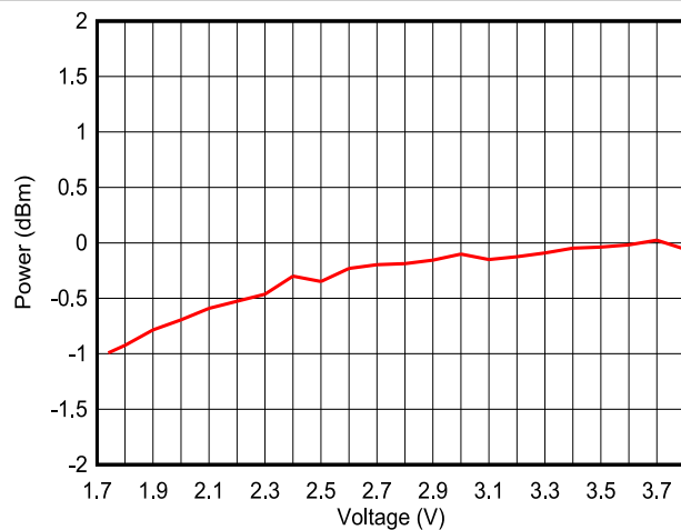
Figure 7-24. Output Power vs Supply Voltage (VDD5) (LE 1M PHY, 2.44GHz, 0dBm)
