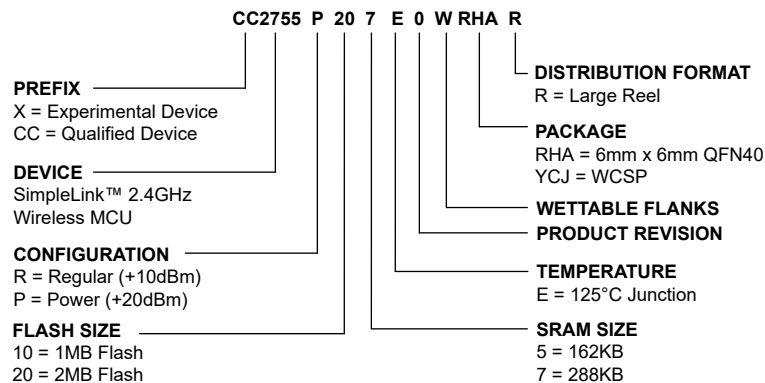
Figure 10-1. Device Nomenclature
