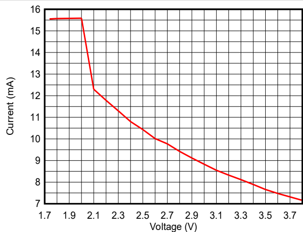
Figure 7-12. TX Current vs Supply Voltage (VDDS) (LE 1M PHY, 2.44GHz, 0dBm)
