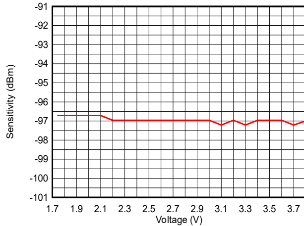
Figure 7-20. Sensitivity vs Supply Voltage (VDD5) (LE 1M PHY, 2.44GHz, DC/DC Disabled)
