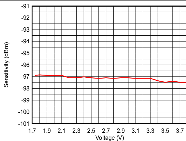
Figure 7-18. Sensitivity vs Supply Voltage (VDD) (LE 1M PHY, 2.44GHz)
