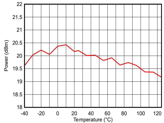
Figure 7-23. Output Power vs Temperature (LE 1M PHY, 2.44GHz, +20dBm)
