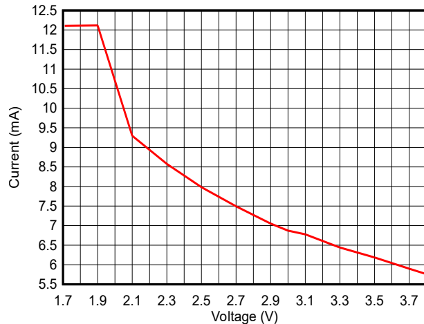
Figure 7-6. Active Mode (MCU) Current vs Supply Voltage ( V_{\text{DDS}} ) (Running CoreMark)
