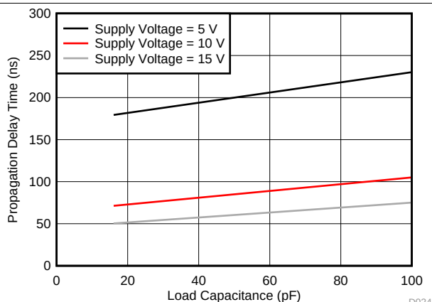
SET to \bar{Q} or RESET to Q Figure 6. Typical Propagation Delay Time vs Load Capacitance
