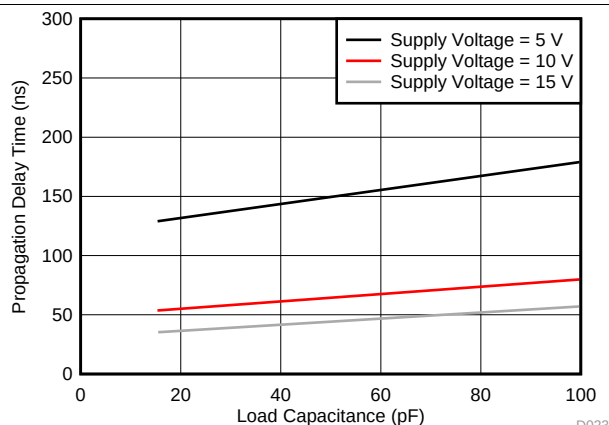
CLOCK or SET to Q, CLOCK or RESET to \bar{Q} Figure 5. Typical Propagation Delay Time vs Load Capacitance
