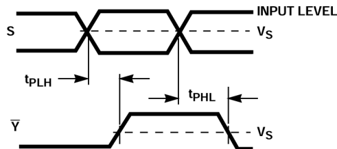
Figure 5-3. Select to Output Propagation Delays (CD74ACT258)
