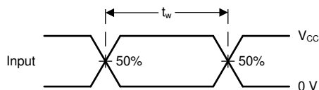
Figure 5-1. Voltage Waveforms, Standard CMOS Inputs Pulse Duration
