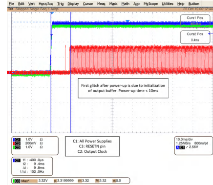
Figure 5-6. All Power Supply = 3.3 V, VDD Ramp Time = 1 ms
