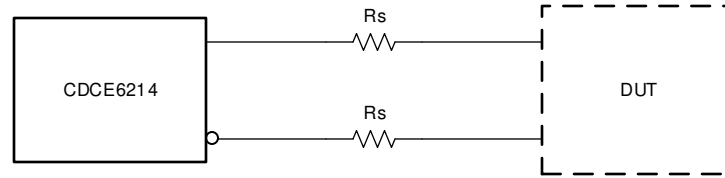
Figure 6-14. LP-HCSL Output
