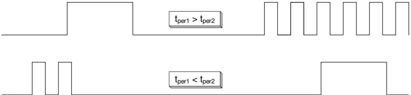
Figure 7-8. Glitchless Divider Update
