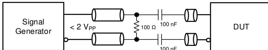
Figure 6-10. Differential Input to Reference
