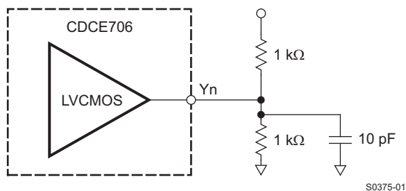
Figure 1. Test Load
