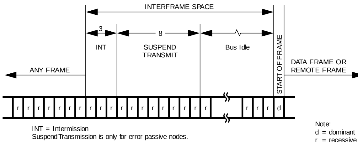
Figure 22-9. Interframe Space
