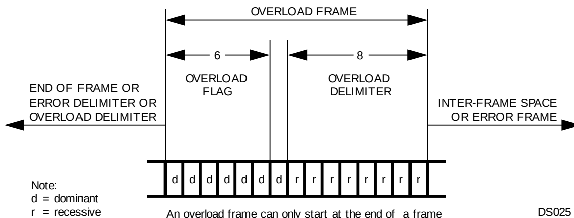
Figure 22-8. Overload Frame
