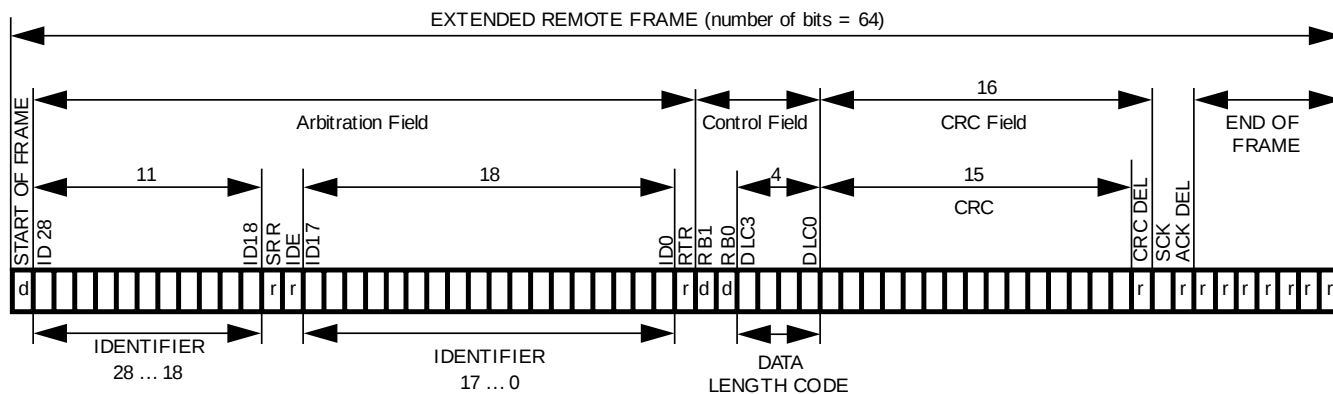
Figure 22-5. Standard Remote Frame
