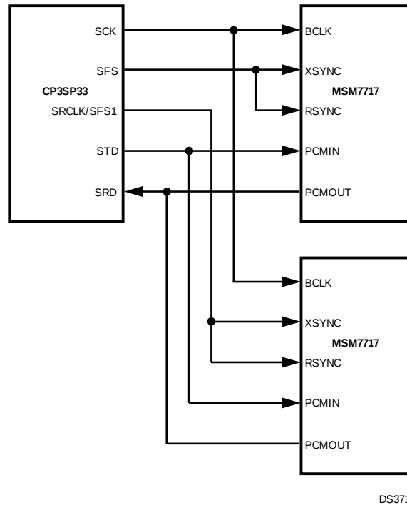
Figure 24-11. Interface to Two External Codecs
