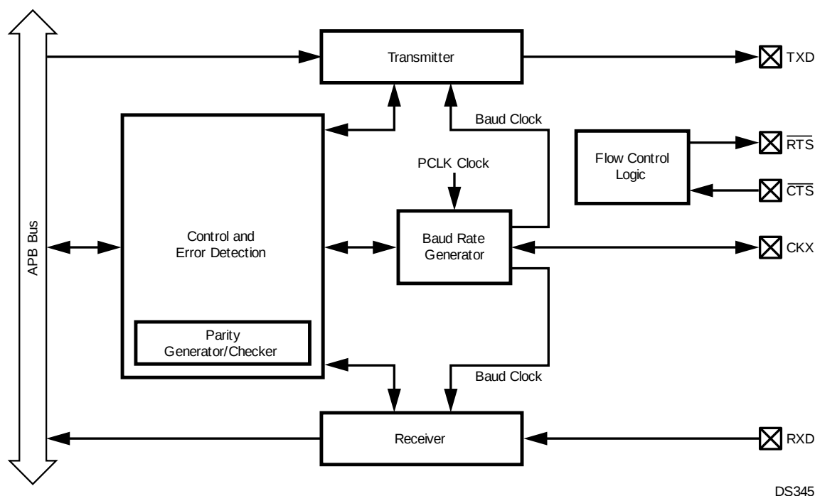
Figure 27-1. UART Block Diagram
