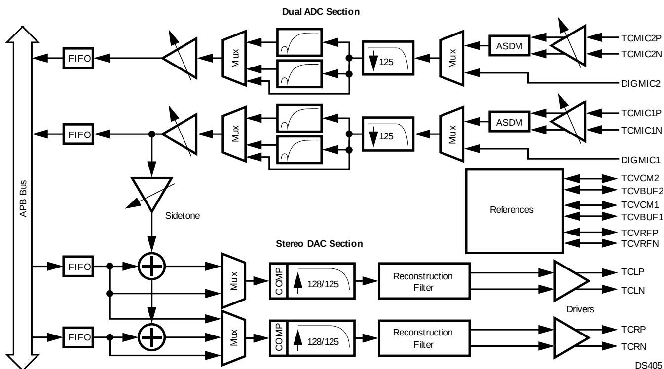
Figure 20-1. Telematics Codec
