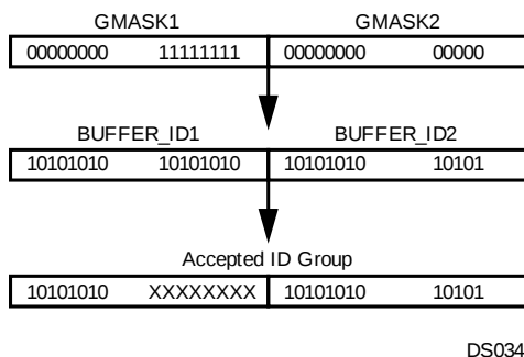
Figure 22-17. Acceptance of a Group of Identifiers
