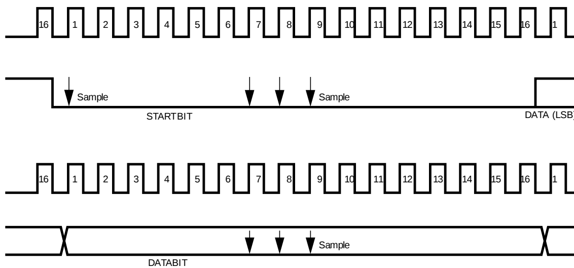
Figure 27-2. UART Asynchronous Communication
