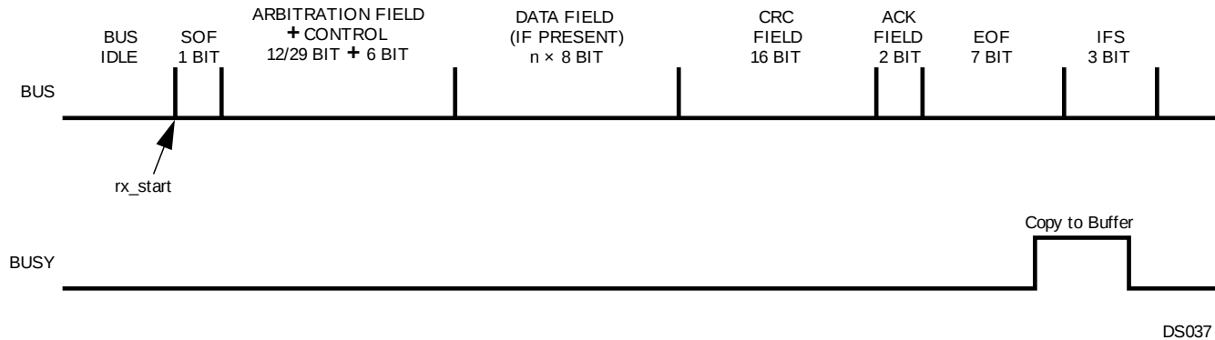
Figure 22-20. Receive Timing
