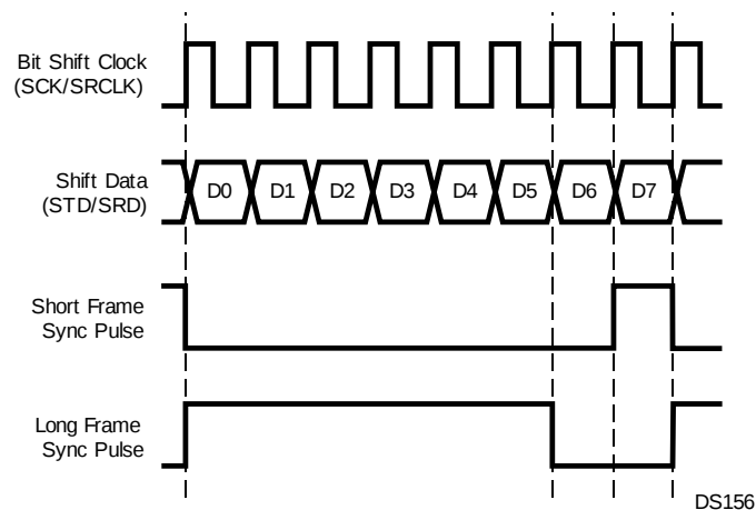
Figure 24-7. Short and Long Frame Sync Pulses
