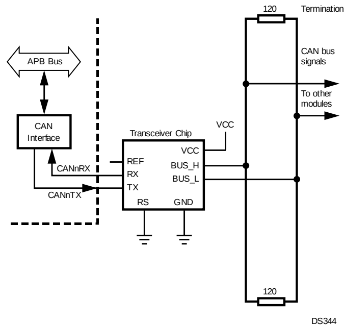
Figure 22-31. External Transceiver
