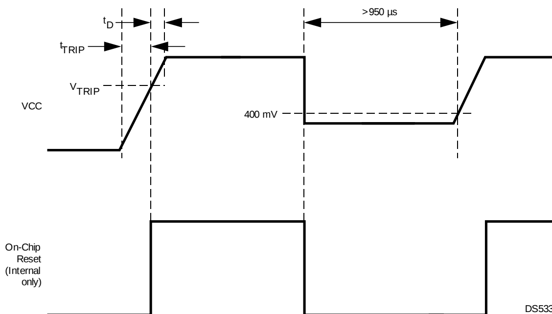
Figure 36-4. Power-On Reset
