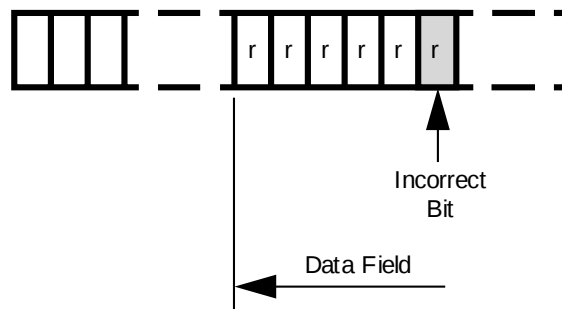
Figure 22-30. EBID Example
