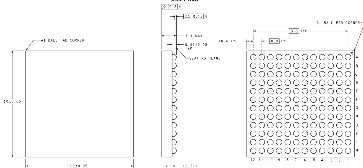
FBGA PACKAGE 144-PINS
