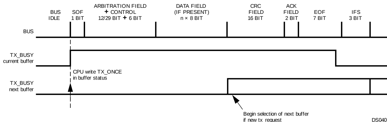
Figure 22-23. Data Transmission
