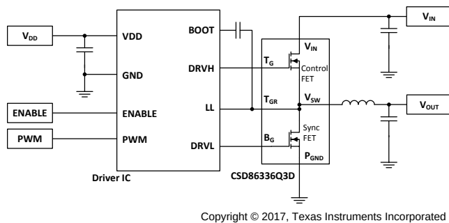
Typical Circuit
