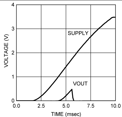
Figure 25. Power-On Reset
