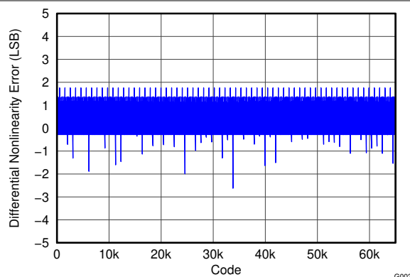
Figure 5-2. Differential Nonlinearity
