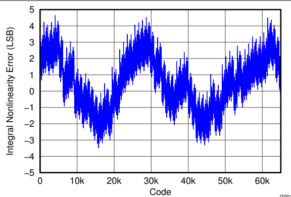
Figure 5-1. Integral Nonlinearity
