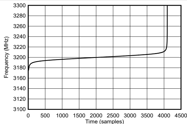
Figure 9-13. NLFM Frequency Ramp
