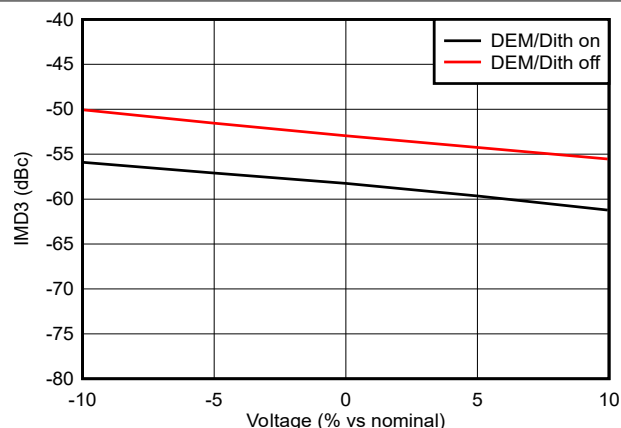
Figure 6-154. IMD3 vs Voltage in RF Mode at 7247MHz
