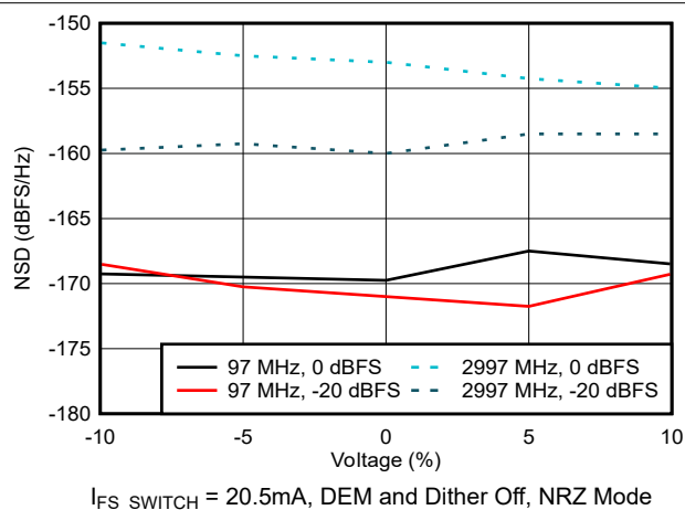
Figure 6-85. NSD vs Supply Voltage
