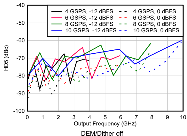
Figure 6-205. HD5 vs Frequency and Sample Rate in NRZ/RF Modes
