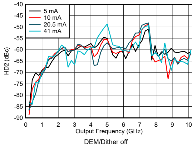
Figure 6-156. HD2 vs Frequency and Output Current in NRZ/RF Modes
