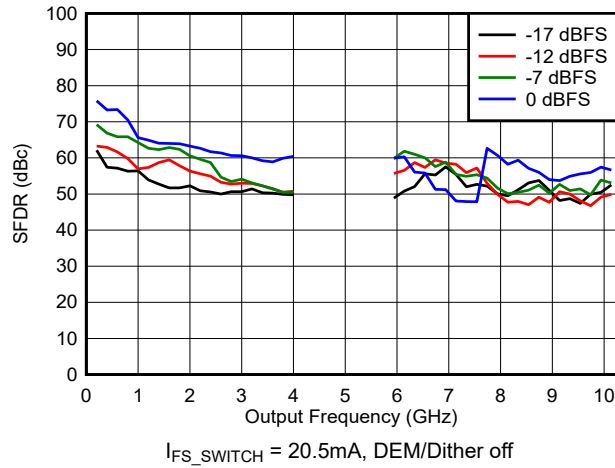
Figure 6-120. SFDR vs Frequency and Digital Amplitude in DES2X Modes
