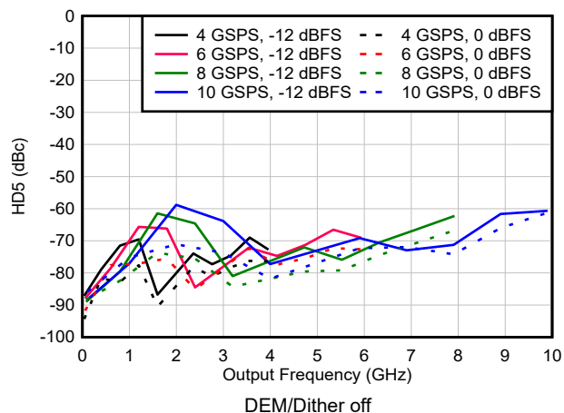
Figure 6-207. HD5 vs Frequency and Sample Rate in DES2X Modes
