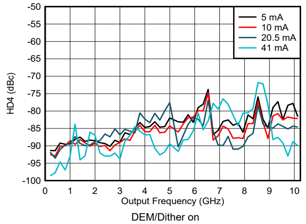
Figure 6-189. HD4 vs Frequency and Output Current in NRZ/RF Modes
