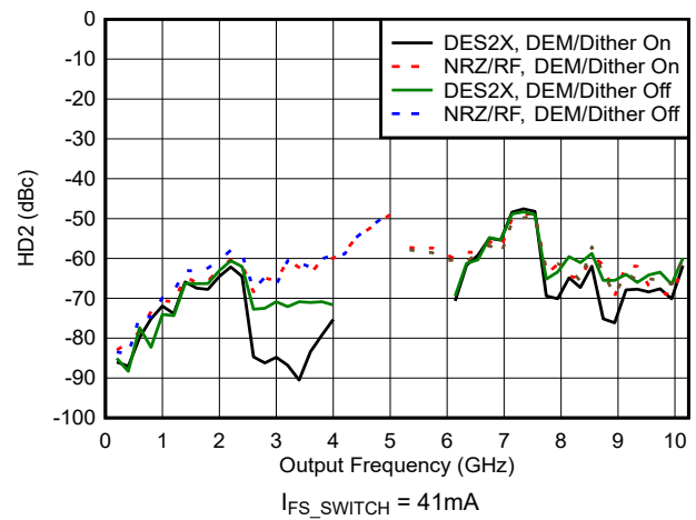
Figure 6-109. HD2 vs Frequency and Mode
