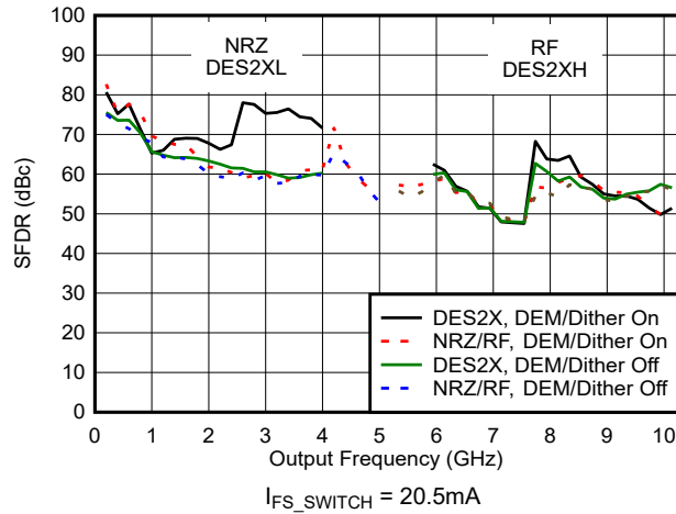
Figure 6-104. SFDR vs Frequency and Mode
