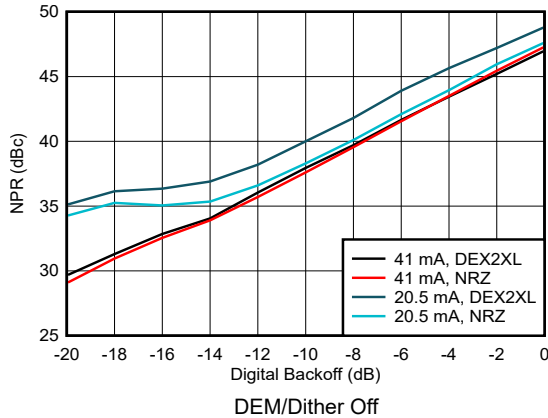
Figure 6-210. Noise Power Ratio vs Digital Backoff: 1 st Nyquist Zone
