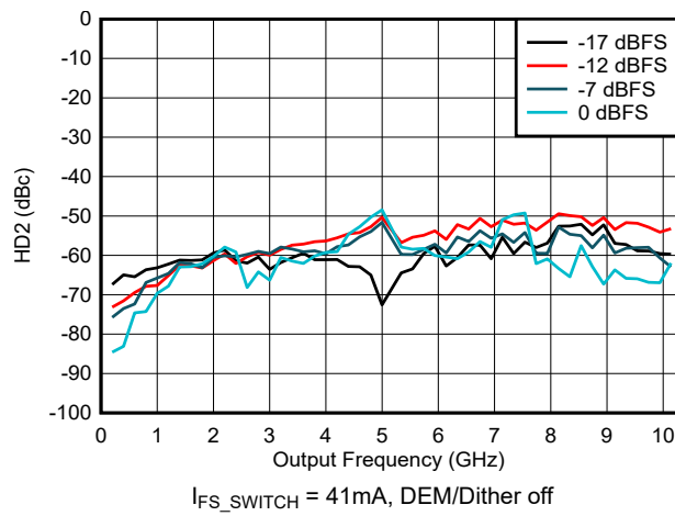
Figure 6-162. HD2 vs Frequency and Digital Amplitude in NRZ/RF Modes
