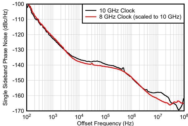
Figure 9-12. 8GHz and 10GHz Clock Phase Noise
