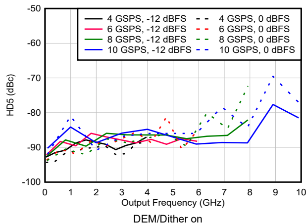
Figure 6-204. HD5 vs Frequency and Sample Rate in NRZ/RF Modes
