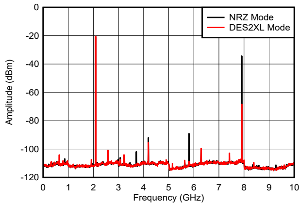
Figure 6-25. f_{\text{OUT}} = 2097\text{ MHz} , 0dBFS
