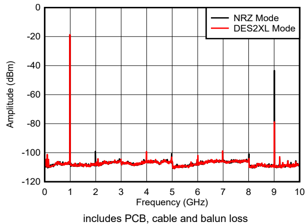
Figure 6-24. f_{\text{OUT}} = 997\text{ MHz} , -12dBFS
