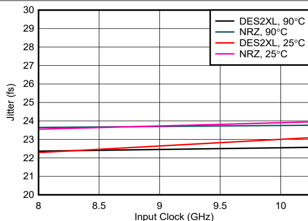
Figure 6-222. Jitter vs Input Clock
