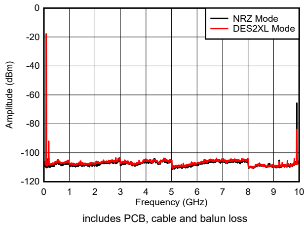
Figure 6-21. f_{\text{OUT}} = 97\text{ MHz} , -12dBFS
