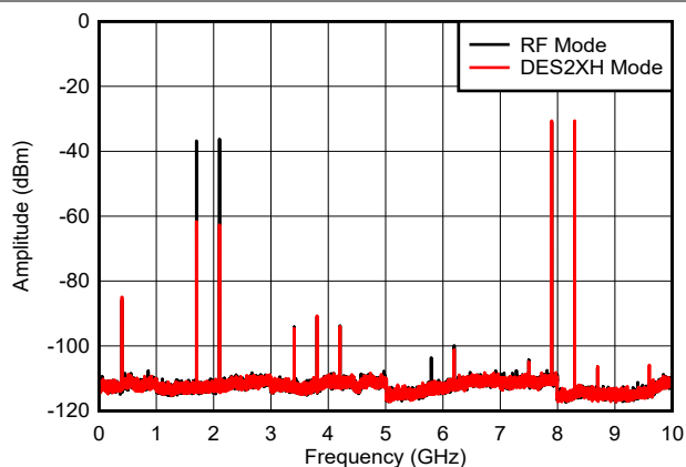
Figure 6-57. Dual Tone, f_{\text{OUT}} = 7997\text{MHz} , -12dBFS
