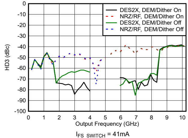
Figure 6-111. HD3 vs Frequency and Mode
