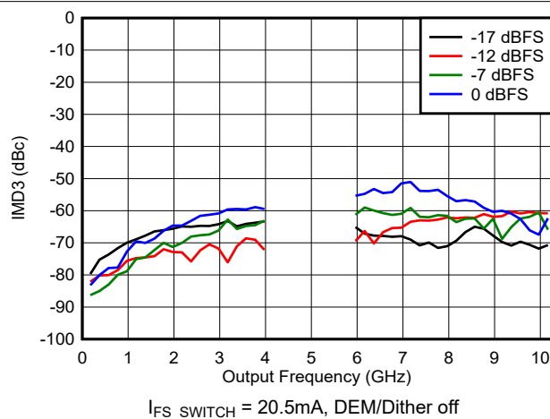
Figure 6-136. IMD3 vs Frequency and Digital Amplitude in DES2X Modes
