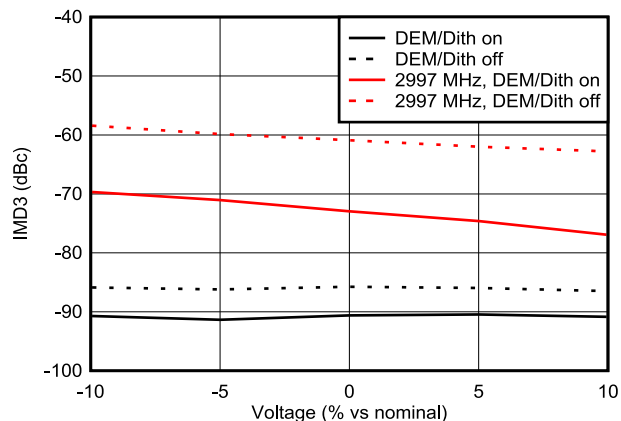
Figure 6-153. IMD3 vs Voltage in DES2XL Mode
