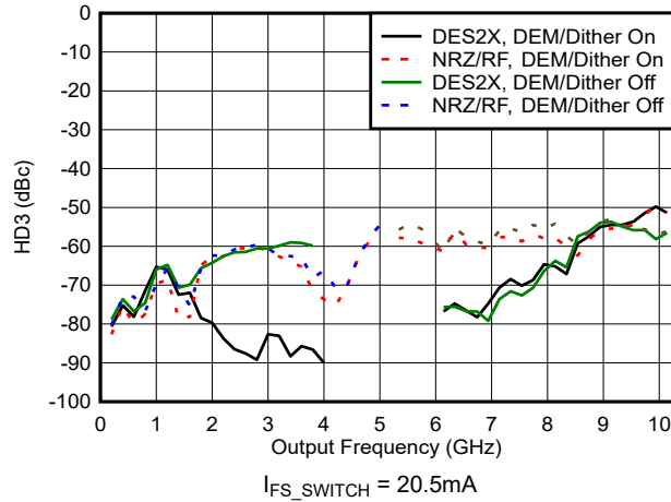
Figure 6-110. HD3 vs Frequency and Mode
