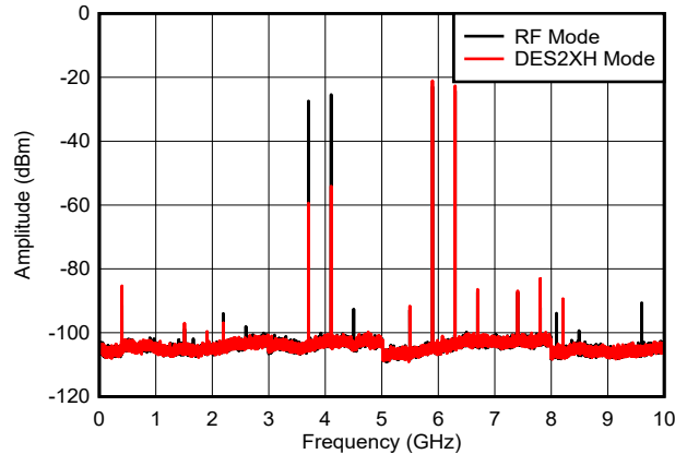
Figure 6-53. Dual Tone, f_{\text{OUT}} = 6097\text{ MHz} , -6dBFS
