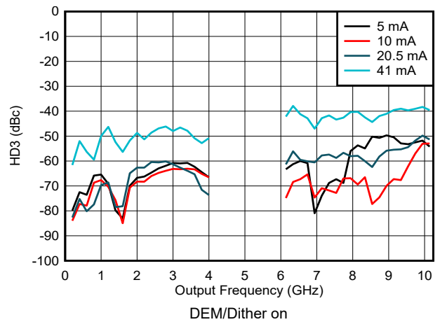
Figure 6-173. HD3 vs Frequency and Output Current in NRZ/RF Modes
