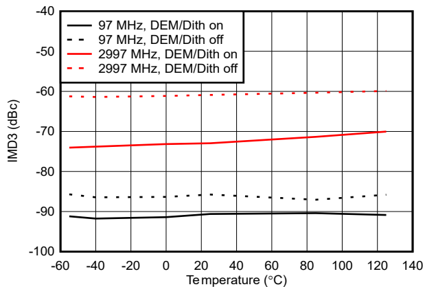
Figure 6-149. IMD3 vs Temperature in DES2XL Mode
