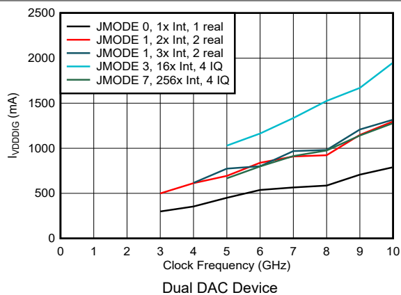
Figure 6-102. VDDDIG Current vs Clock Frequency and Digital Mode
