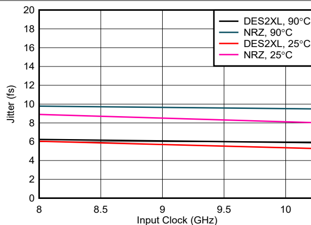
Figure 6-221. Jitter vs Input Clock
