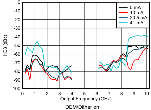
Figure 6-175. HD3 vs Frequency and Output Current in DES2X Modes
