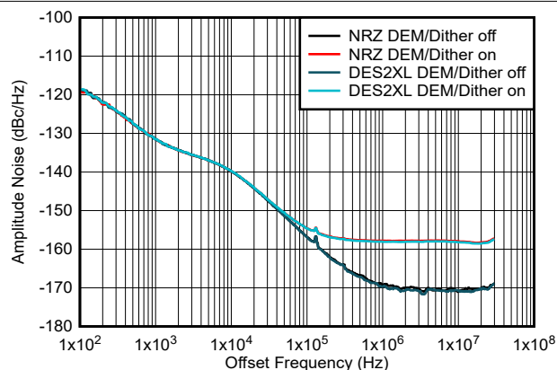
Figure 6-223. Amplitude Noise vs Offset Frequency at 1GHz
