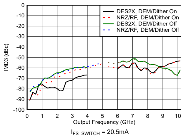
Figure 6-106. IMD3 vs Frequency and Mode
