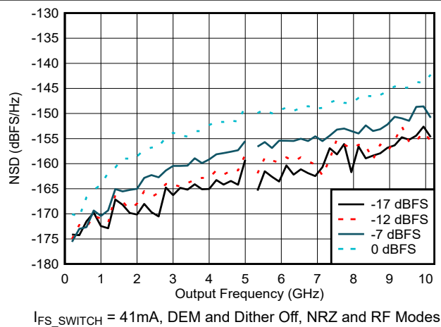
Figure 6-66. NSD vs Output Frequency and Digital Amplitude
