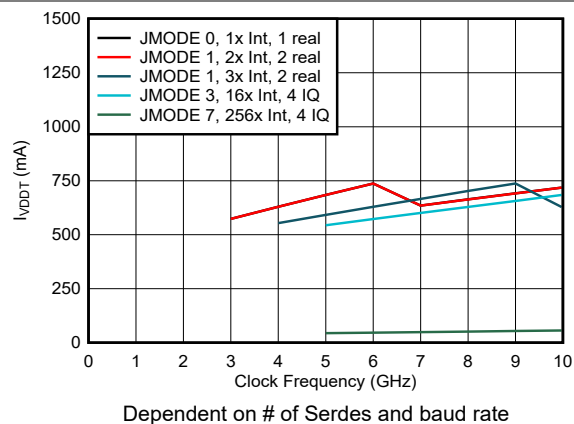
Figure 6-101. VDDT Current vs Clock Frequency and Mode
