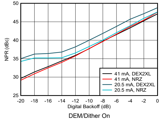
Figure 6-211. Noise Power Ratio vs Digital Backoff: 1 st Nyquist Zone
