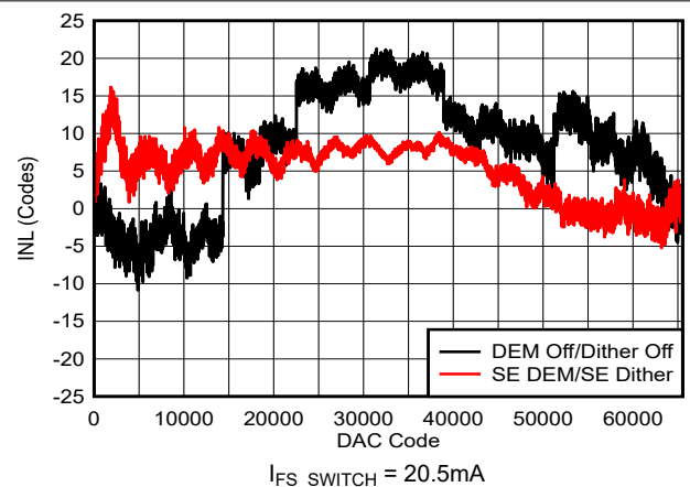
Figure 6-13. INL vs DAC Code: 20.5mA
