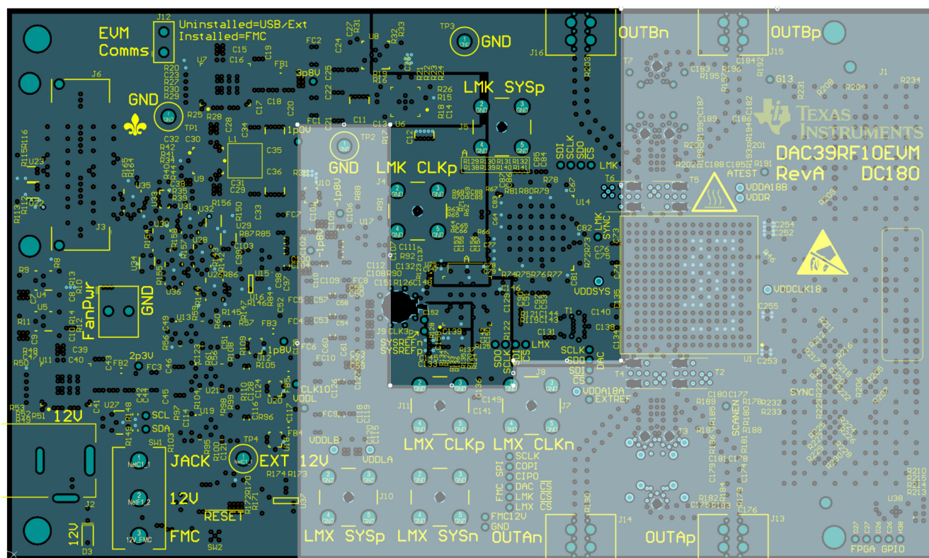
Layer3 / PWR1 DAC DVDD = WHITE Other PWR Planes = AUX Supplies Figure 9-29. Power Plane Layout for Layer 3
