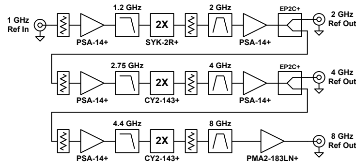
Figure 9-10. Reference Multiplier Chain
