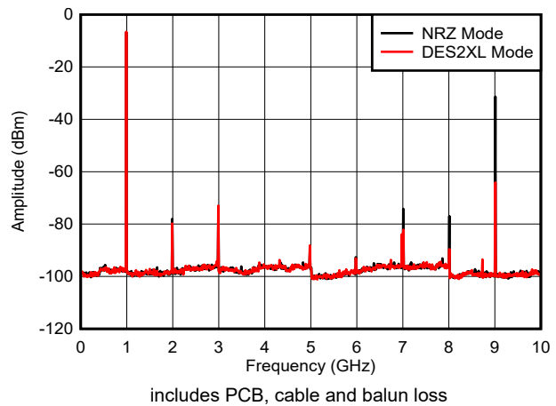
Figure 6-22. f_{\text{OUT}} = 997\text{ MHz} , 0dBFS
