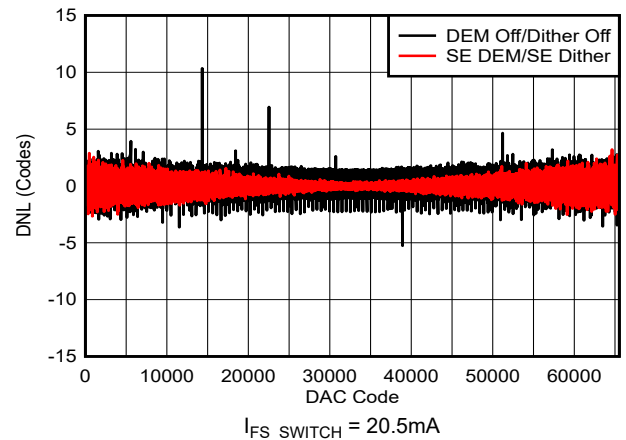
Figure 6-11. DNL vs DAC Code: 20.5mA
