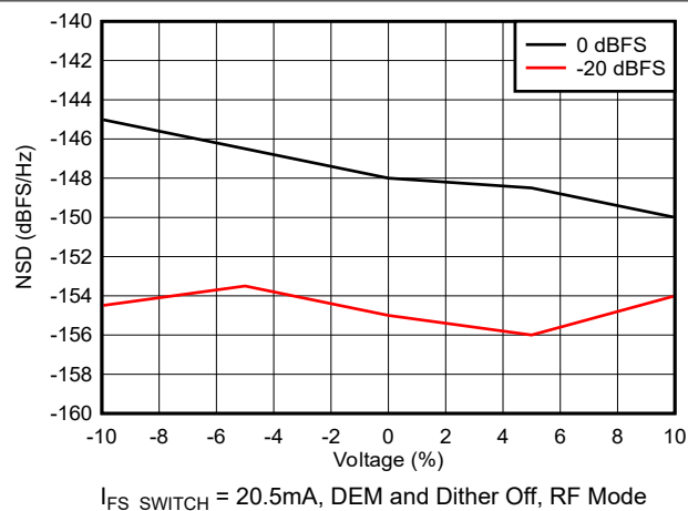
Figure 6-86. NSD vs Supply Voltage
