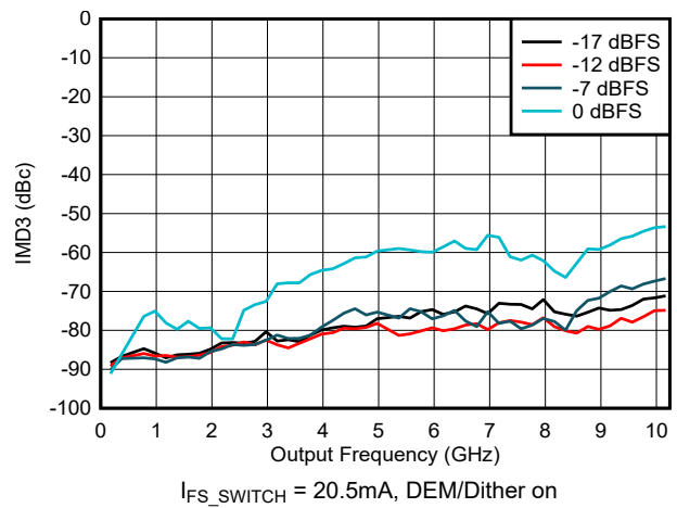
Figure 6-133. IMD3 vs Frequency and Digital Amplitude in NRZ/RF Modes
