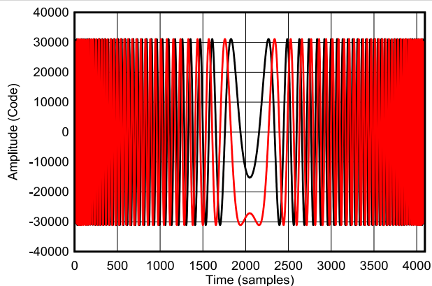
Figure 9-14. Complex Time Domain of NLFM Chirp (Red = real, Black = imag)
