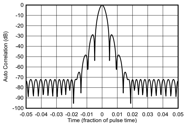
Figure 9-16. Auto-correlation of NLFM Chirp
