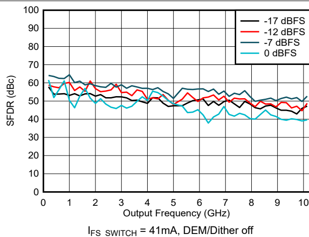
Figure 6-118. SFDR vs Frequency and Digital Amplitude in NRZ/RF Modes
