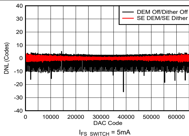
Figure 6-12. DNL vs DAC Code: 5mA
