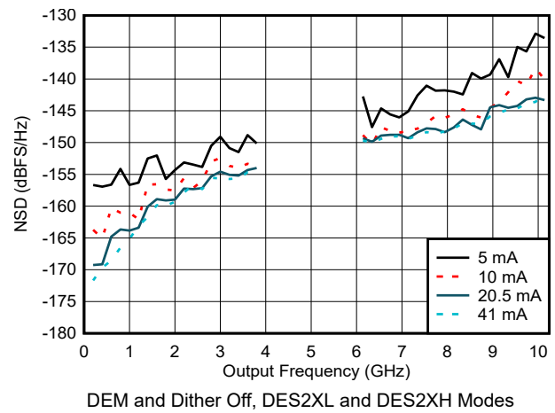
Figure 6-63. NSD vs Output Frequency and Output Current
