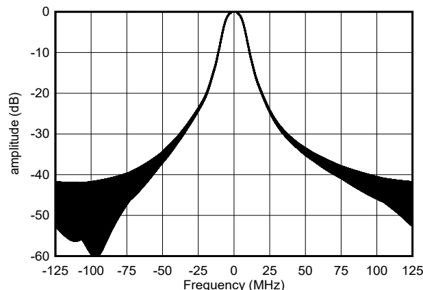
Figure 9-15. Digital Spectrum for NLFM Chirp
