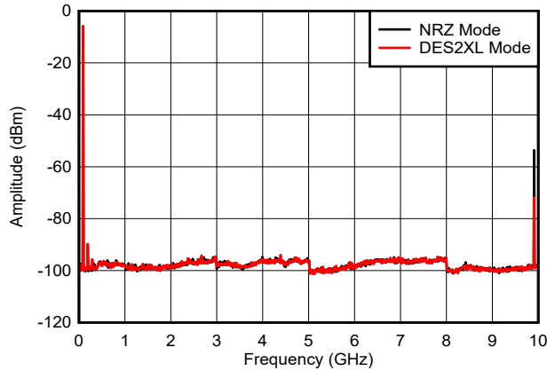
Figure 6-19. f_{\text{OUT}} = 97\text{ MHz} , 0dBFS
