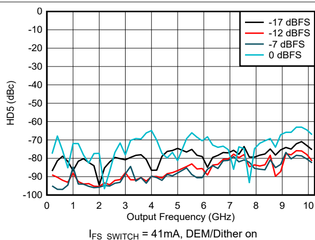
Figure 6-199. HD5 vs Frequency and Digital Amplitude in NRZ/RF Modes
