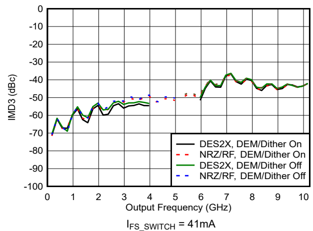
Figure 6-107. IMD3 vs Frequency and Mode
