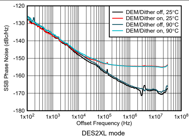
Figure 6-220. Phase Noise vs Offset Frequency at 1GHz
