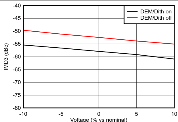
Figure 6-155. IMD3 vs Voltage in DES2XH Mode at 7247MHz
