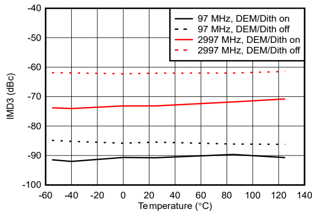
Figure 6-148. IMD3 vs Temperature in NRZ Mode
