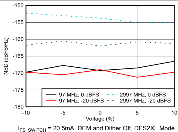
Figure 6-87. NSD vs Supply Voltage
