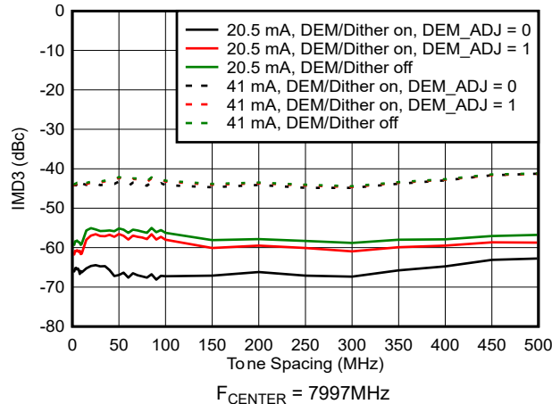
Figure 6-142. IMD3 vs Tone Spacing in RF Mode
