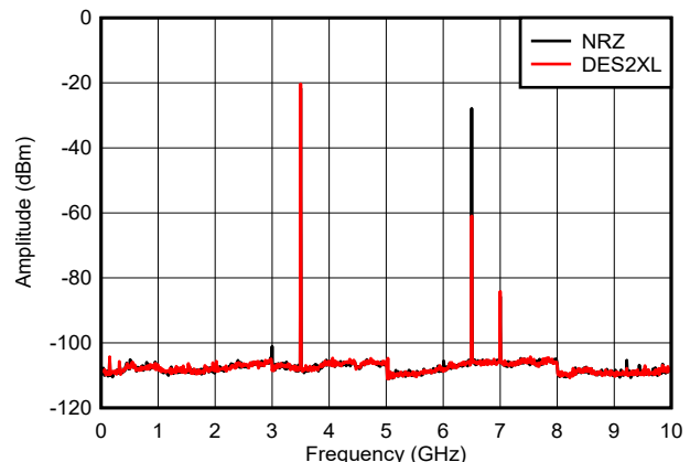
Figure 6-28. f_{\text{OUT}} = 3497\text{ MHz} , 0dBFS
