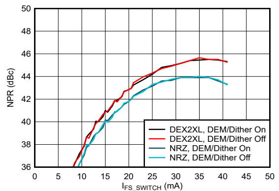
Figure 6-215. Noise Power Ratio vs Output Current: 2 nd Nyquist Zone
