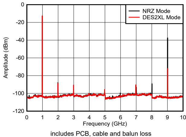
Figure 6-23. f_{\text{OUT}} = 997\text{ MHz} , -6dBFS
