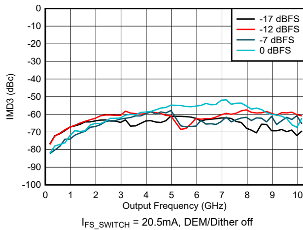
Figure 6-132. IMD3 vs Frequency and Digital Amplitude in NRZ/RF Modes
