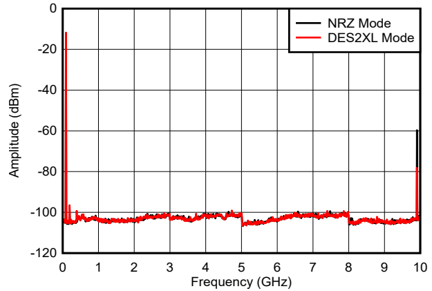
Figure 6-20. f_{\text{OUT}} = 97\text{ MHz} , -6dBFS
