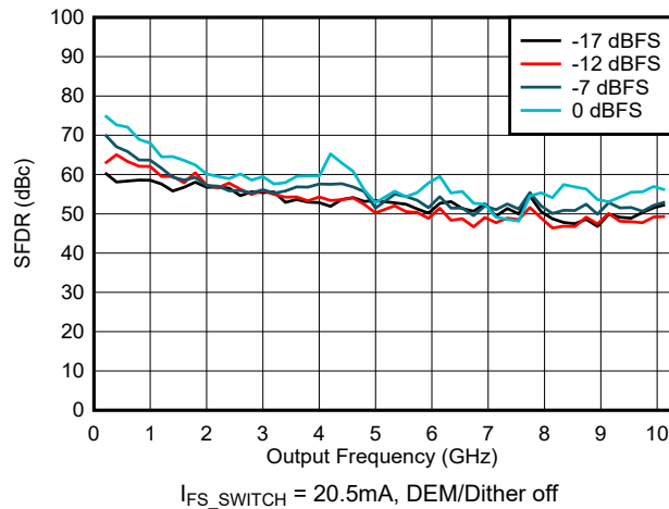
Figure 6-116. SFDR vs Frequency and Digital Amplitude in NRZ/RF Modes
