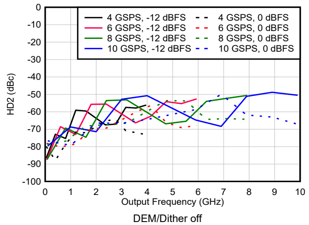
Figure 6-171. HD2 vs Frequency and Sample Rate in DES2X Modes
