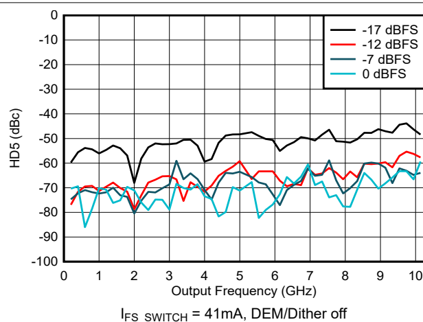
Figure 6-198. HD5 vs Frequency and Digital Amplitude in NRZ/RF Modes
