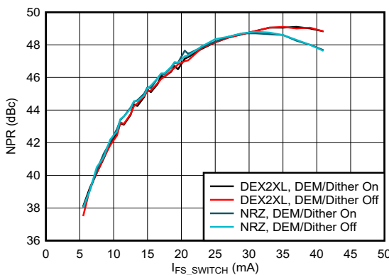
Figure 6-214. Noise Power Ratio vs Output Current: 1 st Nyquist Zone
