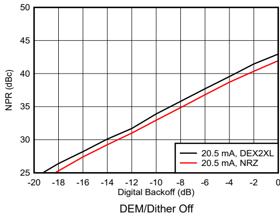
Figure 6-212. Noise Power Ratio vs Digital Backoff: 2 nd Nyquist Zone
