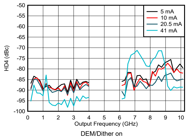
Figure 6-191. HD4 vs Frequency and Output Current in DES2X Modes
