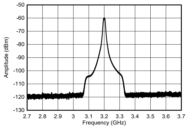
Figure 9-18. NLFM Chirp Output Spectra Across 1GHz
