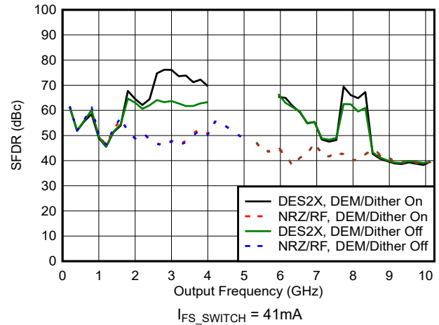
Figure 6-105. SFDR vs Frequency and Mode
