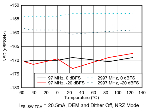
Figure 6-81. NSD vs Temperature
