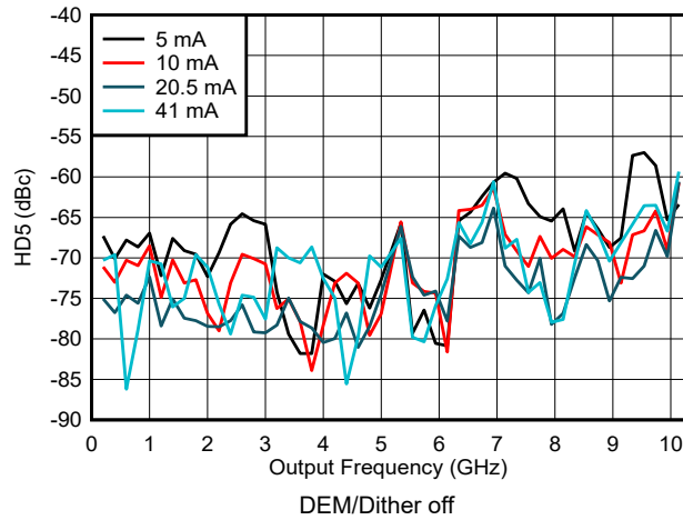
Figure 6-192. HD5 vs Frequency and Output Current in NRZ/RF Modes
