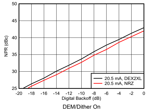
Figure 6-213. Noise Power Ratio vs Digital Backoff: 2 nd Nyquist Zone
