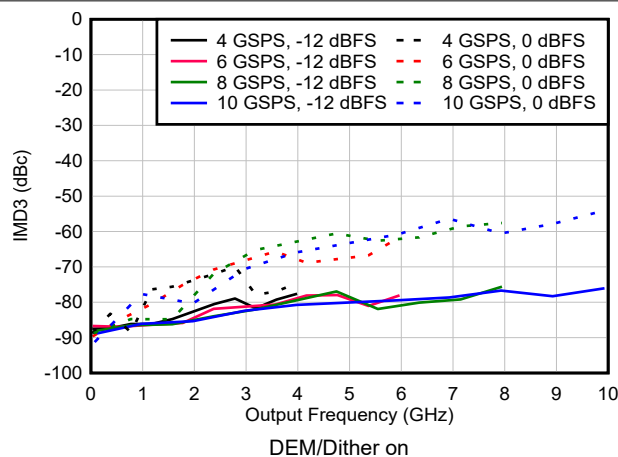
Figure 6-144. IMD3 vs Frequency and Sample Rate in NRZ/RF Modes
