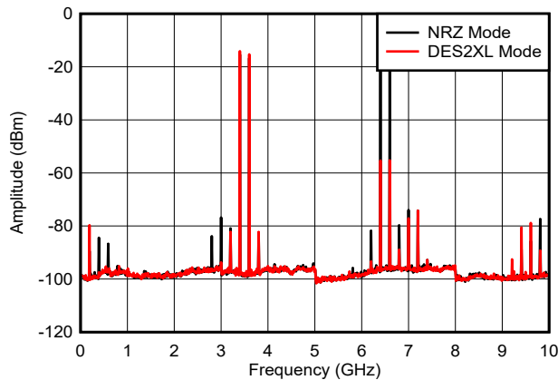
Figure 6-47. Dual Tone, f_{\text{OUT}} = 2097\text{MHz} , -6dBFS
