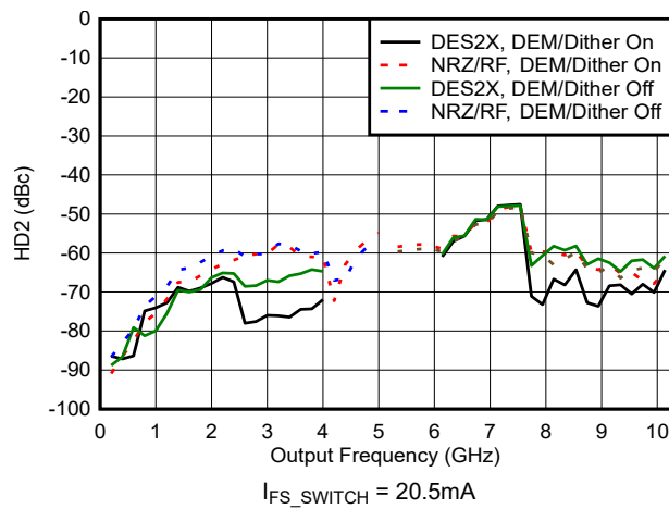
Figure 6-108. HD2 vs Frequency and Mode
