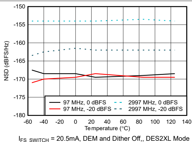
Figure 6-83. NSD vs Temperature
