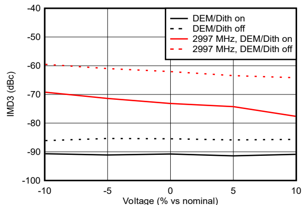
Figure 6-152. IMD3 vs Voltage in NRZ Mode
