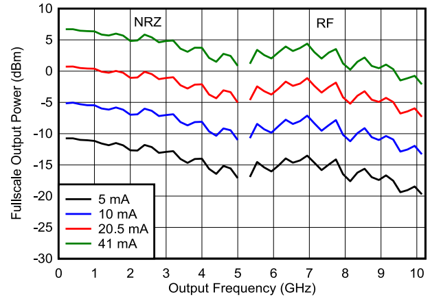
Figure 6-9. Output Power vs Frequency (NRZ/RF modes)
