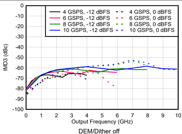
Figure 6-145. IMD3 vs Frequency and Sample Rate in NRZ/RF Modes
