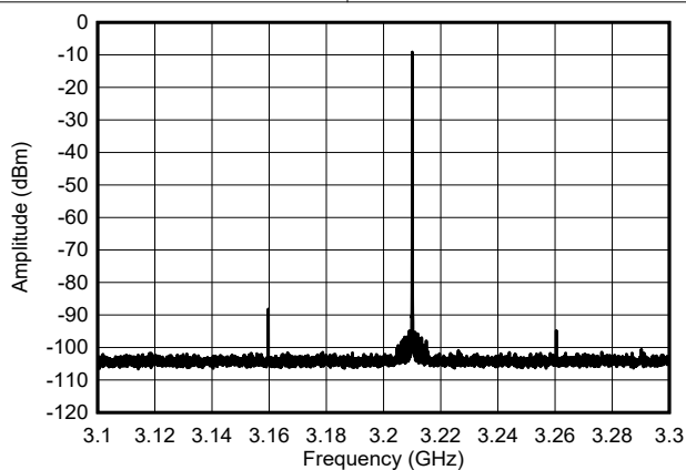
Figure 9-19. In Band Single Tone Frequency Spectra with f_{OUT} = 3.211\text{GHz}
