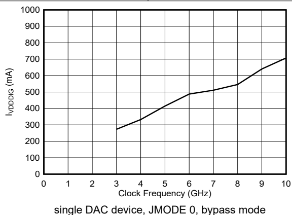
Figure 6-103. VDDDIG Current vs Clock Frequency
