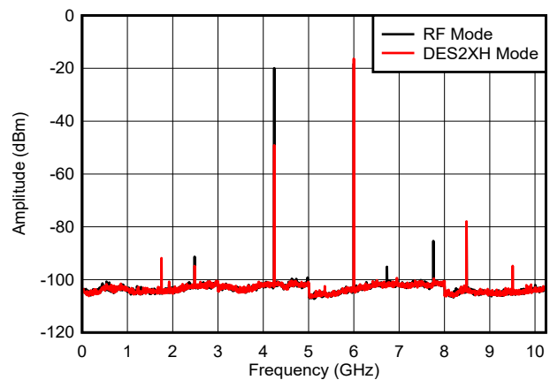
Figure 6-21. f_{\text{OUT}} = 5997\text{ MHz} , -6 dBFS
