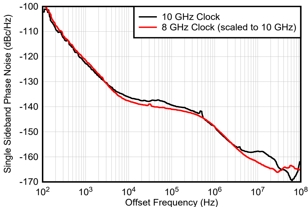
Figure 8-12. 8 GHz and 10 GHz Clock Phase Noise
