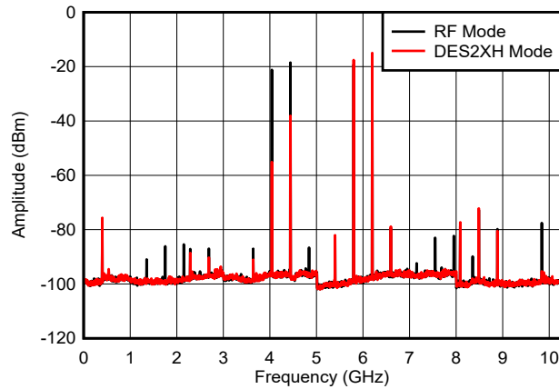
Figure 6-38. Dual Tone, f_{\text{OUT}} = 5997\text{ MHz} , 0 dBFS
