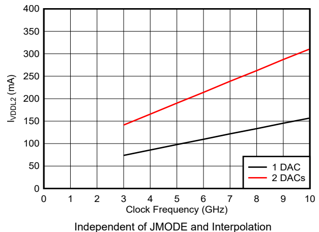
Figure 6-49. VDDLx Current vs Clock Frequency
