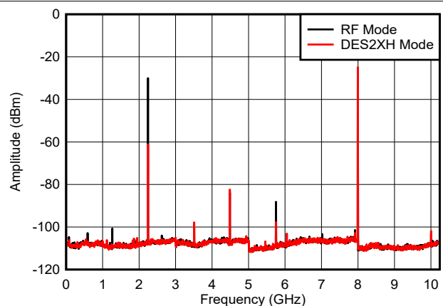
Figure 6-23. f_{\text{OUT}} = 7997\text{ MHz} , 0 dBFS
