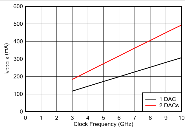
Independent of JMODE and Interpolation Figure 6-50. VDDCLK Current vs Clock Frequency
