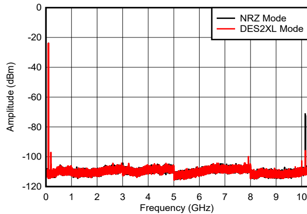
Figure 6-26. Dual Tone, f_{\text{OUT}} = 97\text{ MHz} , 0 dBFS
