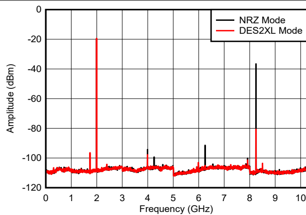
Figure 6-14. f_{\text{OUT}} = 1997\text{ MHz} , 0 dBFS
