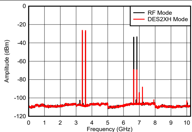
Figure 6-35. Dual Tone, f_{\text{OUT}} = 3497\text{ MHz} , 0 dBFS
