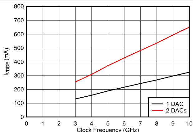
Independent of JMODE and Interpolation Figure 6-51. VDDE Current vs Clock Frequency
