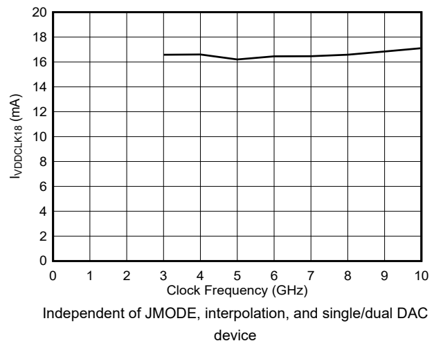
Figure 6-47. VDDCLK18 Current vs Clock Frequency
