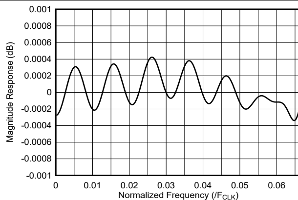
Figure 7-21. 6x Interpolation Filter Passband Response
