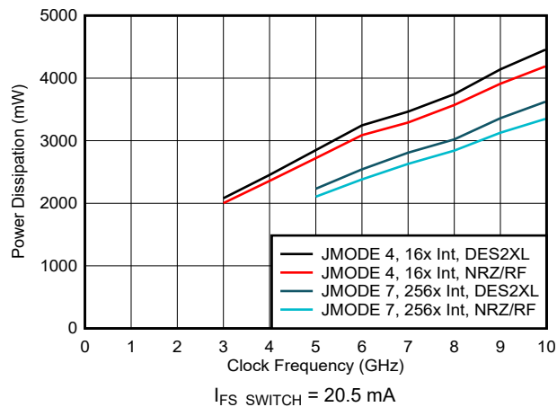
Figure 6-44. Power Dissipation vs Clock Frequency and Digital Mode
