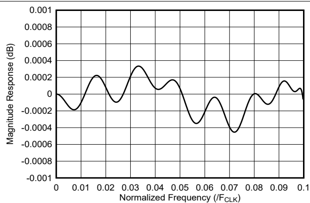
Figure 7-19. 4x Interpolation Filter Passband Response
