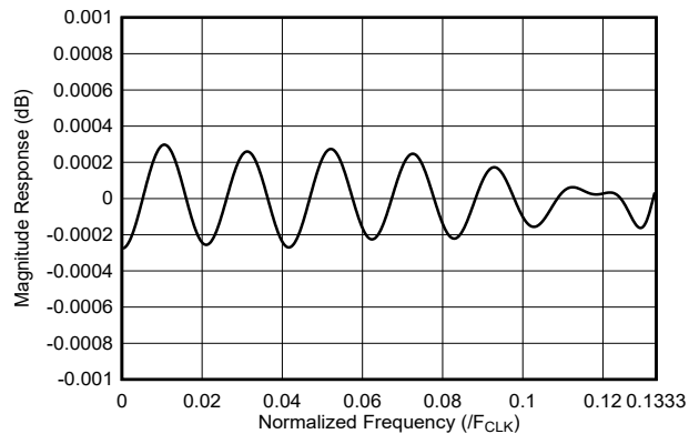
Figure 7-17. 3x Interpolation Filter Passband Response
