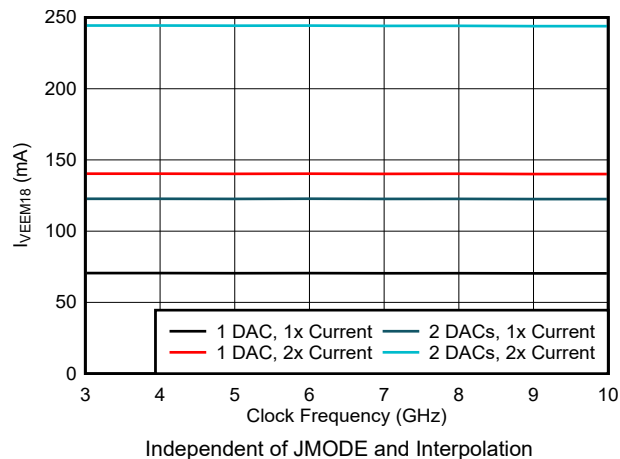
Figure 6-48. VEEM18 Current vs Clock Frequency and Output Current
