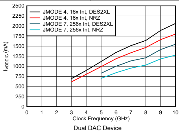
Dual DAC Device Figure 6-54. VDDDIG Current vs Clock Frequency and Digital Mode
