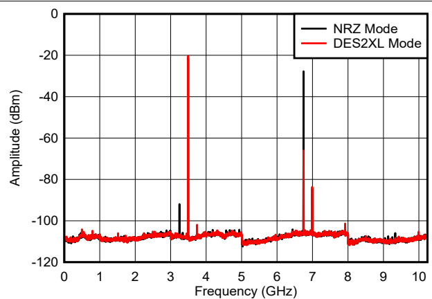
Figure 6-17. f_{\text{OUT}} = 3497\text{ MHz} , 0 dBFS
