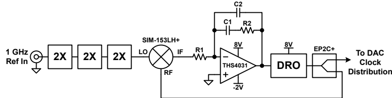
Figure 8-9. Discrete Analog PLL
