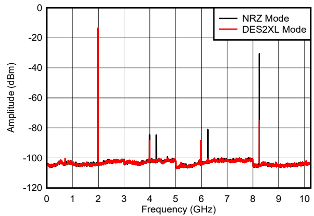
Figure 6-15. f_{\text{OUT}} = 1997\text{ MHz} , -6 dBFS
