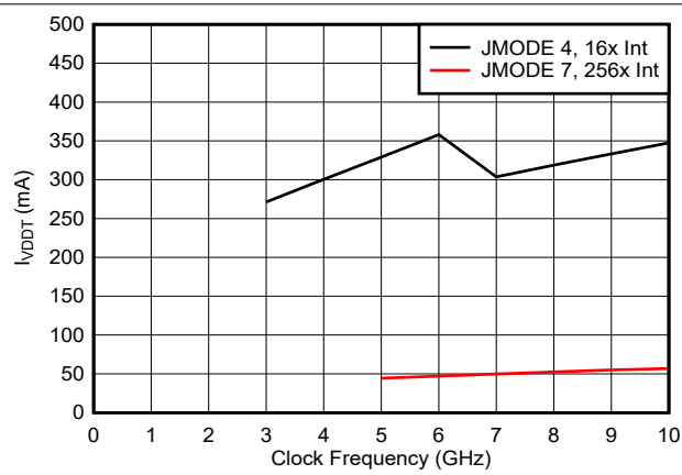
Dependent on # of Serdes and baud rate Figure 6-53. VDDT Current vs Clock Frequency and Interface Mode
