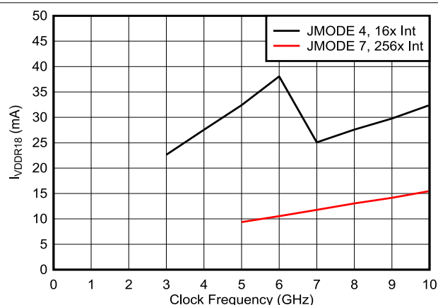
Dependent on # of Serdes and baud rate Figure 6-52. VDDR18 Current vs Clock Frequency and Interface Mode
