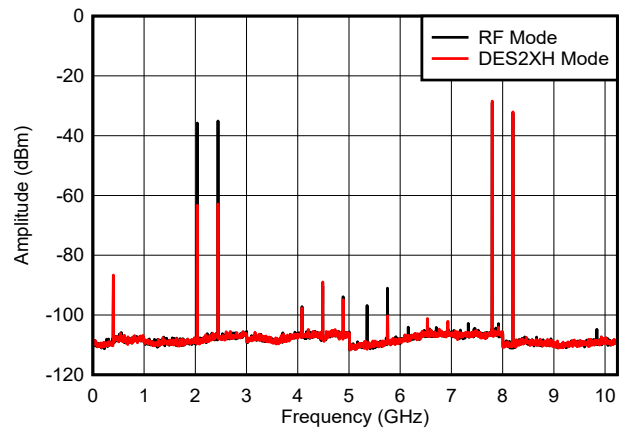
Figure 6-41. Dual Tone, f_{\text{OUT}} = 7997\text{ MHz} , 0 dBFS
