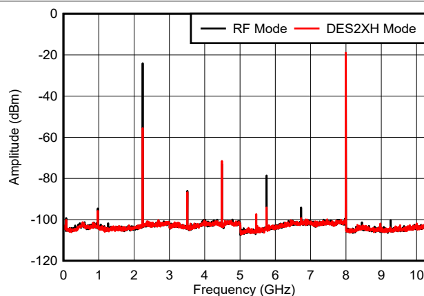
Figure 6-22. f_{\text{OUT}} = 5997\text{ MHz} , -12 dBFS
