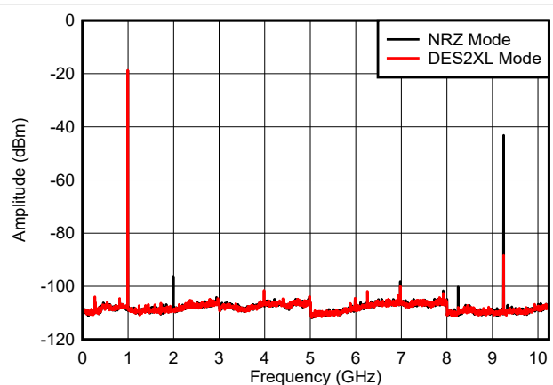
Figure 6-11. f_{\text{OUT}} = 997\text{ MHz} , 0 dBFS
