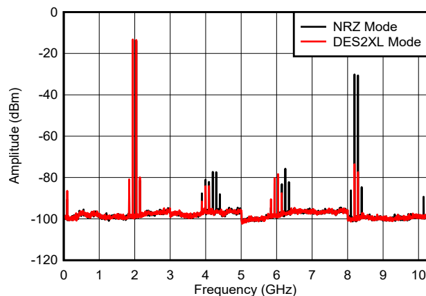
Figure 6-32. Dual Tone, f_{\text{OUT}} = 1997\text{ MHz} , 0 dBFS
