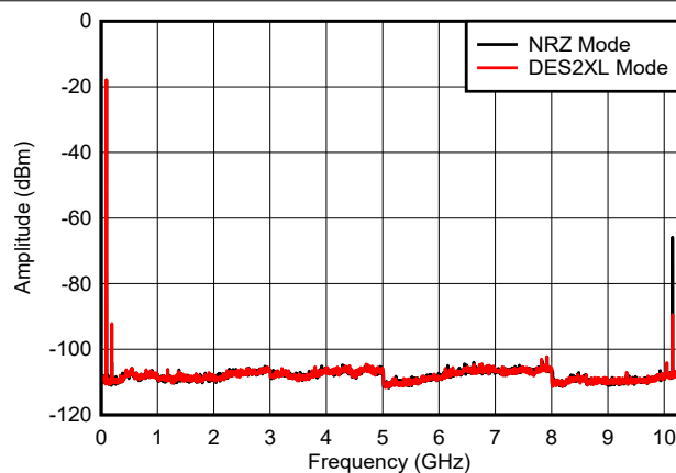
Figure 6-8. f_{\text{OUT}} = 97\text{ MHz} , 0 dBFS
