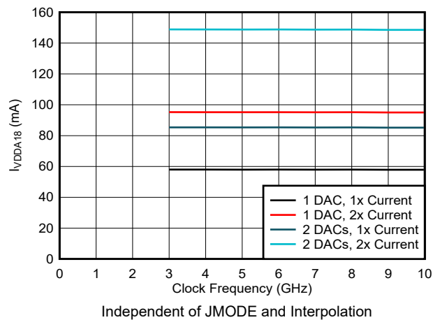
Figure 6-46. VDDA18 Current vs Clock Frequency and DAC Mode
