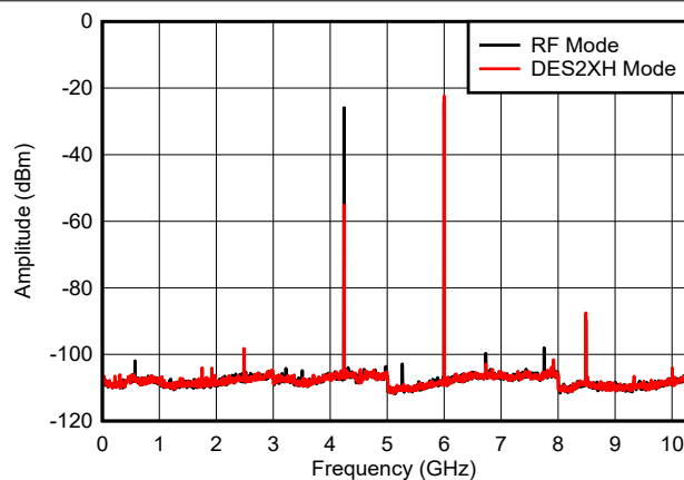
Figure 6-20. f_{\text{OUT}} = 5997\text{ MHz} , 0 dBFS
