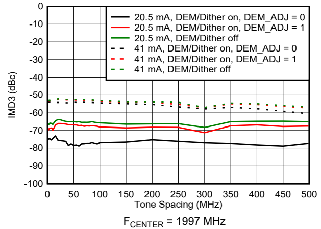
Figure 6-119. IMD3 vs Tone Spacing in DES2XL Mode
