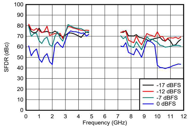
Figure 6-99. SFDR vs Frequency and Digital Amplitude in DES2X Modes
