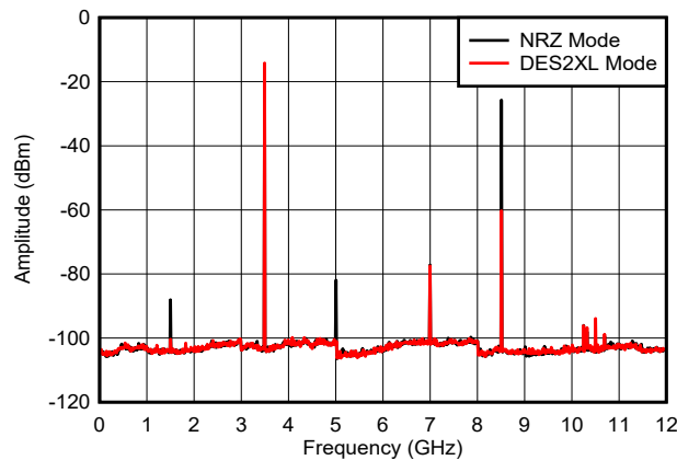
includes PCB, cable and balun loss Figure 6-27. f_{\text{OUT}} = 2097\text{ MHz} , -12 dBFS
