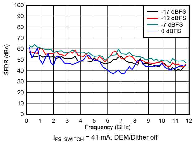
Figure 6-96. SFDR vs Frequency and Digital Amplitude in NRZ/RF Modes
