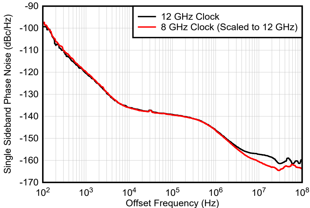
Figure 8-12. 8 GHz and 12 GHz Clock Phase Noise
