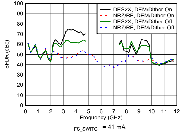
Figure 6-83. SFDR vs Frequency and Mode
