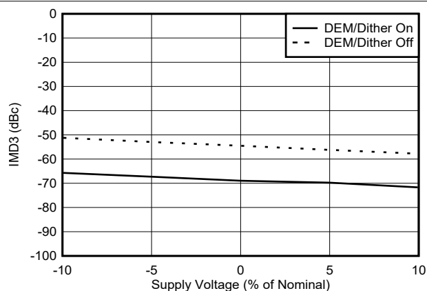
Figure 6-133. IMD3 vs Voltage in DES2XH Mode at 9002 MHz
