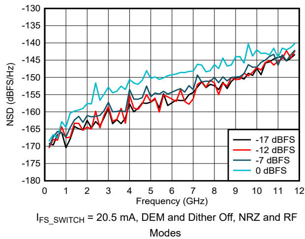
Figure 6-64. NSD vs Output Frequency and Digital Amplitude
