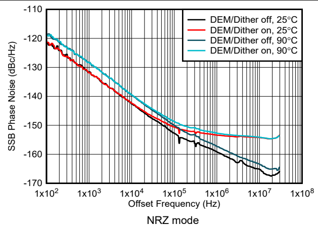
Figure 6-196. Phase Noise vs Offset Frequency at 1 GHz
