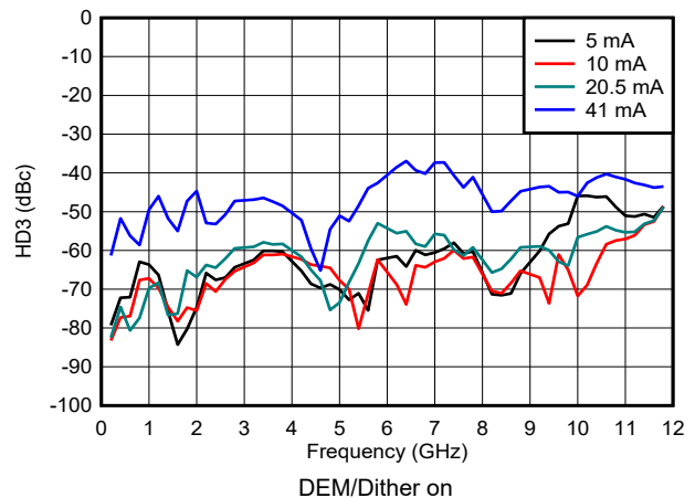
Figure 6-151. HD3 vs Frequency and Output Current in NRZ/RF Modes
