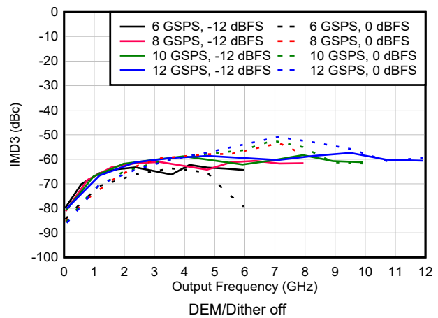
Figure 6-123. IMD3 vs Frequency and Sample Rate in NRZ/RF Modes
