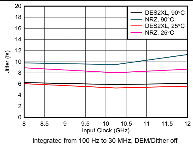
Figure 6-198. Jitter vs Input Clock
