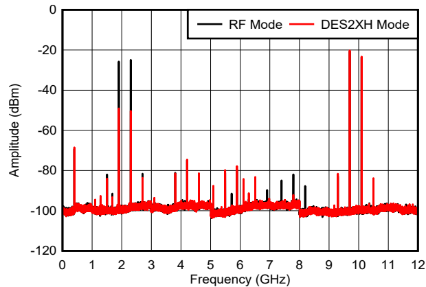
Figure 6-55. Dual Tone, f_{\text{OUT}} = 9897\text{ MHz} , 0 dBFS
