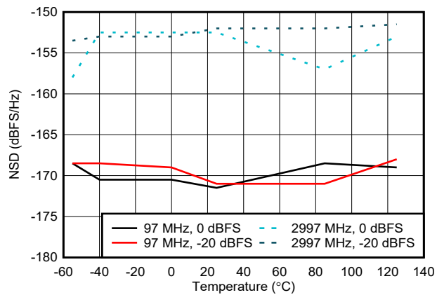
Figure 6-76. NSD vs Temperature
