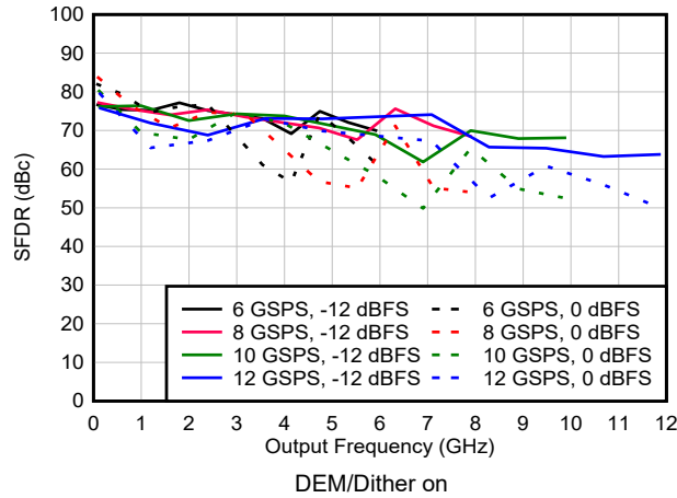
Figure 6-104. SFDR vs Frequency and Sample Rate in DES2X Modes
