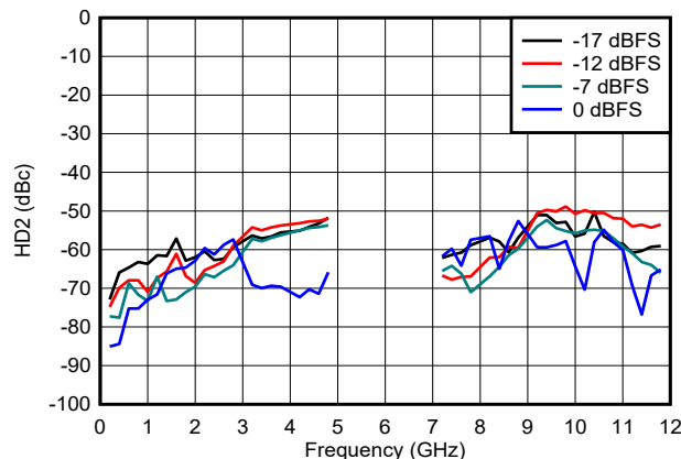
Figure 6-142. HD2 vs Frequency and Digital Amplitude in DES2X Modes
