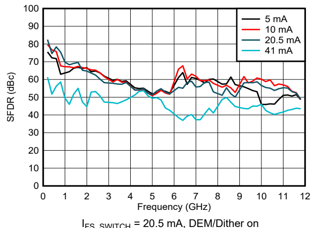
Figure 6-91. SFDR vs Frequency and Output Current in NRZ/RF Modes
