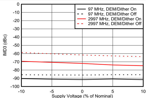
Figure 6-130. IMD3 vs Voltage in NRZ Mode
