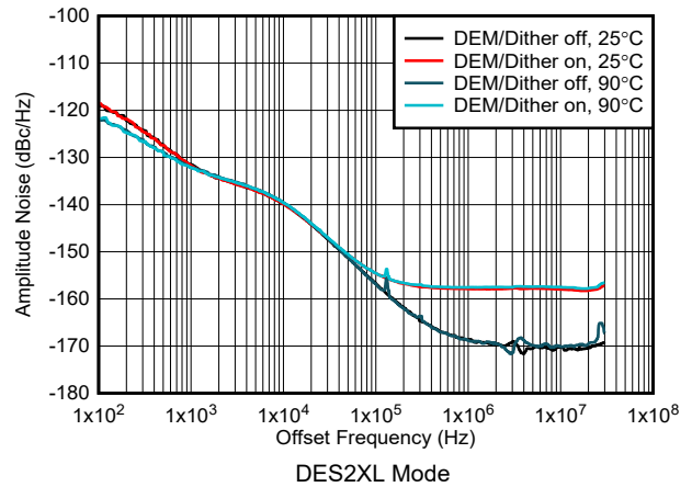
Figure 6-202. Amplitude Noise vs Offset Frequency and Temperature at 1 GHz
