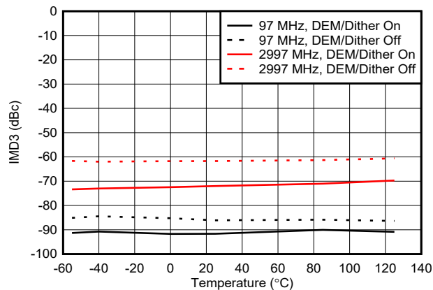
Figure 6-126. IMD3 vs Temperature in NRZ Mode
