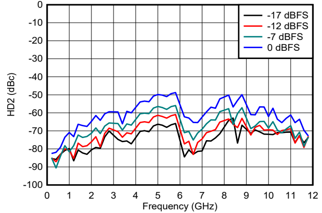
Figure 6-141. HD2 vs Frequency and Digital Amplitude in NRZ/RF Modes
