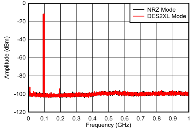
Figure 6-38. Dual Tone, f_{\text{OUT}} = 97\text{ MHz} , 0 dBFS (0 - 1 GHz)
