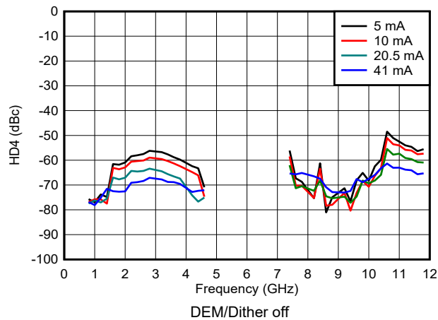
Figure 6-168. HD4 vs Frequency and Output Current in DES2X Modes
