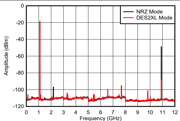
Figure 6-22. f_{\text{OUT}} = 1097\text{ MHz} , 0 dBFS
