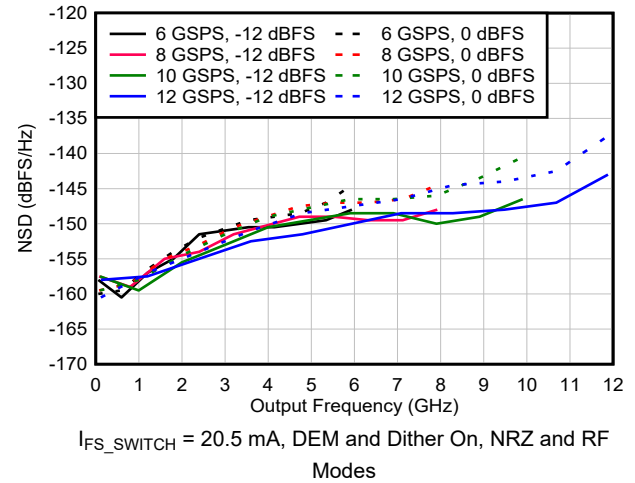
Figure 6-73. NSD vs Output Frequency and Sample Rate
