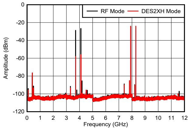
Figure 6-53. Dual Tone, f_{\text{OUT}} = 8097\text{ MHz} , -6 dBFS
