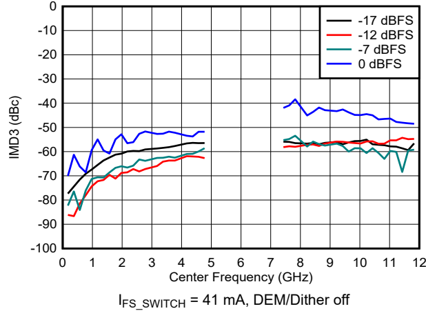
Figure 6-116. IMD3 vs Frequency and Digital Amplitude in DES2X Modes
