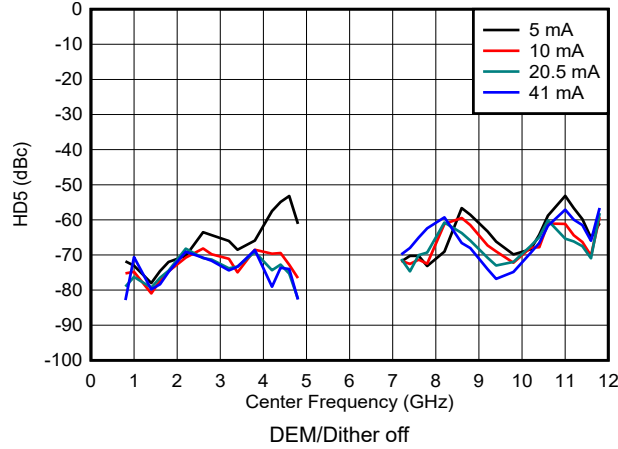
Figure 6-176. HD5 vs Frequency and Output Current in DES2X Modes
