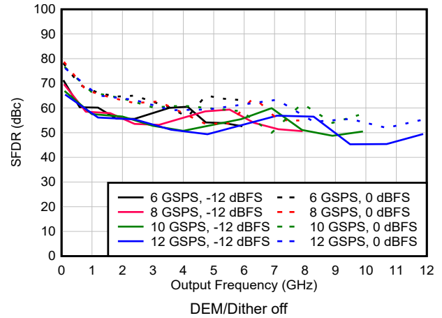
Figure 6-105. SFDR vs Frequency and Sample Rate in DES2X Modes
