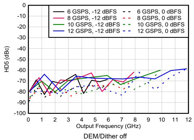
Figure 6-183. HD5 vs Frequency and Sample Rate in NRZ/RF Modes
