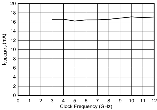
Figure 6-209. VDDCLK18 Current vs Clock Frequency
