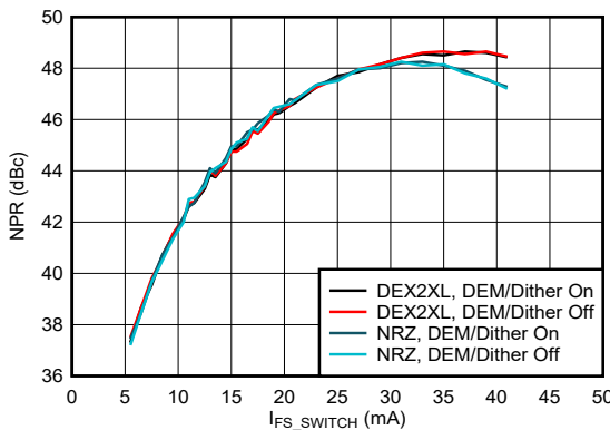
Figure 6-191. Noise Power Ratio vs Output Current: 1 st Nyquist Zone
