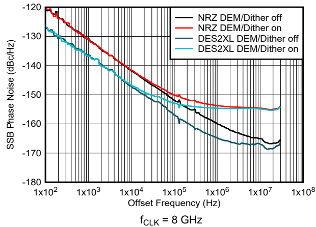
Figure 6-193. Phase Noise vs Offset Frequency at 1 GHz
