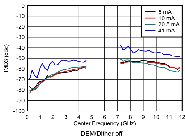
Figure 6-108. IMD3 vs Frequency and Output Current in DES2X Modes
