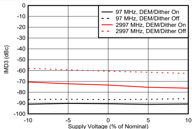
Figure 6-131. IMD3 vs Voltage in DES2XL Mode
