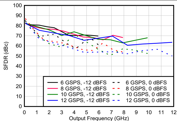
Figure 6-100. SFDR vs Frequency and Digital Amplitude in DES2X Modes
