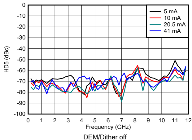
Figure 6-174. HD5 vs Frequency and Output Current in NRZ/RF Modes
