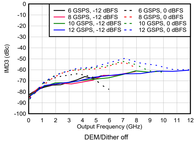
Figure 6-125. IMD3 vs Frequency and Sample Rate in DES2X Modes
