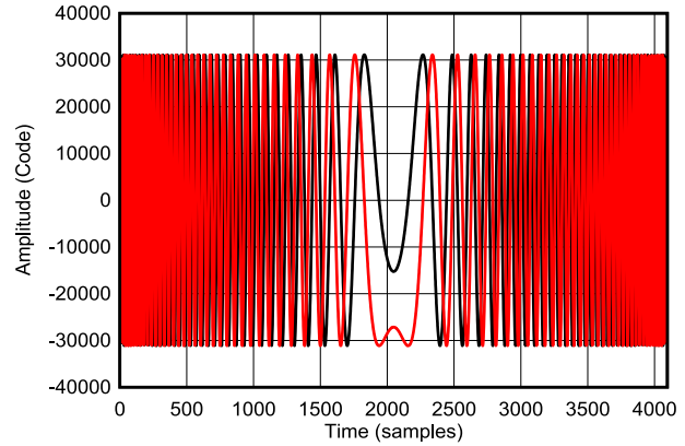
Figure 8-14. Complex Time Domain of NLFM Chirp (Red = real, Black = imag)
