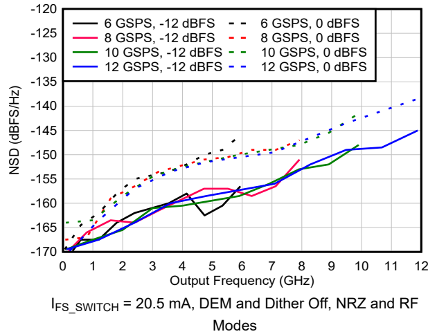
Figure 6-72. NSD vs Output Frequency and Sample Rate
