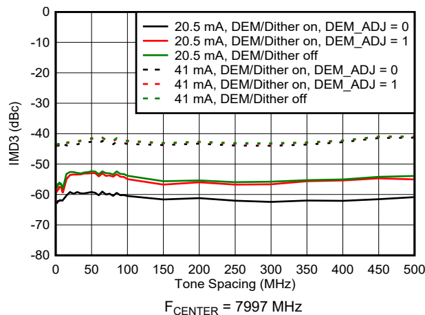
Figure 6-120. IMD3 vs Tone Spacing in RF Mode
