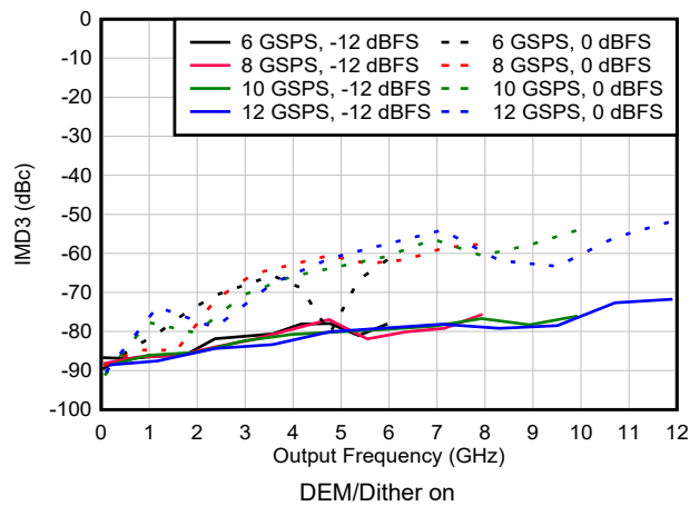
Figure 6-122. IMD3 vs Frequency and Sample Rate in NRZ/RF Modes
