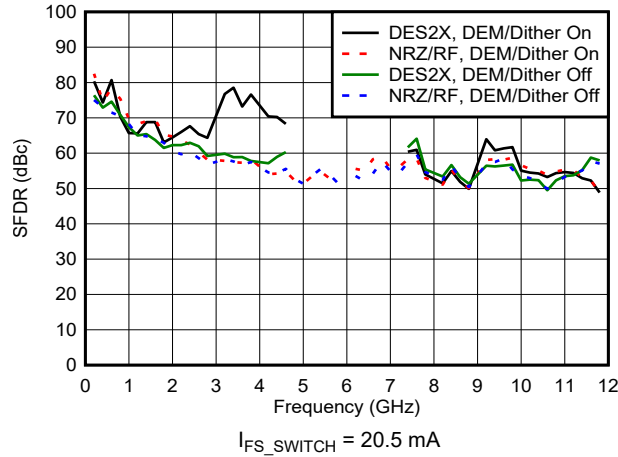
Figure 6-82. SFDR vs Frequency and Mode
