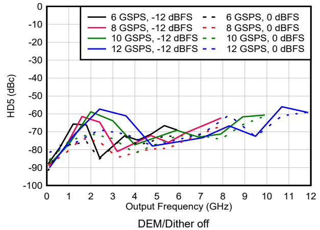
Figure 6-185. HD5 vs Frequency and Sample Rate in DES2X Modes
