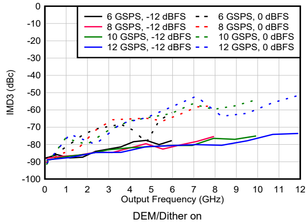
Figure 6-124. IMD3 vs Frequency and Sample Rate in DES2X Modes
