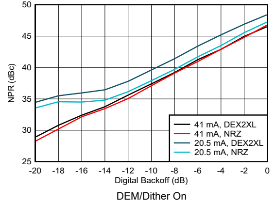
Figure 6-188. Noise Power Ratio vs Digital Backoff: 1 st Nyquist Zone
