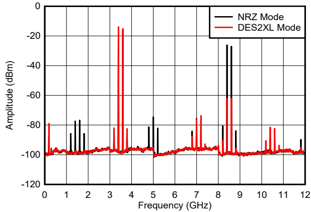
Figure 6-49. Dual Tone, f_{\text{OUT}} = 3497\text{ MHz} , 0 dBFS
