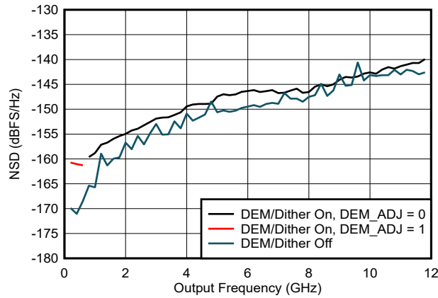
Figure 6-58. NSD vs Output Frequency and DEM/Dither Mode
