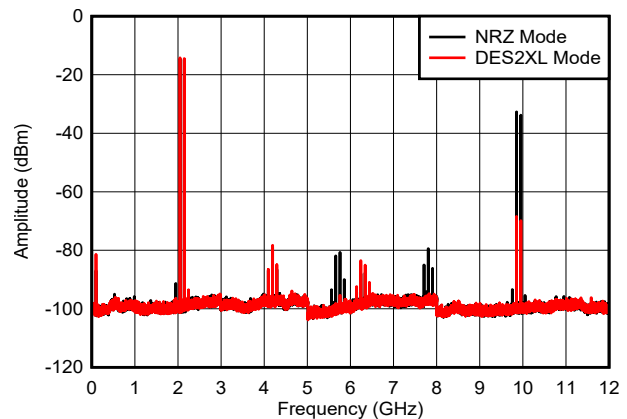
Figure 6-44. Dual Tone, f_{\text{OUT}} = 1097\text{ MHz} , -6 dBFS
