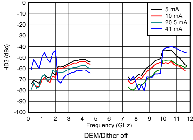
Figure 6-152. HD3 vs Frequency and Output Current in DES2X Modes
