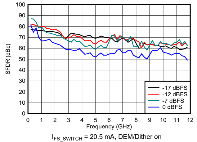
Figure 6-95. SFDR vs Frequency and Digital Amplitude in NRZ/RF Modes
