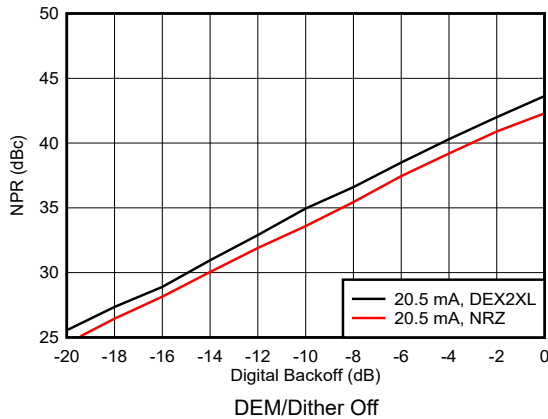
Figure 6-189. Noise Power Ratio vs Digital Backoff: 2 nd Nyquist Zone
