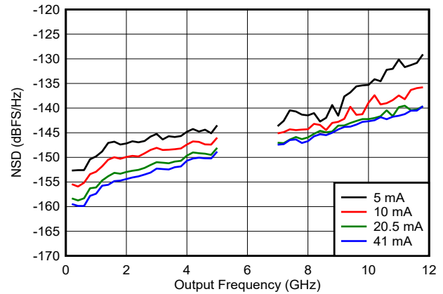
Figure 6-61. NSD vs Output Frequency and Output Current
