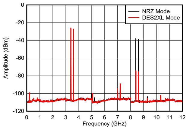
Figure 6-49. Dual Tone, f_{\text{OUT}} = 3497\text{ MHz} , 0 dBFS
