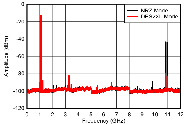
Figure 6-43. Dual Tone, f_{\text{OUT}} = 1097\text{ MHz} , 0 dBFS
