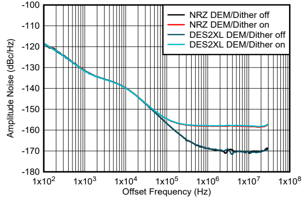
Figure 6-200. Amplitude Noise vs Offset Frequency at 1 GHz
