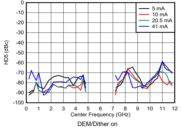
Figure 6-177. HD5 vs Frequency and Output Current in DES2X Modes
