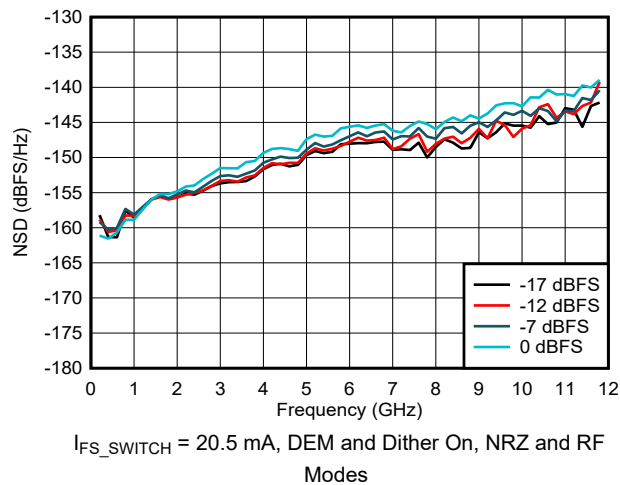
Figure 6-66. NSD vs Output Frequency and Digital Amplitude
