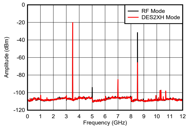
includes PCB, cable and balun loss Figure 6-28. f_{\text{OUT}} = 3497\text{ MHz} , 0 dBFS
