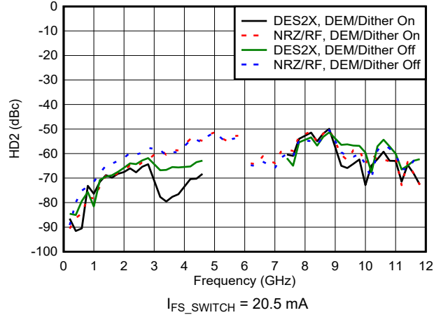
Figure 6-86. HD2 vs Frequency and Mode
