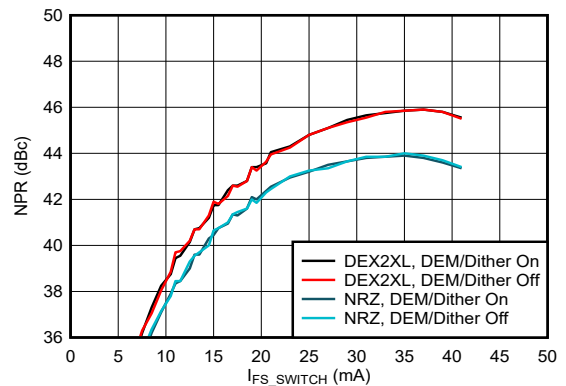
Figure 6-192. Noise Power Ratio vs Output Current: 2 nd Nyquist Zone
