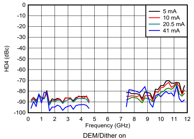
Figure 6-169. HD4 vs Frequency and Output Current in DES2X Modes
