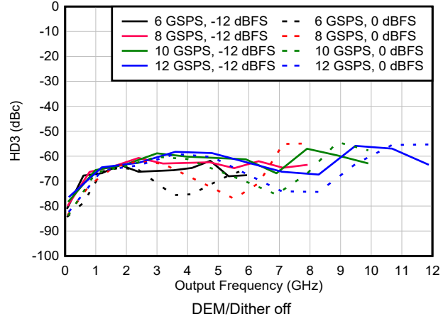
Figure 6-165. HD3 vs Frequency and Sample Rate in DES2X Modes
