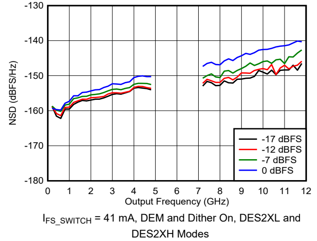
Figure 6-71. NSD vs Output Frequency and Digital Amplitude
