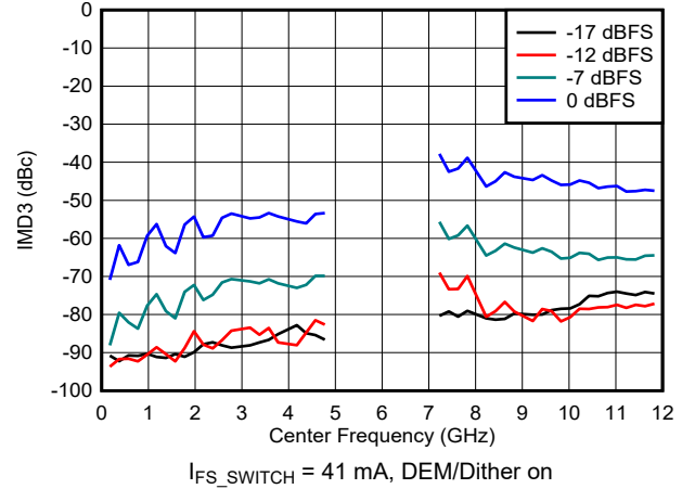
Figure 6-117. IMD3 vs Frequency and Digital Amplitude in DES2X Modes
