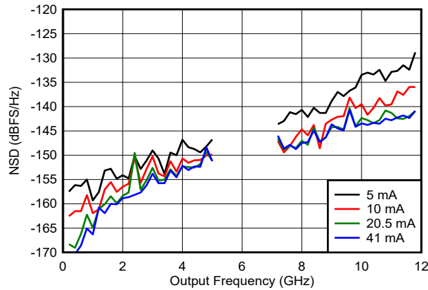
Figure 6-60. NSD vs Output Frequency and Output Current
