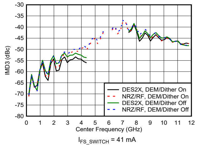
Figure 6-85. IMD3 vs Frequency and Mode
