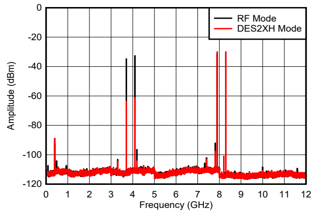
Figure 6-54. Dual Tone, f_{\text{OUT}} = 8097\text{ MHz} , -12 dBFS
