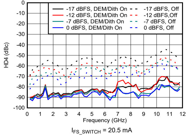
Figure 6-170. HD4 vs Frequency and Digital Amplitude in NRZ/RF Modes
