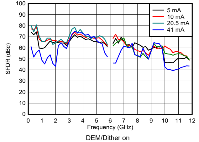
Figure 6-93. SFDR vs Frequency and Output Current in DES2X Modes
