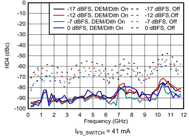
Figure 6-171. HD4 vs Frequency and Digital Amplitude in NRZ/RF Modes
