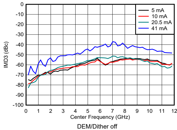
Figure 6-106. IMD3 vs Frequency and Output Current in NRZ/RF Modes
