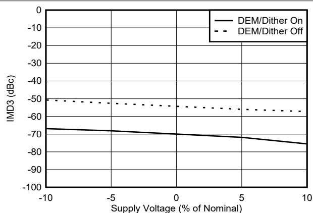
Figure 6-132. IMD3 vs Voltage in RF Mode at 9002 MHz
