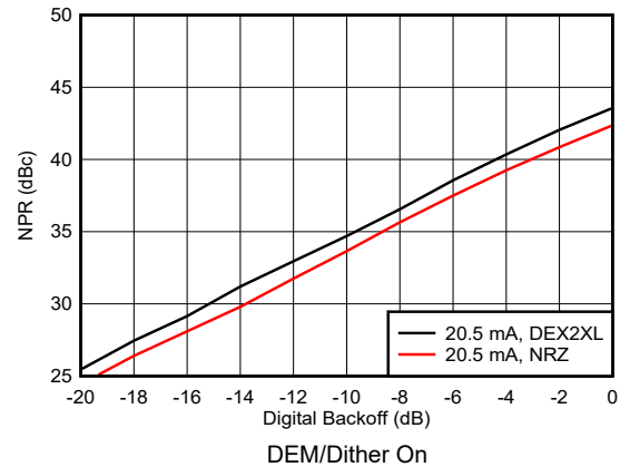
Figure 6-190. Noise Power Ratio vs Digital Backoff: 2 nd Nyquist Zone
