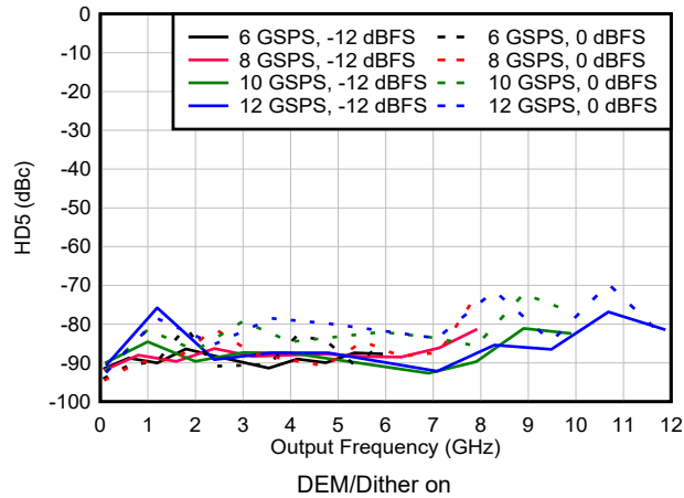
Figure 6-184. HD5 vs Frequency and Sample Rate in DES2X Modes
