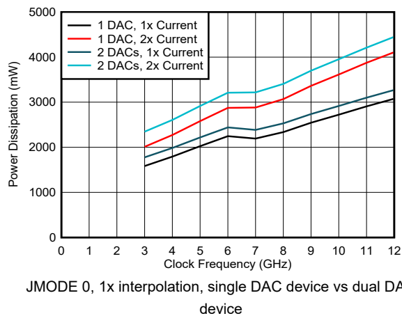
Figure 6-207. Power Dissipation vs Clock Frequency and DAC Mode
