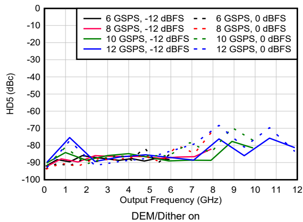
Figure 6-182. HD5 vs Frequency and Sample Rate in NRZ/RF Modes
