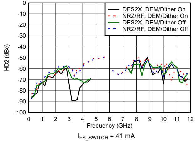
Figure 6-87. HD2 vs Frequency and Mode
