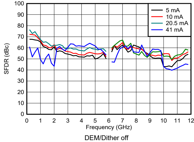
Figure 6-92. SFDR vs Frequency and Output Current in DES2X Modes
