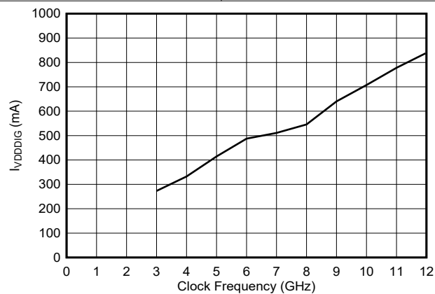
Figure 6-216. VDDDIG Current vs Clock Frequency and Digital Mode
