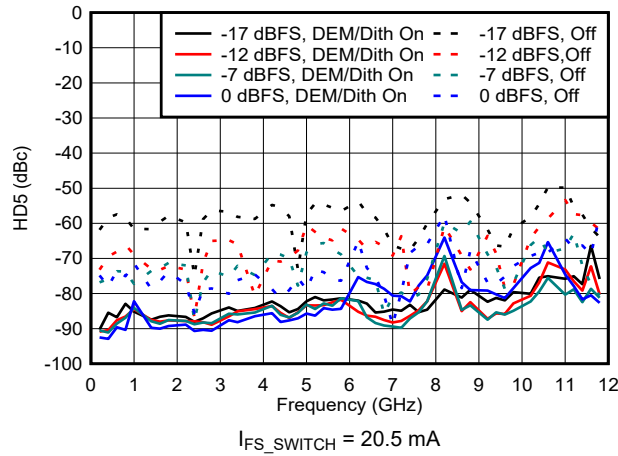
Figure 6-178. HD5 vs Frequency and Digital Amplitude in NRZ/RF Modes
