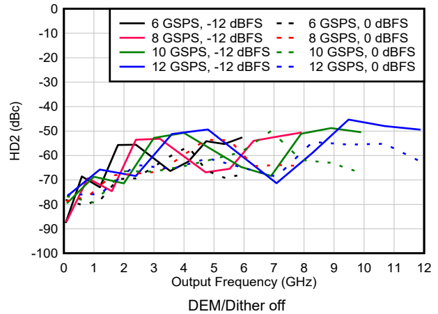
Figure 6-149. HD2 vs Frequency and Sample Rate in DES2X Modes
