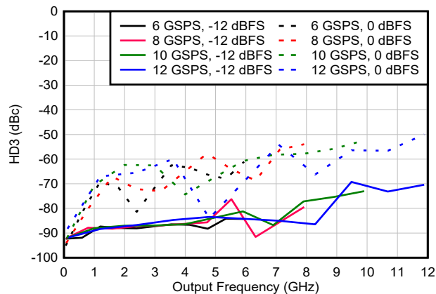
Figure 6-160. HD3 vs Frequency and Digital Amplitude in DES2X Modes
