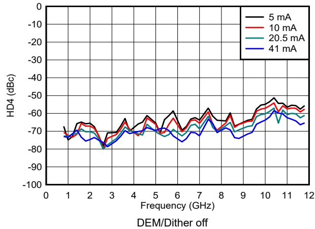
Figure 6-166. HD4 vs Frequency and Output Current in NRZ/RF Modes
