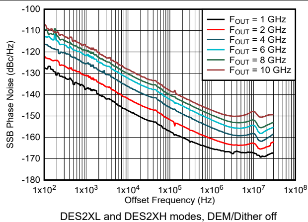
Figure 6-195. Phase Noise vs Offset Frequency and Output Frequency
