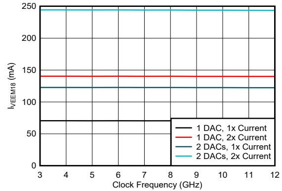
Figure 6-210. VEEM18 Current vs Clock Frequency and DAC Mode
