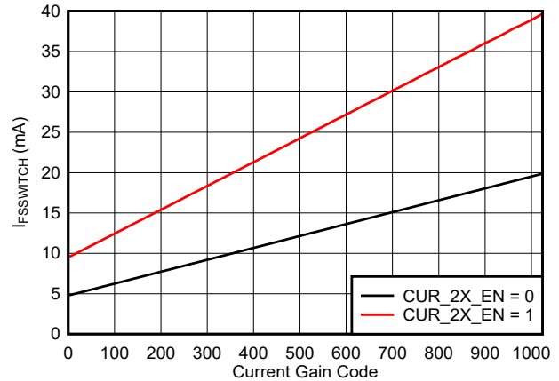
Figure 6-15. I_{\text{FS\_SWITCH}} vs Gain Code
