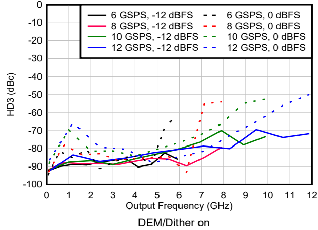
Figure 6-164. HD3 vs Frequency and Sample Rate in DES2X Modes
