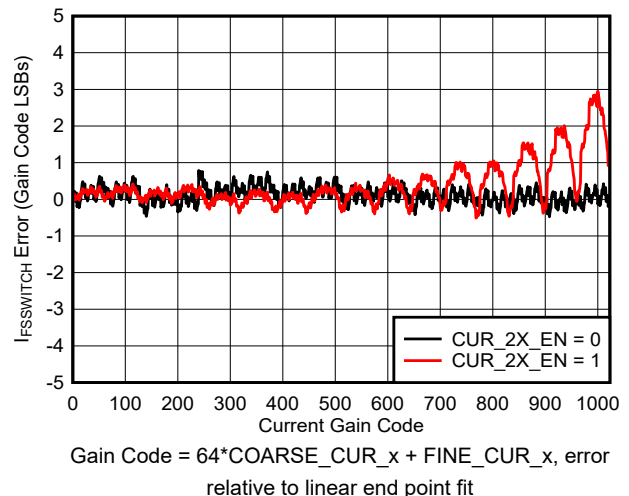
Figure 6-17. I_{\text{FS\_SWITCH}} Error vs Gain Code
