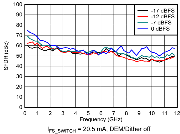
Figure 6-94. SFDR vs Frequency and Digital Amplitude in NRZ/RF Modes
