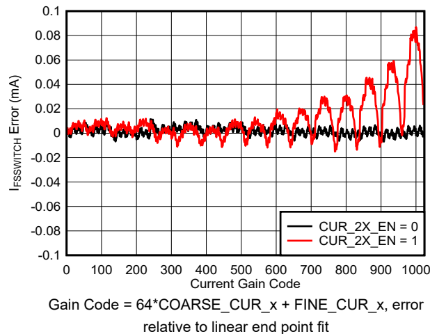
Figure 6-16. I_{\text{FS\_SWITCH}} Error vs Gain Code
