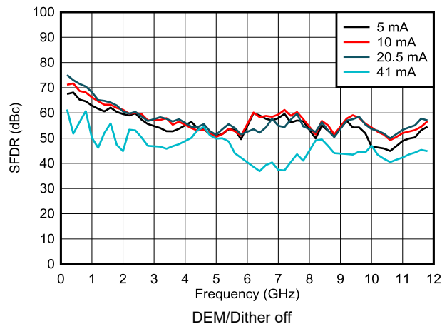
Figure 6-90. SFDR vs Frequency and Output Current in NRZ/RF Modes
