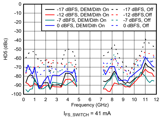
Figure 6-181. HD5 vs Frequency and Digital Amplitude in DES2X Modes
