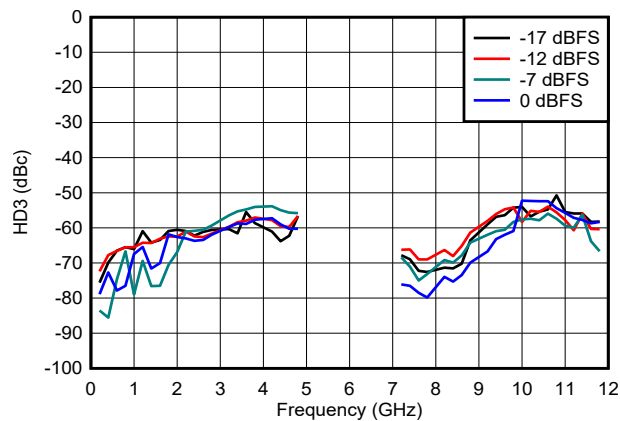
Figure 6-158. HD3 vs Frequency and Digital Amplitude in DES2X Modes
