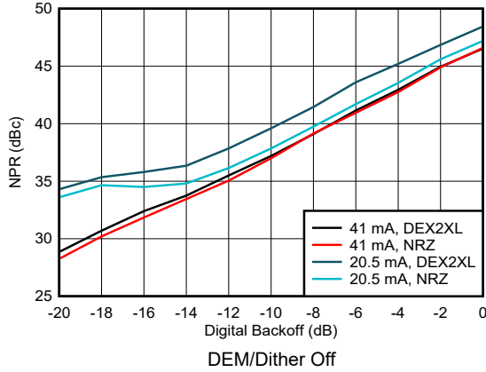
Figure 6-187. Noise Power Ratio vs Digital Backoff: 1 st Nyquist Zone
