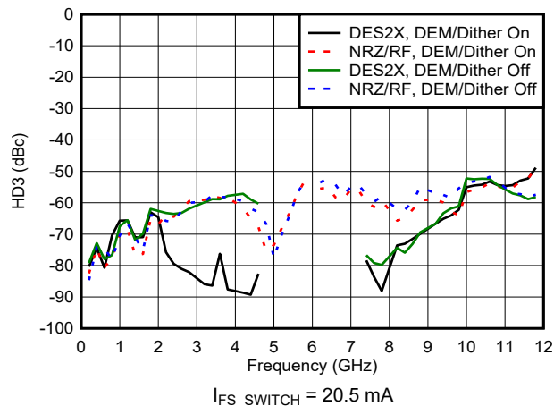
Figure 6-88. HD3 vs Frequency and Mode
