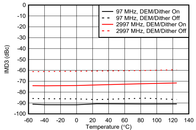
Figure 6-127. IMD3 vs Temperature in DES2XL Mode
