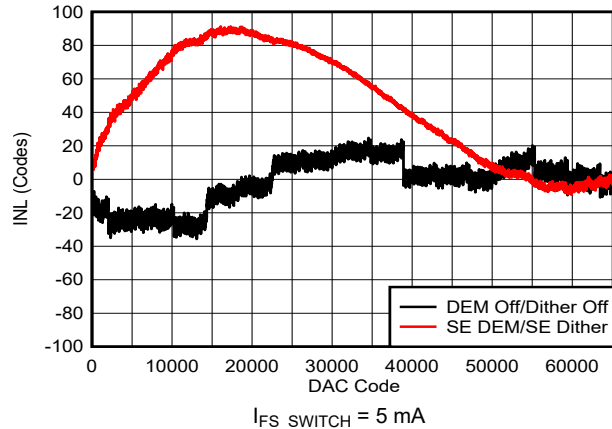
Figure 6-14. INL vs DAC Code: 5 mA
