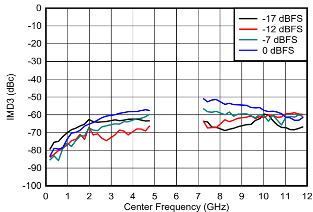
Figure 6-112. IMD3 vs Frequency and Digital Amplitude in NRZ/RF Modes
