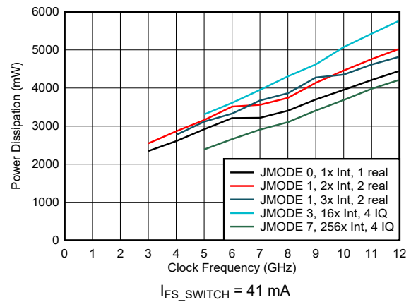
Figure 6-204. Power Dissipation vs Clock Frequency and Digital Mode
