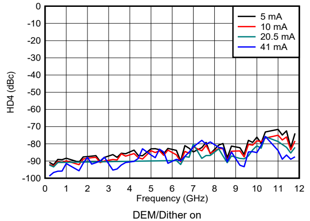
Figure 6-167. HD4 vs Frequency and Output Current in NRZ/RF Modes
