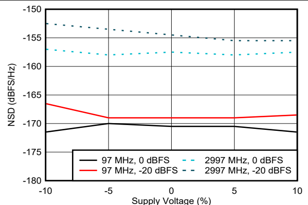
Figure 6-79. NSD vs Supply Voltage
