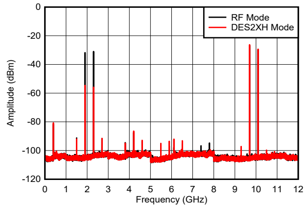
Figure 6-56. Dual Tone, f_{\text{OUT}} = 9897\text{ MHz} , -6 dBFS
