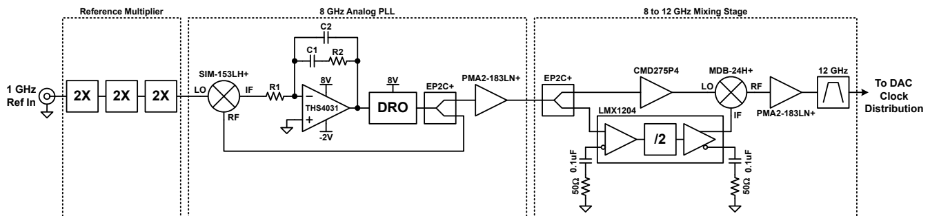
Figure 8-11. 12 GHz Clock Synthesizer
