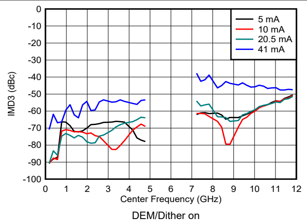
Figure 6-109. IMD3 vs Frequency and Output Current in DES2X Modes
