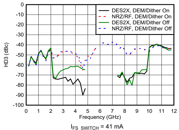
Figure 6-89. HD3 vs Frequency and Mode
