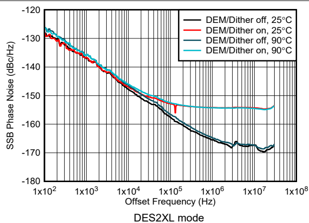
Figure 6-197. Phase Noise vs Offset Frequency at 1 GHz
