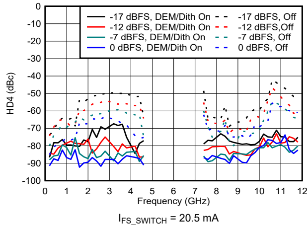
Figure 6-172. HD4 vs Frequency and Digital Amplitude in NRZ/RF Modes
