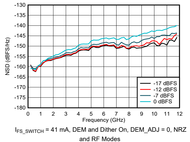
Figure 6-67. NSD vs Output Frequency and Digital Amplitude
