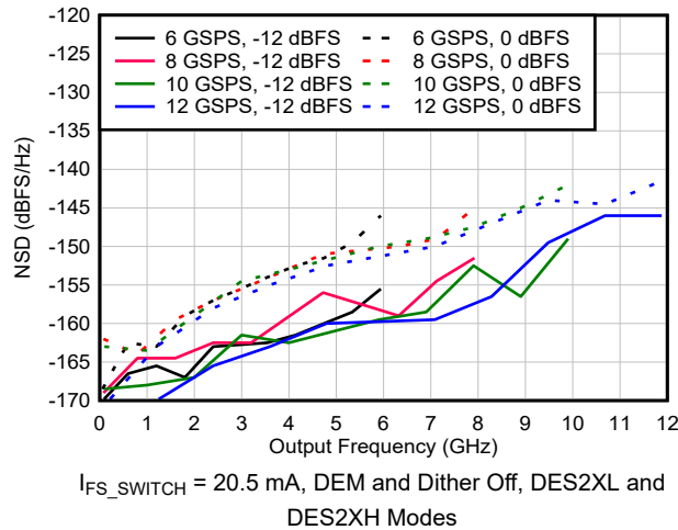
Figure 6-74. NSD vs Output Frequency and Sample Rate
