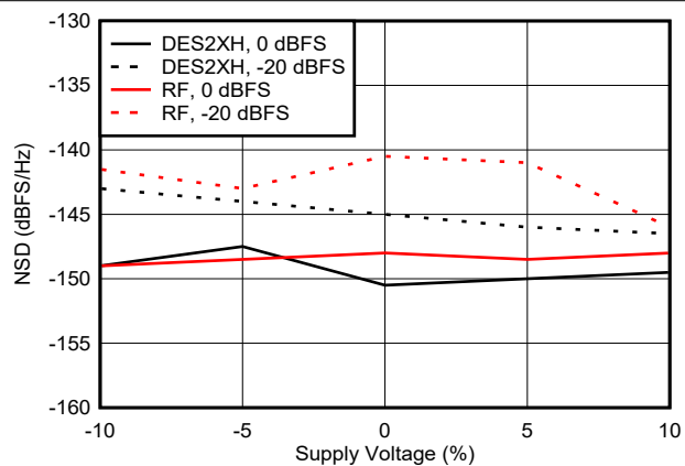
Figure 6-80. NSD vs Supply Voltage
