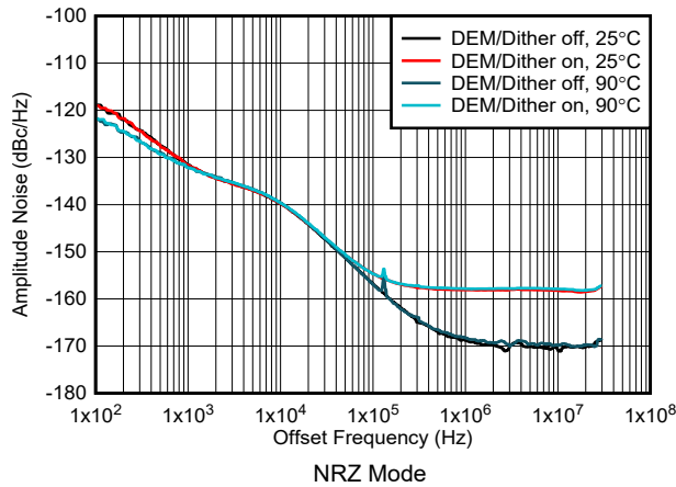
Figure 6-201. Amplitude Noise vs Offset Frequency and Temperature at 1 GHz
