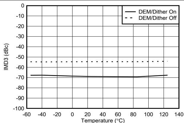
Figure 6-129. IMD3 vs Temperature in DES2XH Mode at 9002 MHz
