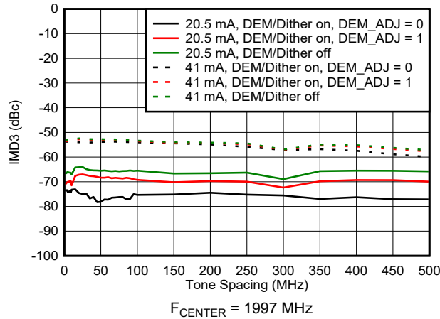
Figure 6-118. IMD3 vs Tone Spacing in NRZ Mode
