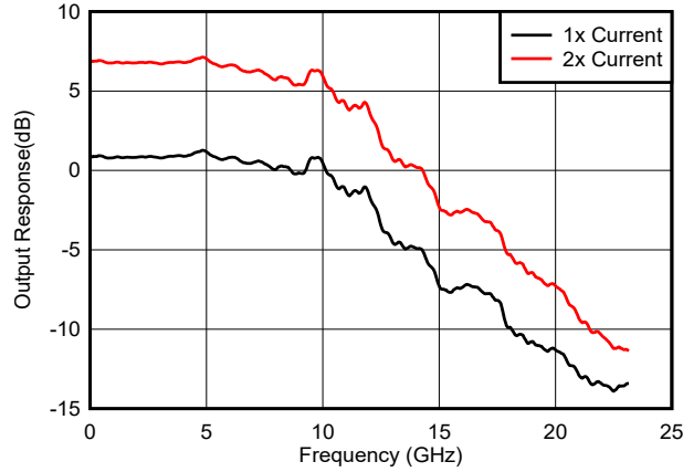
Figure 6-8. Output Response vs Frequency
