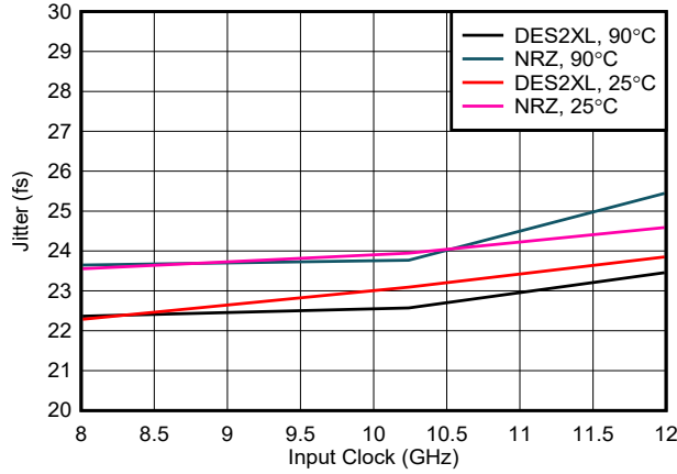
Figure 6-199. Jitter vs Input Clock
