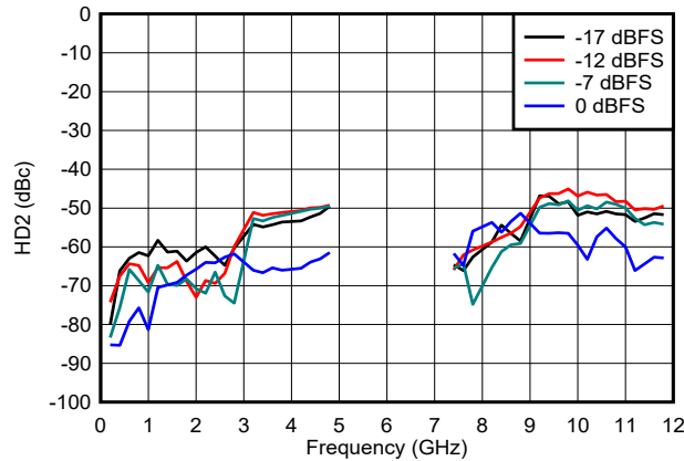
Figure 6-140. HD2 vs Frequency and Digital Amplitude in NRZ/RF Modes
