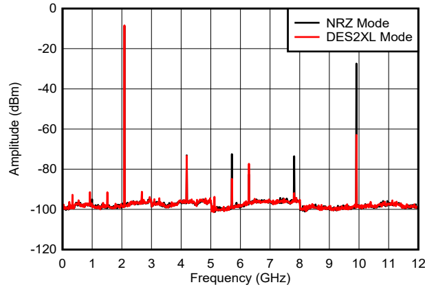
includes PCB, cable and balun loss Figure 6-25. f_{\text{OUT}} = 2097\text{ MHz} , 0 dBFS
