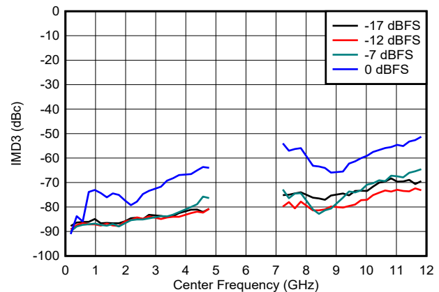
Figure 6-113. IMD3 vs Frequency and Digital Amplitude in NRZ/RF Modes
