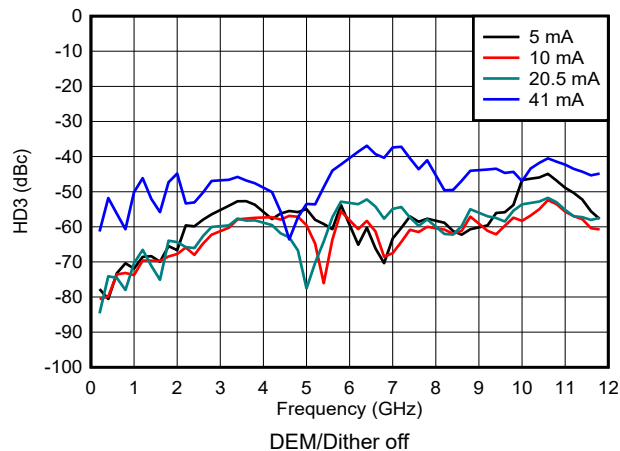
Figure 6-150. HD3 vs Frequency and Output Current in NRZ/RF Modes
