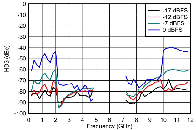
Figure 6-159. HD3 vs Frequency and Digital Amplitude in DES2X Modes
