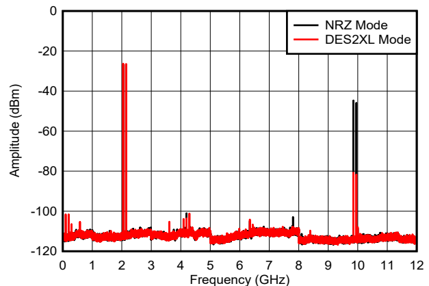
Figure 6-46. Dual Tone, f_{\text{OUT}} = 2097\text{ MHz} , 0 dBFS
