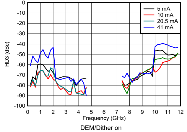
Figure 6-153. HD3 vs Frequency and Output Current in DES2X Modes
