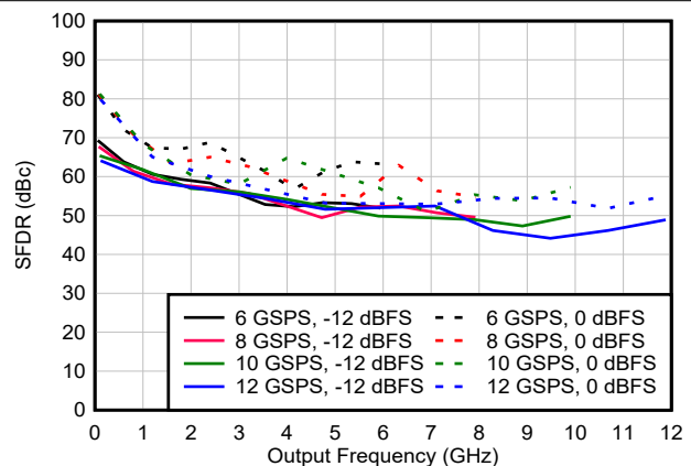
Figure 6-101. SFDR vs Frequency and Digital Amplitude in DES2X Modes
