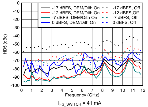
Figure 6-179. HD5 vs Frequency and Digital Amplitude in NRZ/RF Modes
