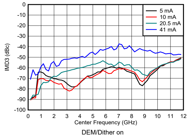
Figure 6-107. IMD3 vs Frequency and Output Current in NRZ/RF Modes
