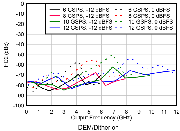
Figure 6-148. HD2 vs Frequency and Sample Rate in DES2X Modes
