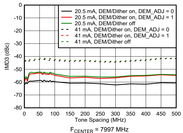
Figure 6-121. IMD3 vs Tone Spacing in DES2XH Mode
