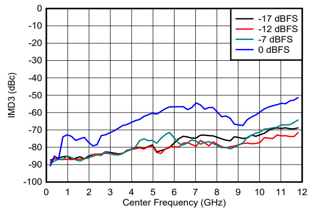
Figure 6-111. IMD3 vs Frequency and Digital Amplitude in NRZ/RF Modes
