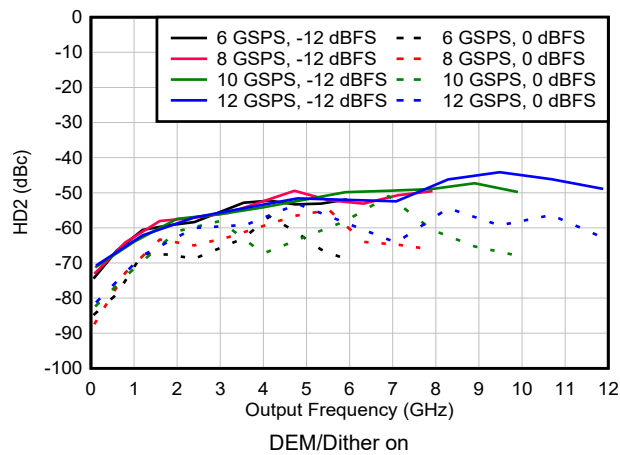
Figure 6-146. HD2 vs Frequency and Sample Rate in NRZ/RF Modes
