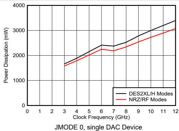
Figure 6-205. Power Dissipation vs Clock Frequency and DAC Mode
