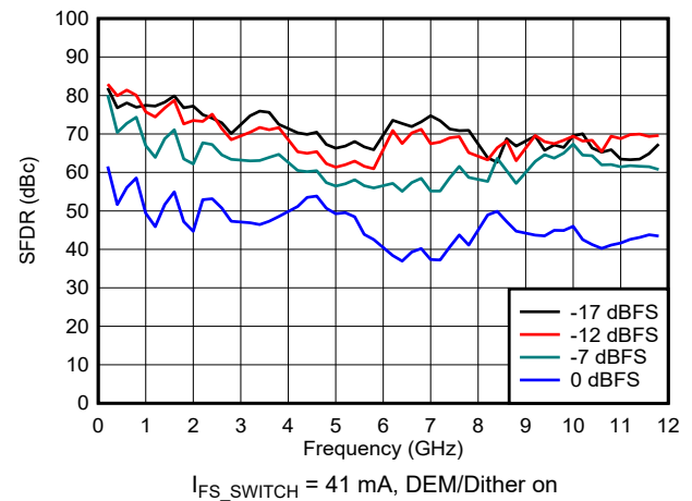
Figure 6-97. SFDR vs Frequency and Digital Amplitude in NRZ/RF Modes
