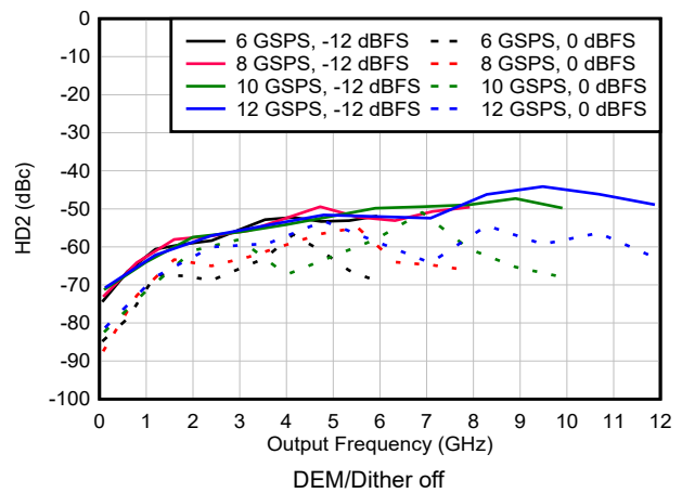
Figure 6-147. HD2 vs Frequency and Sample Rate in NRZ/RF Modes
