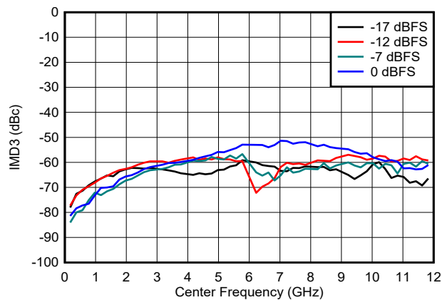
Figure 6-110. IMD3 vs Frequency and Digital Amplitude in NRZ/RF Modes
