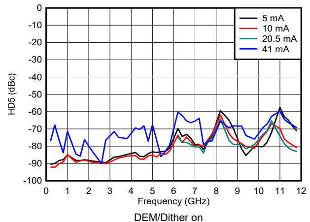
Figure 6-175. HD5 vs Frequency and Output Current in NRZ/RF Modes
