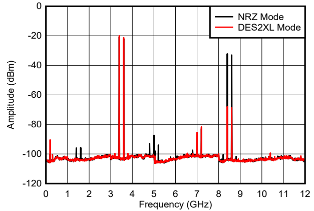
Figure 6-50. Dual Tone, f_{\text{OUT}} = 3497\text{ MHz} , -6 dBFS
