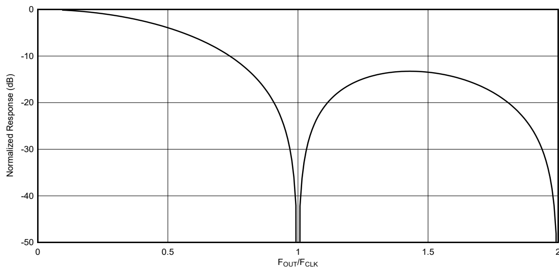
Figure 7-4. NRZ Mode Output Frequency Response
