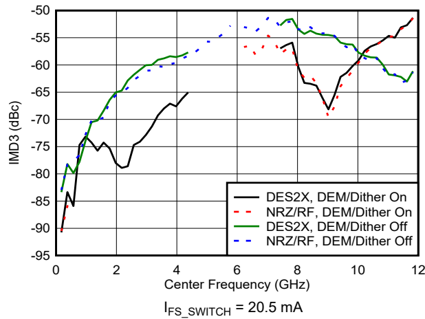
Figure 6-84. IMD3 vs Frequency and Mode
