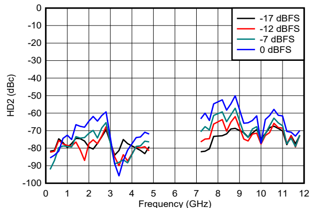
Figure 6-143. HD2 vs Frequency and Digital Amplitude in DES2X Modes
