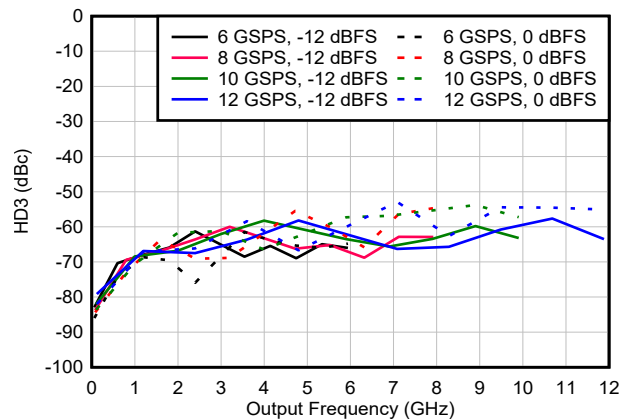
Figure 6-161. HD3 vs Frequency and Digital Amplitude in DES2X Modes
