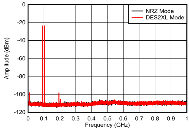
Figure 6-40. Dual Tone, f_{\text{OUT}} = 97\text{ MHz} , -6 dBFS (0 - 1 GHz)
