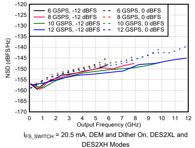
Figure 6-75. NSD vs Output Frequency and Sample Rate
