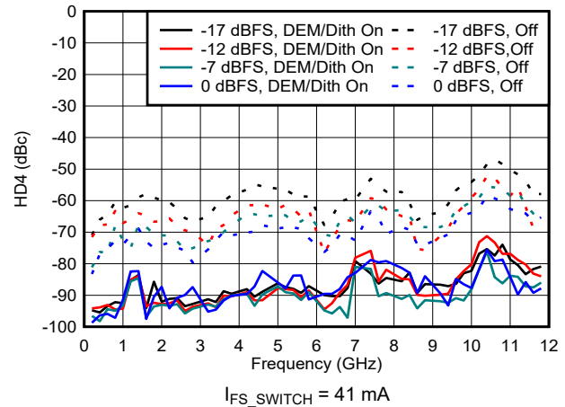
Figure 6-173. HD4 vs Frequency and Digital Amplitude in NRZ/RF Modes
