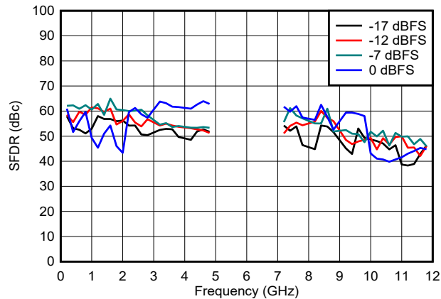
Figure 6-98. SFDR vs Frequency and Digital Amplitude in DES2X Modes
