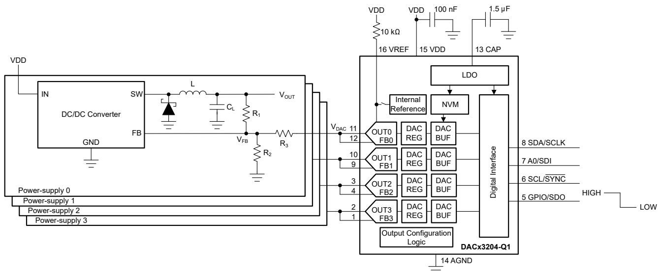
Figure 8-1. APD Biasing
