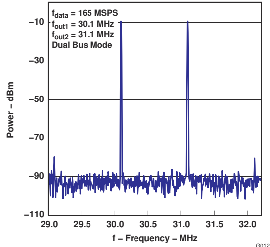
Figure 6-12. Two-Tone Spectrum
