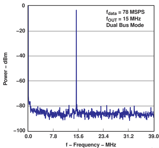
Figure 6-7. Single-Tone Spectrum
