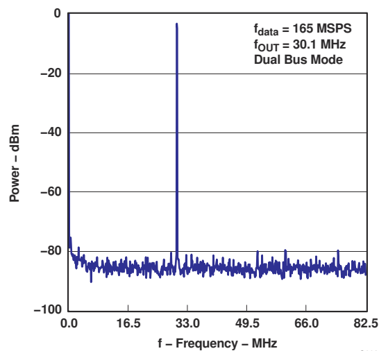
Figure 6-8. Single-Tone Spectrum
