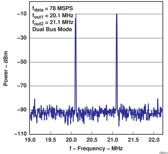
Figure 6-11. Two-Tone Spectrum
