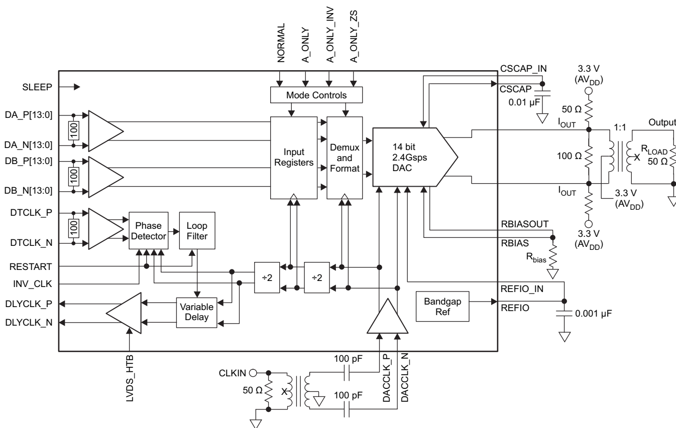
Figure 26. Current Steering DAC5670
