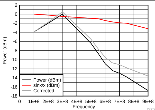
Figure 28. DAC5670 Bandwidth 2 GSPS
