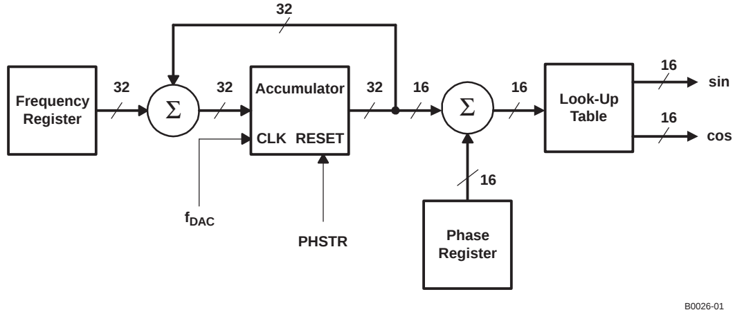
Figure 40. Block Diagram of the NCO
