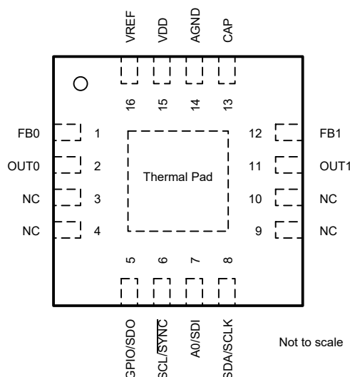
Figure 5-1. RTE (16-pin WQFN) Package, Top View
