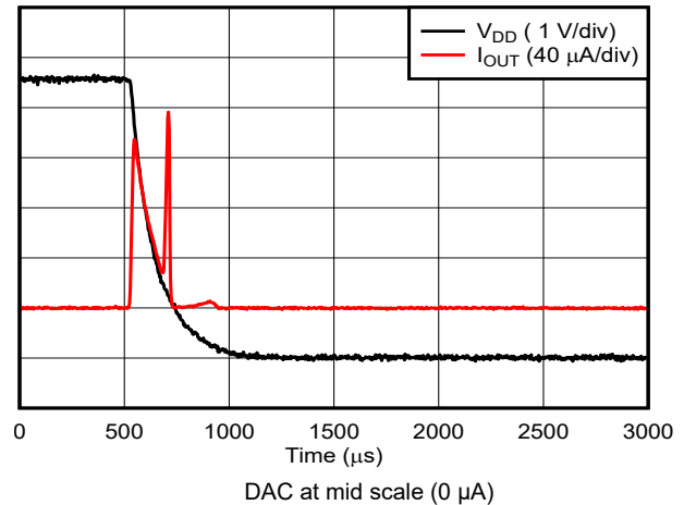
Figure 6-45. Current Output Power-Off Glitch
