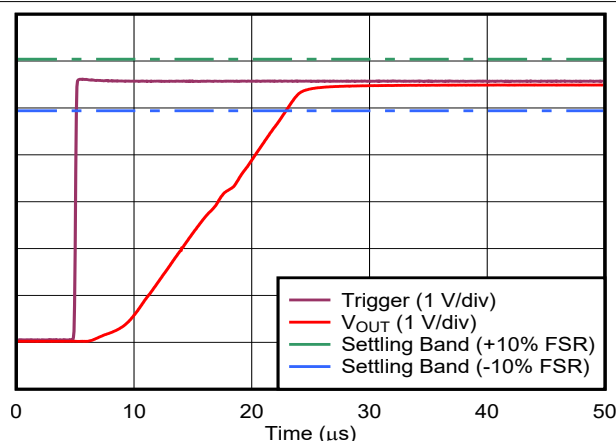
Zero scale to full scale swing
