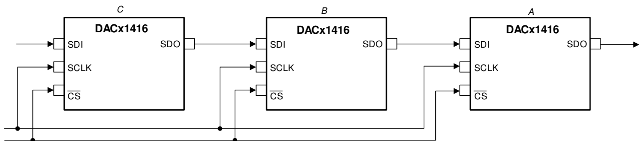
Figure 6-5. Daisy-Chain Layout
