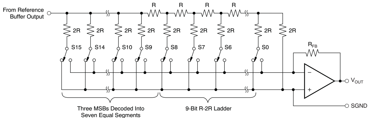
Figure 41. DAC7716 Architecture
