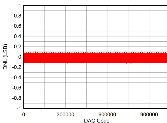
Figure 58. DNL at \pm 10 -V Output
