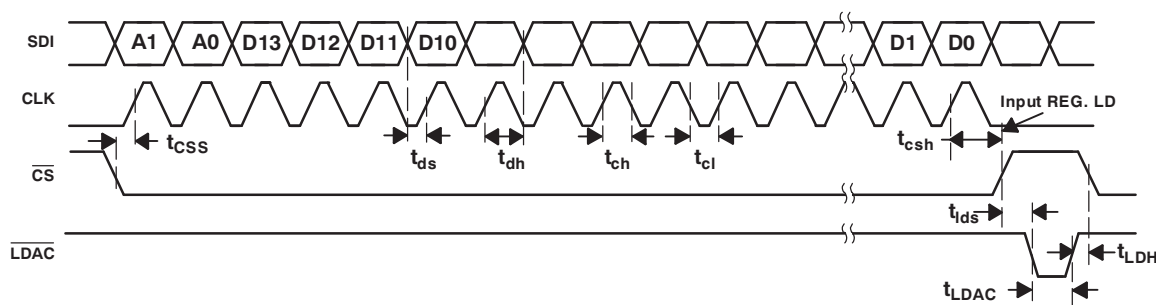
Figure 1. DAC8802 Timing Diagram
