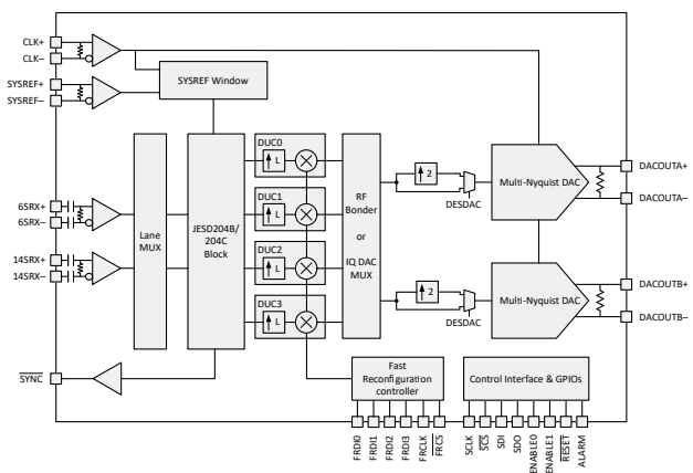
Block Diagram (Dual Channel Devices)
