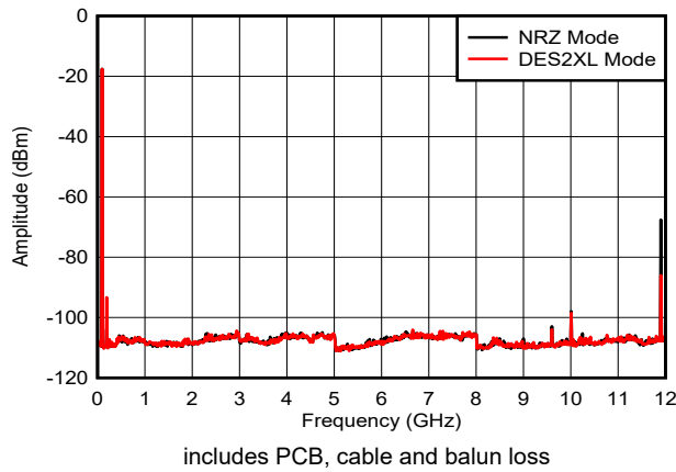
Figure 6-10. f_{\text{OUT}} = 97\text{MHz} , -12dBFS
