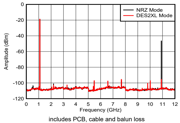
Figure 6-13. f_{\text{OUT}} = 1097\text{MHz} , -12dBFS
