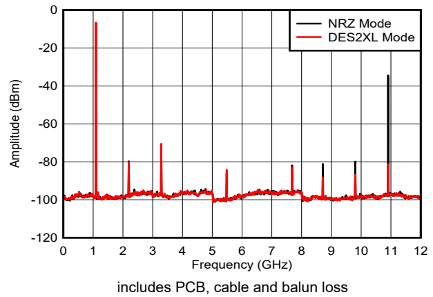
Figure 6-11. f_{\text{OUT}} = 1097\text{MHz} , 0dBFS
