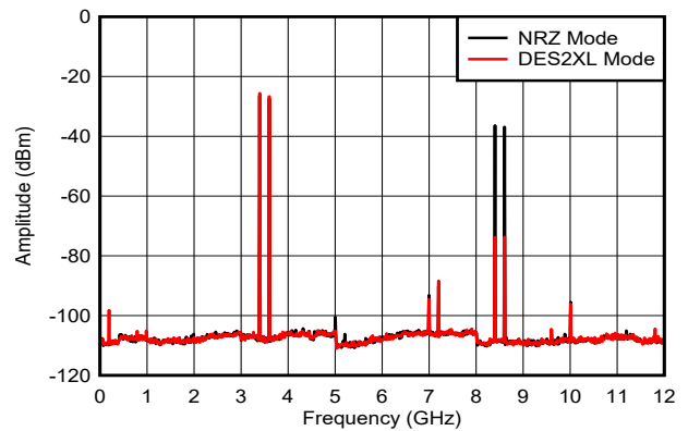
Figure 6-35. Dual Tone, f_{\text{OUT}} = 3497\text{MHz} , 0dBFS
