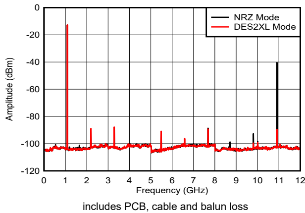
Figure 6-12. f_{\text{OUT}} = 1097\text{MHz} , -6dBFS
