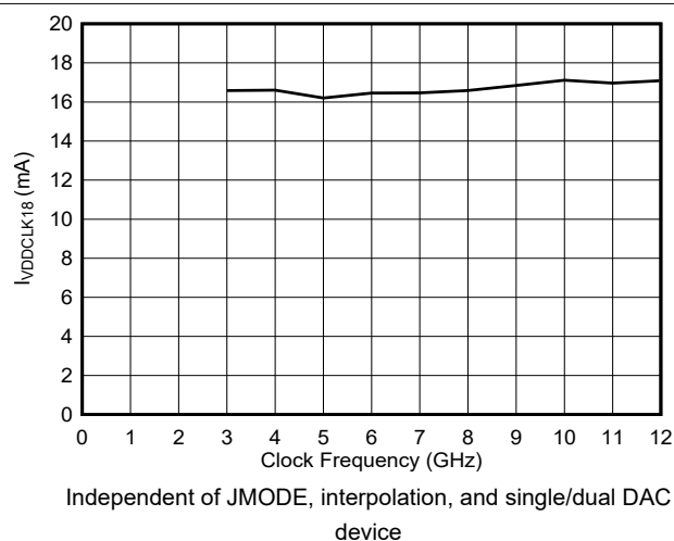
Figure 6-49. VDDCLK18 Current vs Clock Frequency
