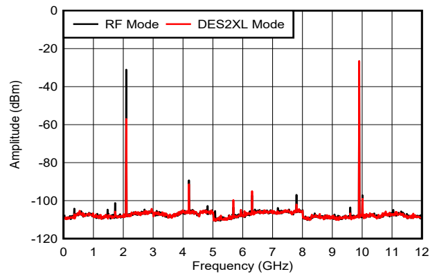
Figure 6-23. f_{\text{OUT}} = 9897\text{MHz} , 0dBFS
