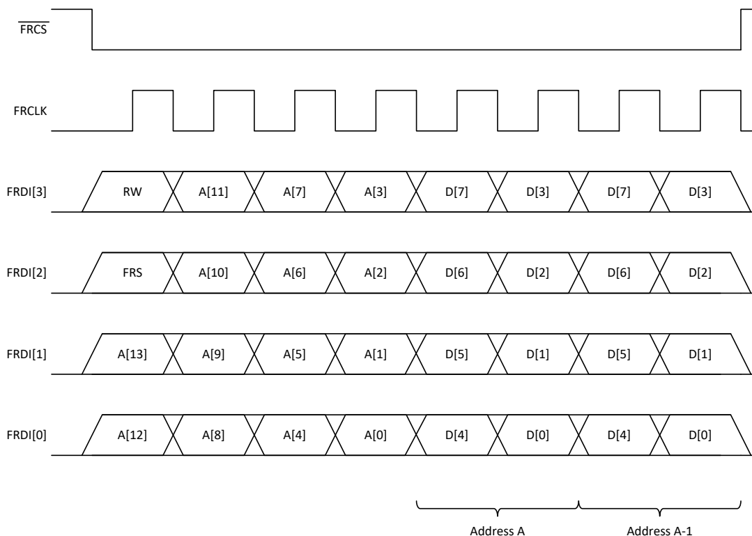
Figure 7-60. FR Interface Timing Diagram
