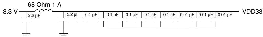
Figure 10-4. VDD33 Recommended Filter
