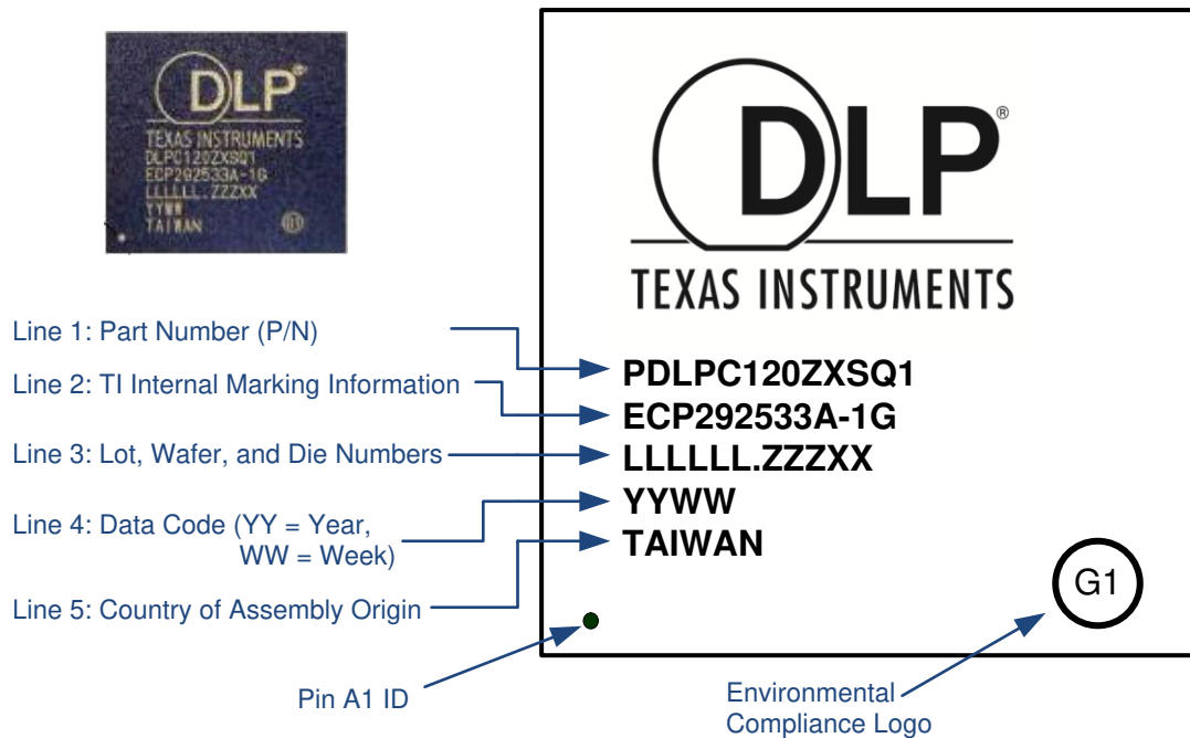
Figure 12-1. Device Marking
