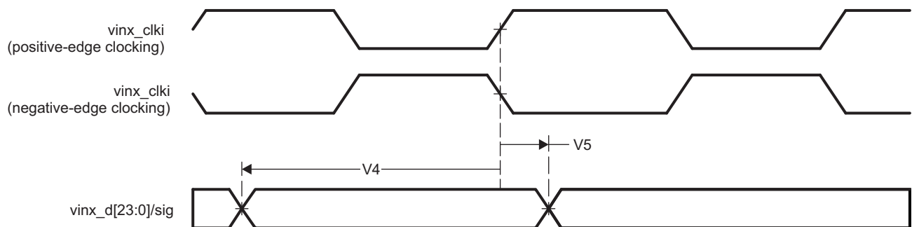
Figure 5-19. Video Input Ports Clock Signal
