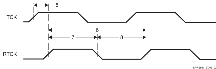
Figure 5-63. JTAG With RTCK Timing
