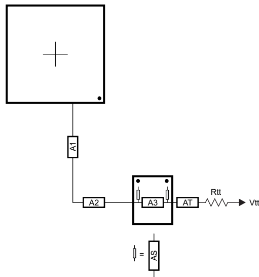
Figure 7-60. ADDR_CTRL Routing for Two Mirrored DDR3 Devices
