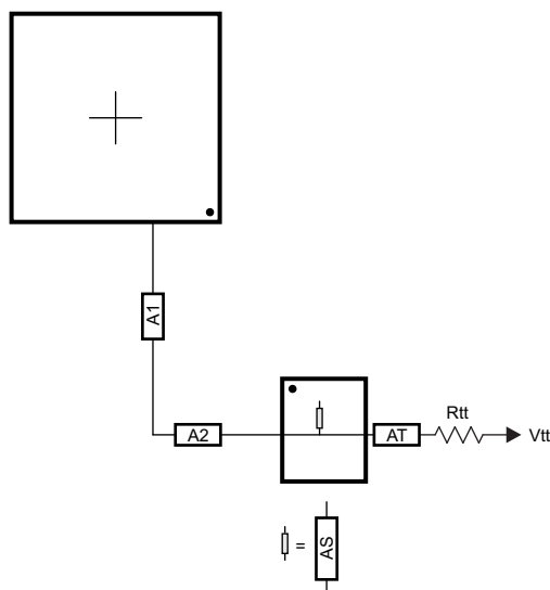
Figure 7-63. CK Routing for One DDR3 Device
