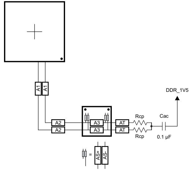
Figure 7-59. CK Routing for Two Mirrored DDR3 Devices
