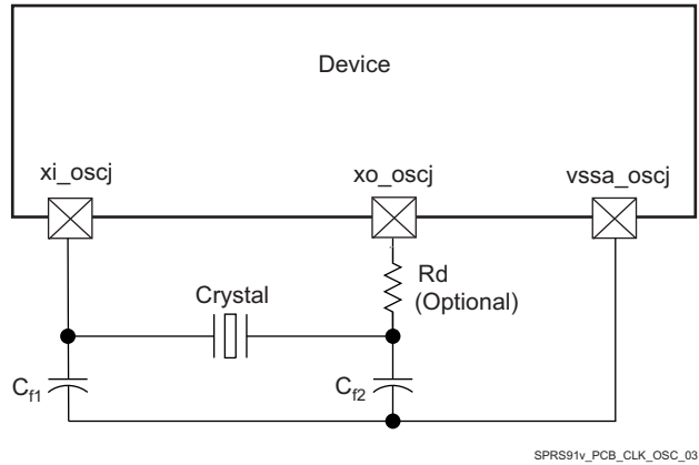
Figure 7-22. Grounding Scheme for High-Frequency Clock
