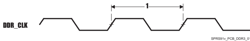
Figure 7-45. DDR3 Memory Controller Clock Timing
