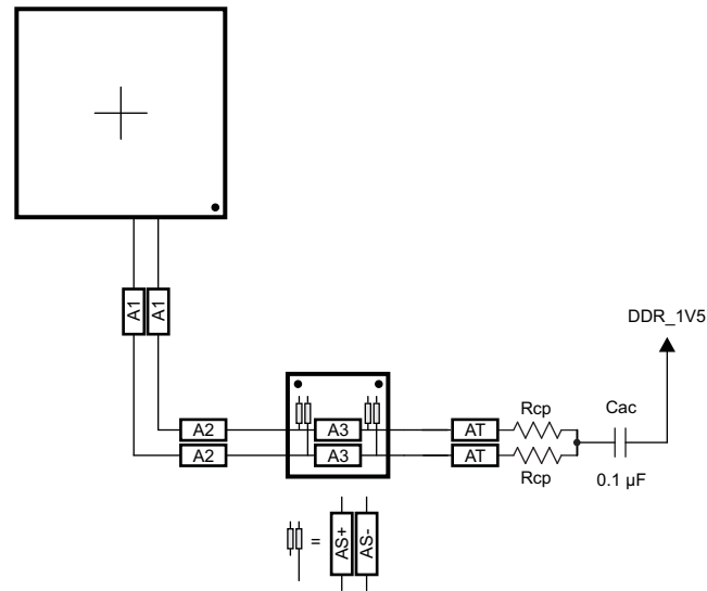
Figure 7-53. CK Routing for Two Mirrored DDR3 Devices
