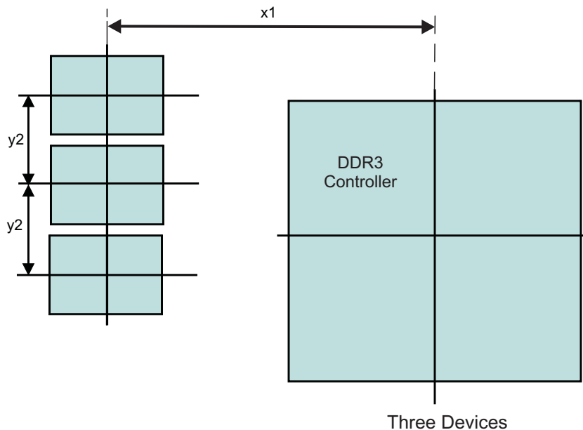
Figure 7-47. Placement Specifications
