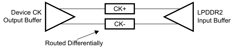
Figure 7-32. CK Signals Topology
