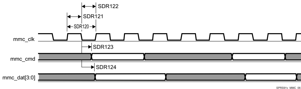
Figure 5-59. MMC/SD/SDIOj in - SDR12 - Transmitter Mode
