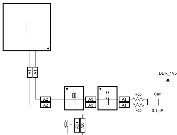
Figure 7-57. CK Routing for Two Single-Side DDR3 Devices
