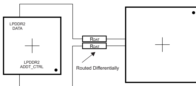
Figure 7-28. DQ[x] Topology
