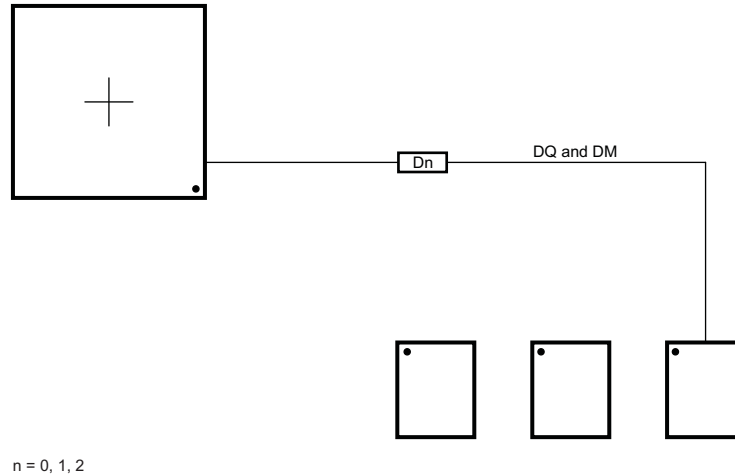
Figure 7-68. DQ/DM Routing With Any Number of Allowed DDR3 Devices
