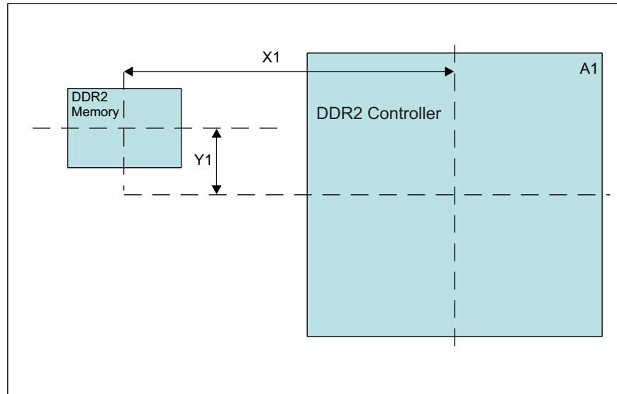
Figure 7-40. Device and DDR2 Device Placement
