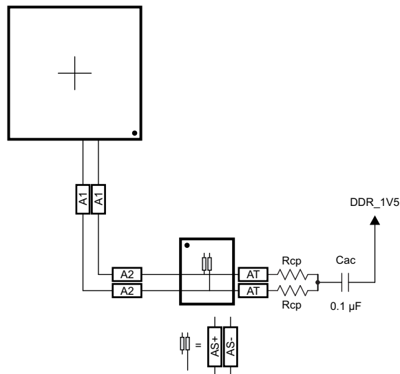
Figure 7-63. CK Routing for One DDR3 Device
