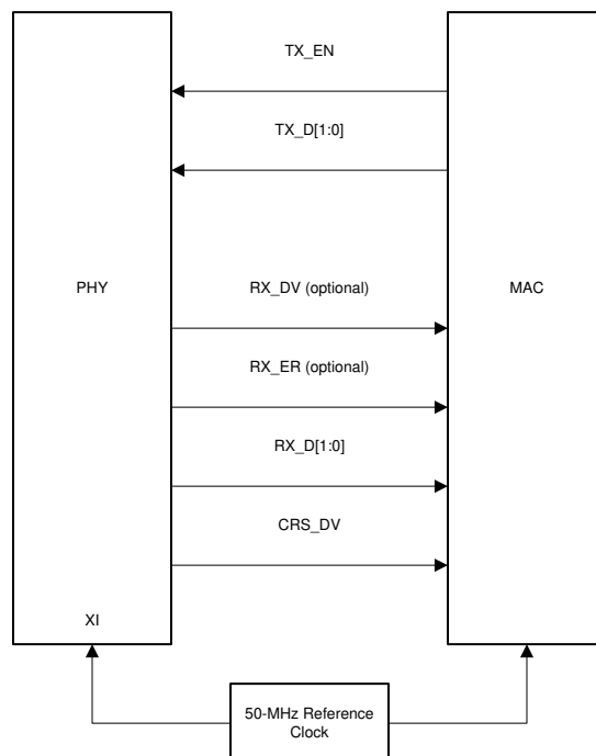
Figure 8-3. RMII Follower Signaling with an External 50MHz CMOS-level Oscillator
