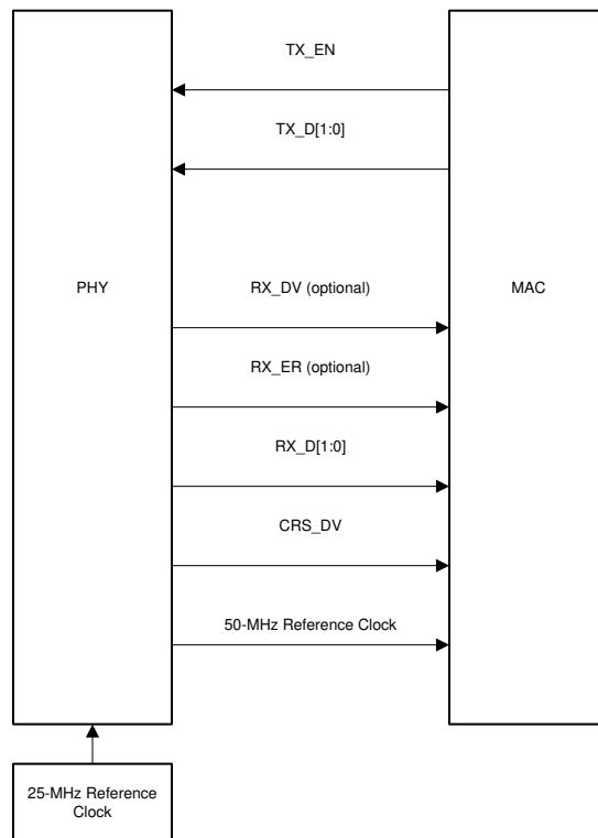
Figure 8-5. RMII Leader Signaling
