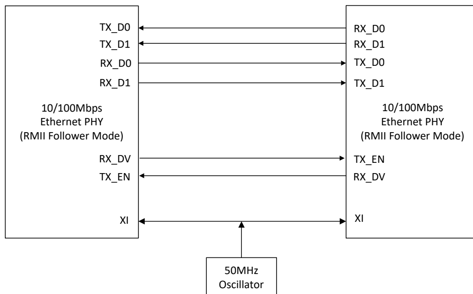
Figure 8-7. RMII Repeater Mode: Follower-Follower
