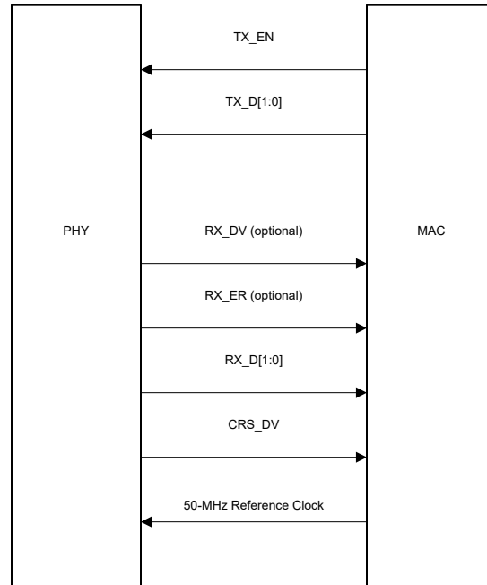
Figure 8-4. RMII Follower Signaling with 50MHz Clocking from MAC
