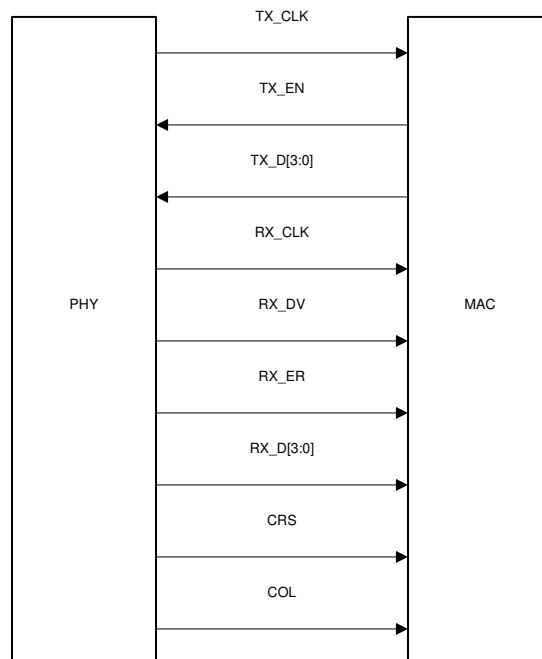
Figure 8-2. MII Signaling
