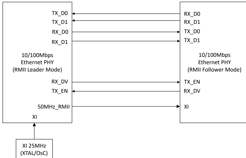
Figure 8-6. RMII Repeater Mode: Leader-Follower
