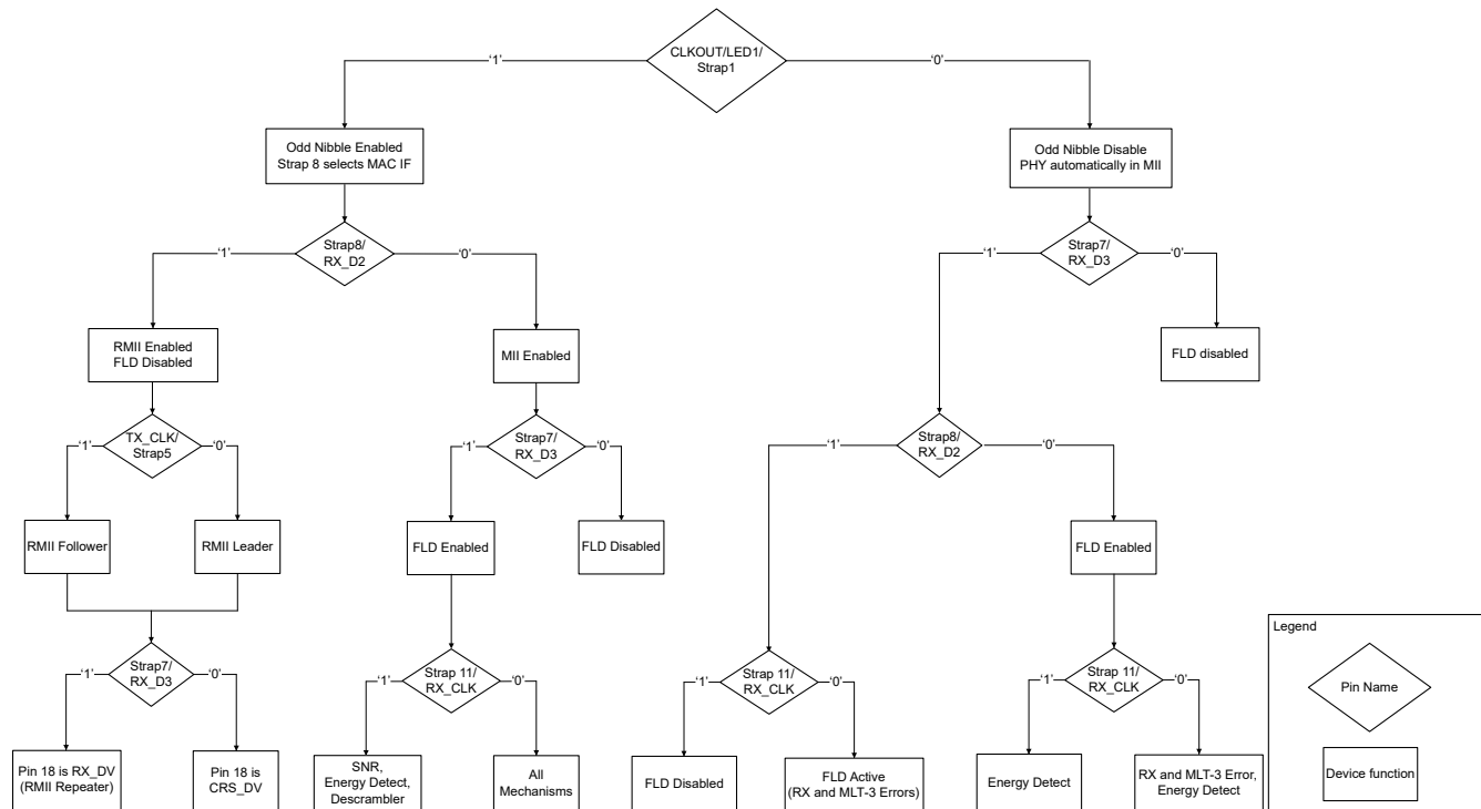
Figure 8-13. Enhanced Bootstrap Flowchart
