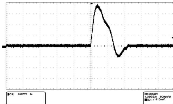
Figure 7-14. 10BASE-Tc Link Pulse Waveform
