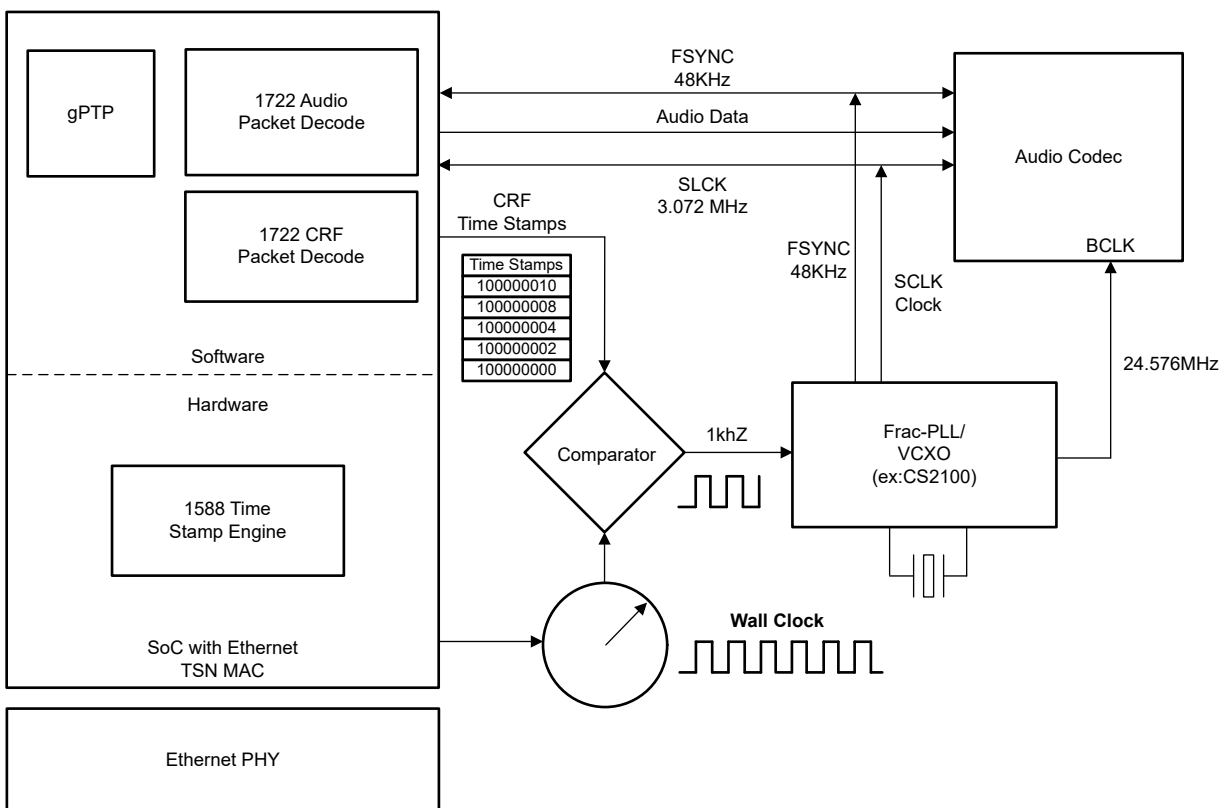
Figure 5-2. Typical Audio Over Ethernet Architecture
