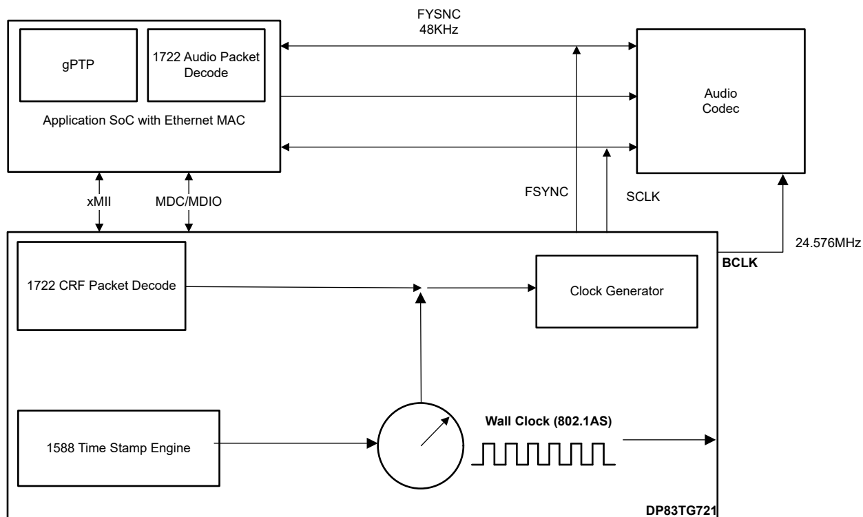
Figure 5-3. Audio Over Ethernet Architecture with DP83TG721-Q1
