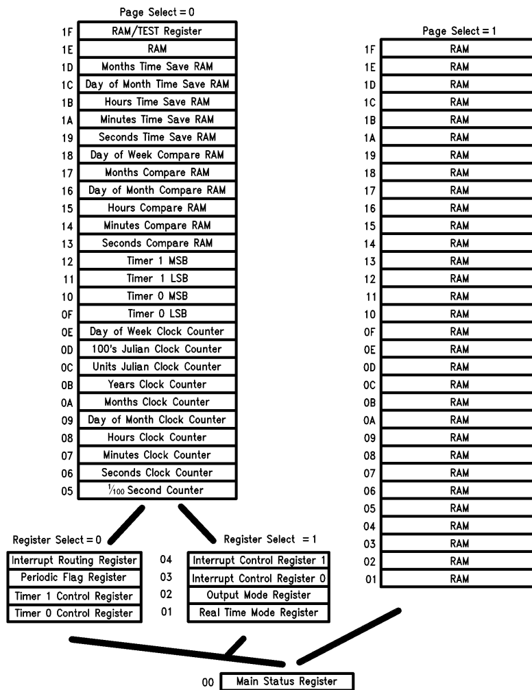
FIGURE 2. DP8570A Internal Memory Map
