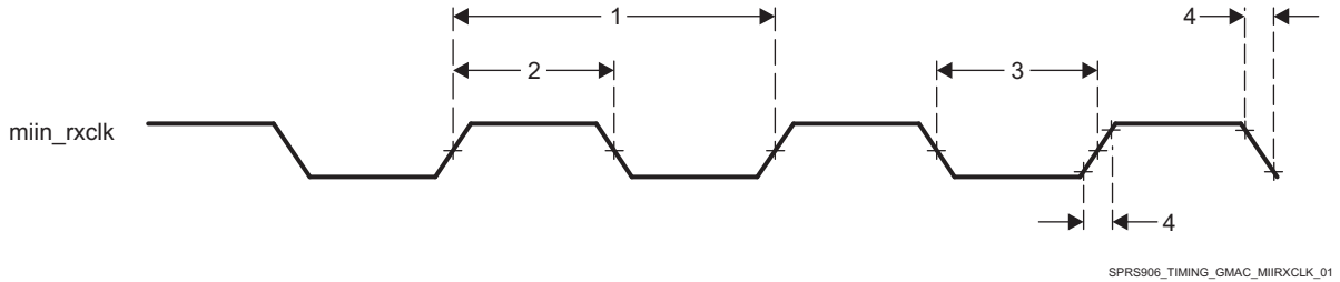
Figure 5-68. Clock Timing (GMAC Receive) - MII operation
