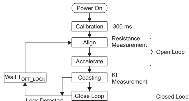
Figure 7. DRV10963 Initialization and Motor Start-up Sequence
