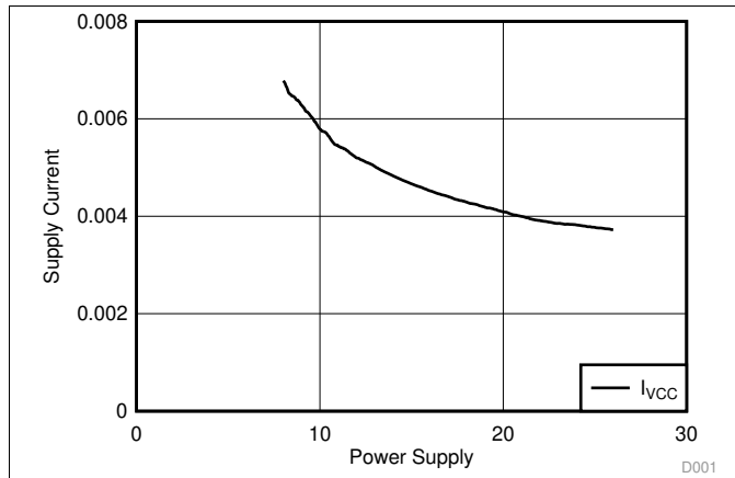
Figure 1. Supply Current vs Power Supply
