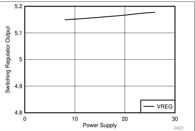
Figure 2. Step-down Regulator Output vs Power Supply (VregSel = 0)
