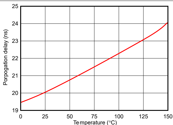
Figure 6-12. HI/LI Propagation Delay
