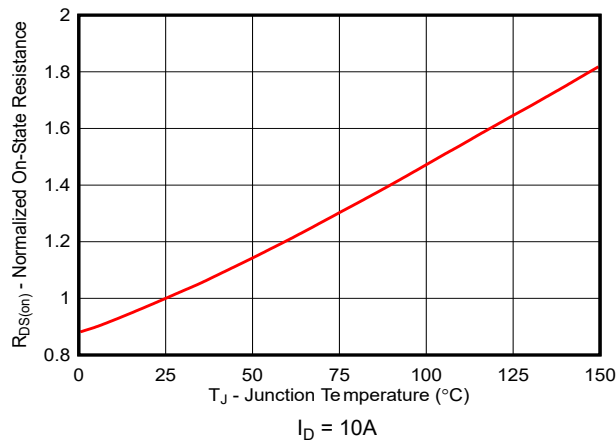
Figure 6-1. DRV7167 Normalized On-State Resistance vs Temperature
