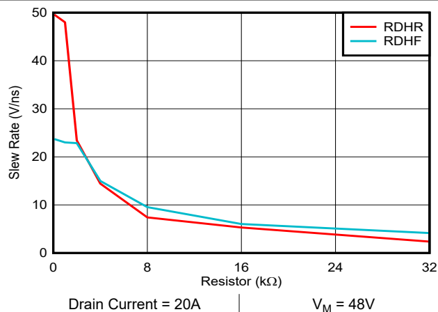
Figure 6-8. DRV7167: Slew Rate Control - Current leaving OUT pin
