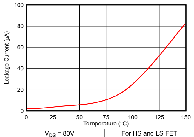
Figure 6-4. DRV7167: Drain Leakage Current
