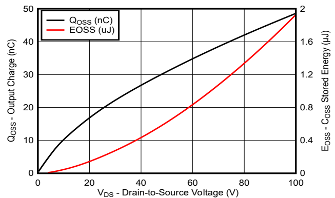
Figure 6-6. DRV7167 Typical Output Charge and Stored Energy
