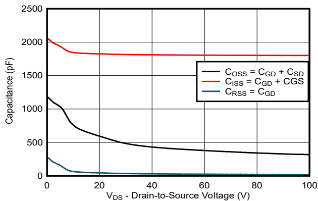
Figure 6-5. DRV7167: Typical Capacitance
