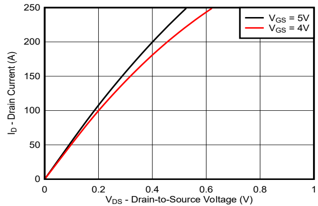
Figure 6-2. DRV7167 Typical Output Characteristics
