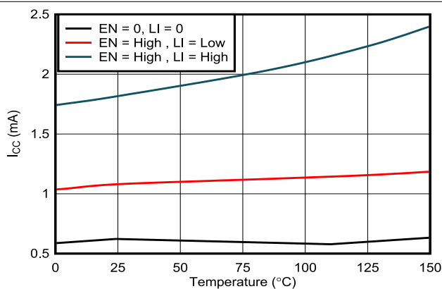
Figure 6-9. GVDD-AGND Current
