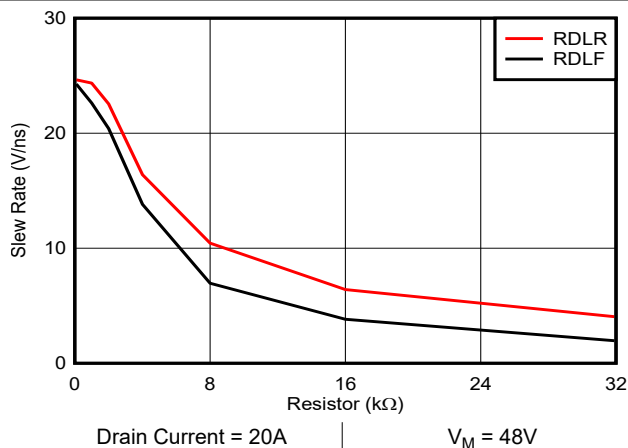
Figure 6-7. DRV7167: Slew Rate Control - Current entering into OUT pin
