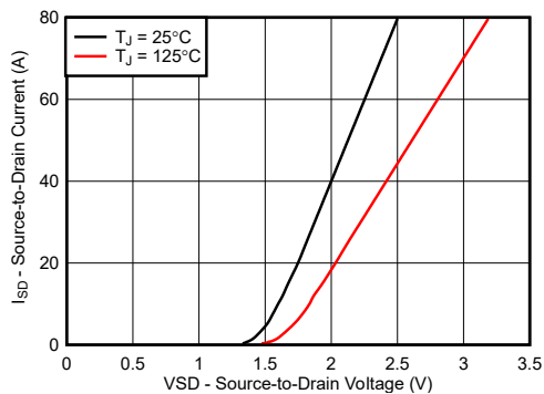
Figure 6-3. DRV7167 Reverse Drain-Source Characteristics
