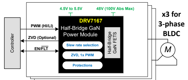
DRV7167 Simplified Schematic
