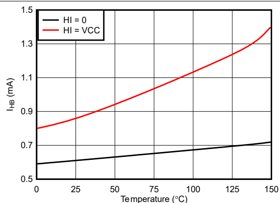
Figure 6-10. BOOT-HS Current
