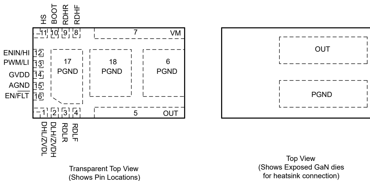
Figure 4-1. VBN Package, 18-Pin VQFN (Top View)
