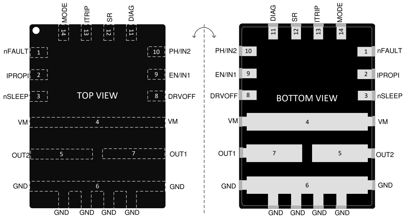
Figure 5-2. DRV8243H -Q1 HW variant in VQFN-HR (14) package
