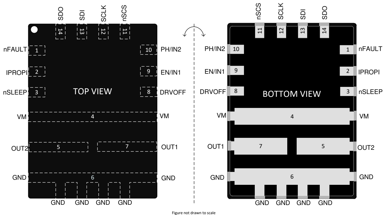
Figure 5-4. DRV8243S -Q1 SPI variant in VQFN-HR (14) package
