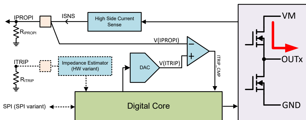
Figure 7-4. ITRIP Implementation
