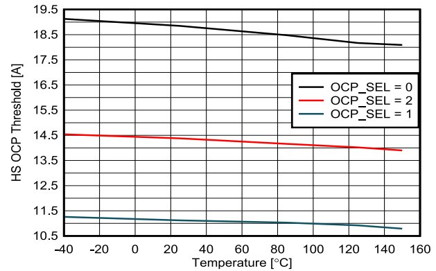
Figure 6-15. HS OCP Threshold vs Temperature at V_{VM} = 13.5\text{ V}
