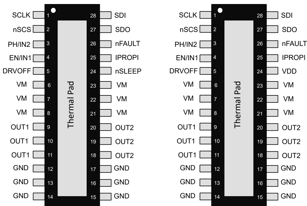
Figure 5-3. DRV8243S -Q1 SPI variant in HVSSOP (28) package
