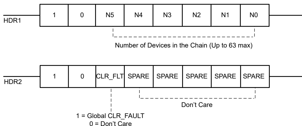
Figure 7-12. Header bytes
